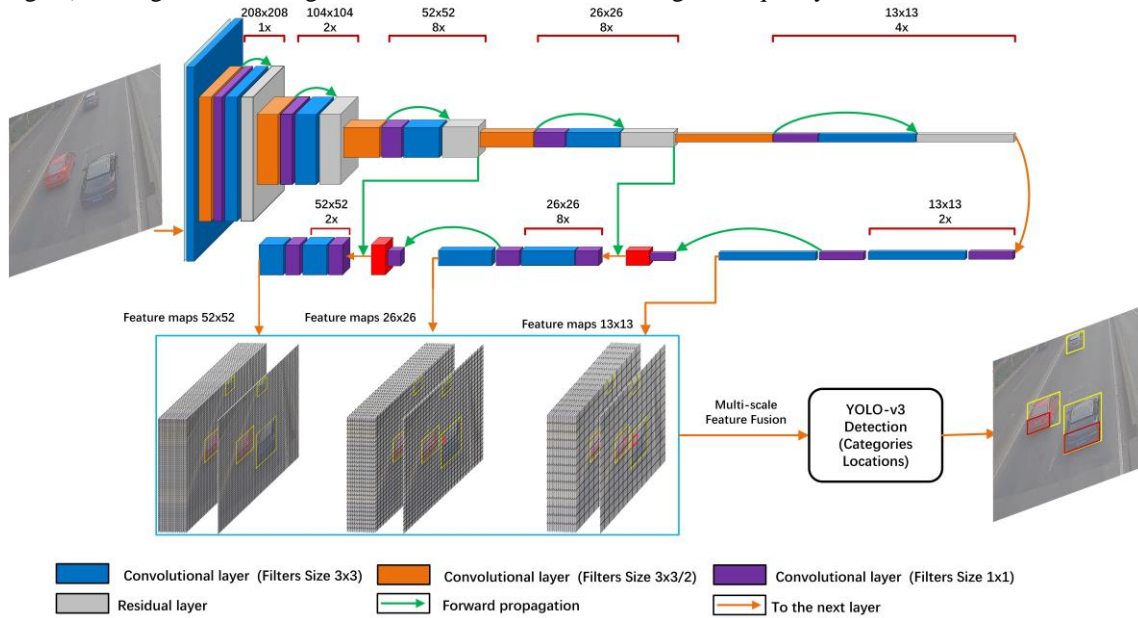
Fig. 8. Network structure of yolov3 overall and rear of vehicle dual target detection model
