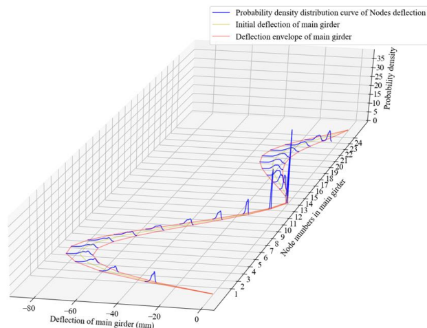
Fig.18. Spatial probability density distribution of deflection at bottom of main girder
