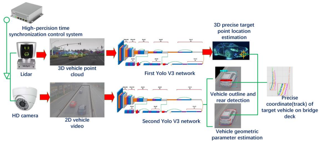
Fig. 9. Dual Yolo v3 network fusion target detection model of high-definition camera and lidar video signal
