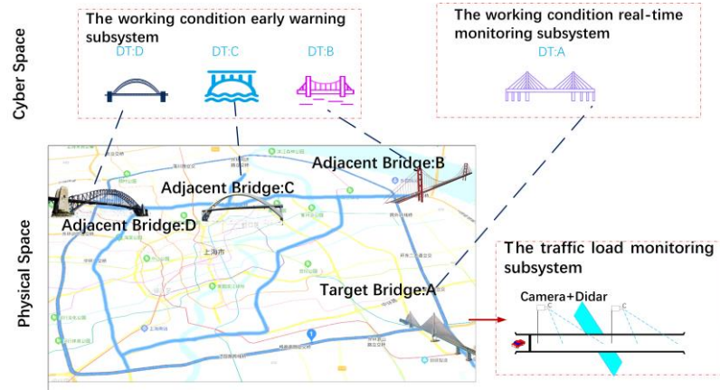
Fig. 2. Composition of bridge digital twin system of bridge network
