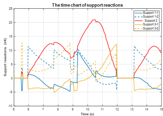
Fig. 15. Analysis results of support reactions of digital twin model for real-time overturning early warning analysis of box girder under measured traffic flow load
