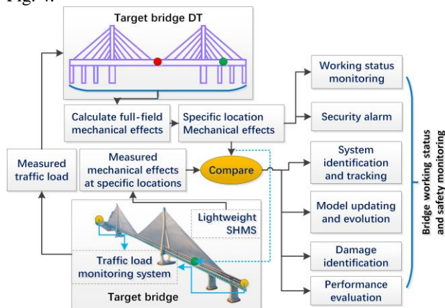
Fig. 4. Digital twin system on the target bridge
