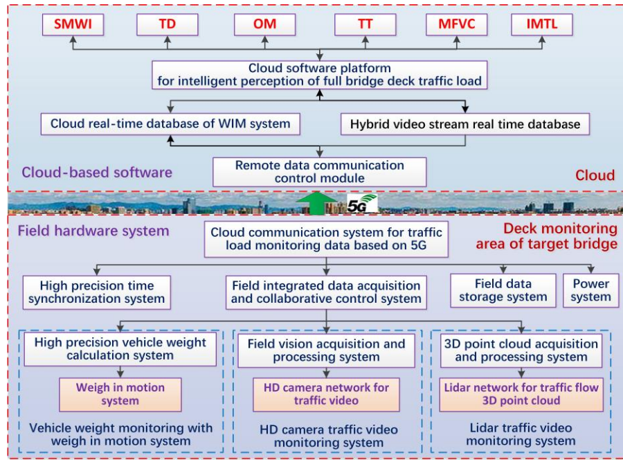
Fig. 6. Technical route of bridge traffic load spatio-temporal distribution perception system
