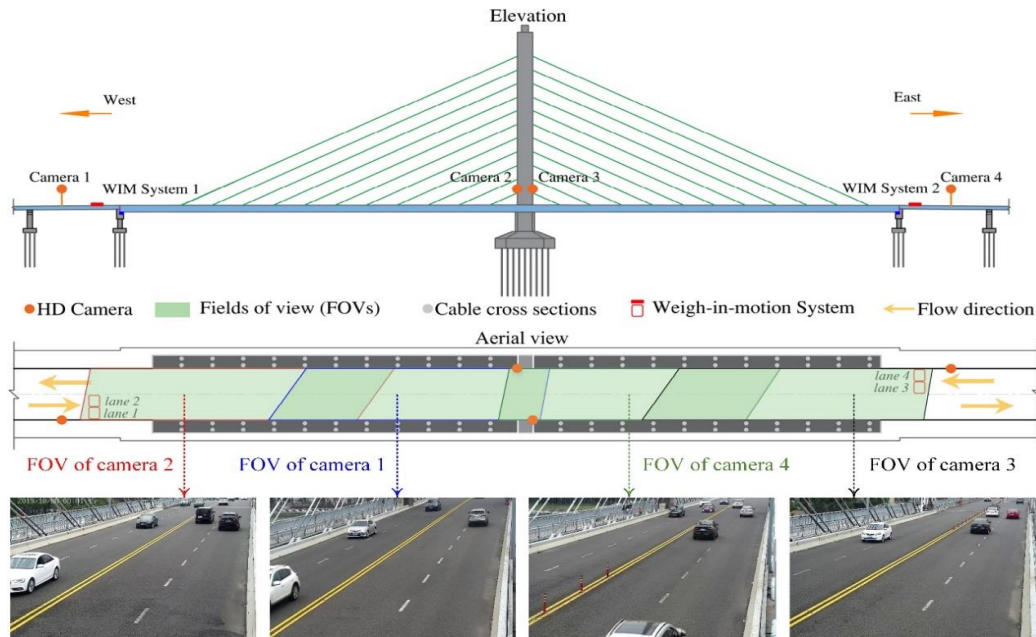
Fig. 11. Traffic flow load monitoring system of Yongjiang Bridge
