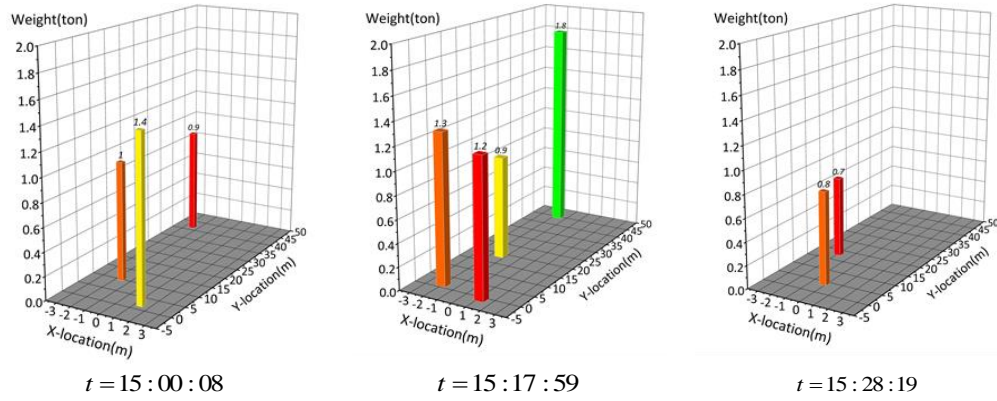
Fig. 12. Identification results of traffic load distribution of N4 ramp bridge on Tongji Road in Shanghai
