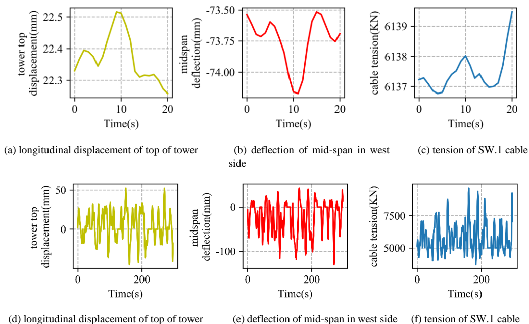
Fig. 16. Transient vehicle-induced response of cable-stayed bridge under different measured traffic load
