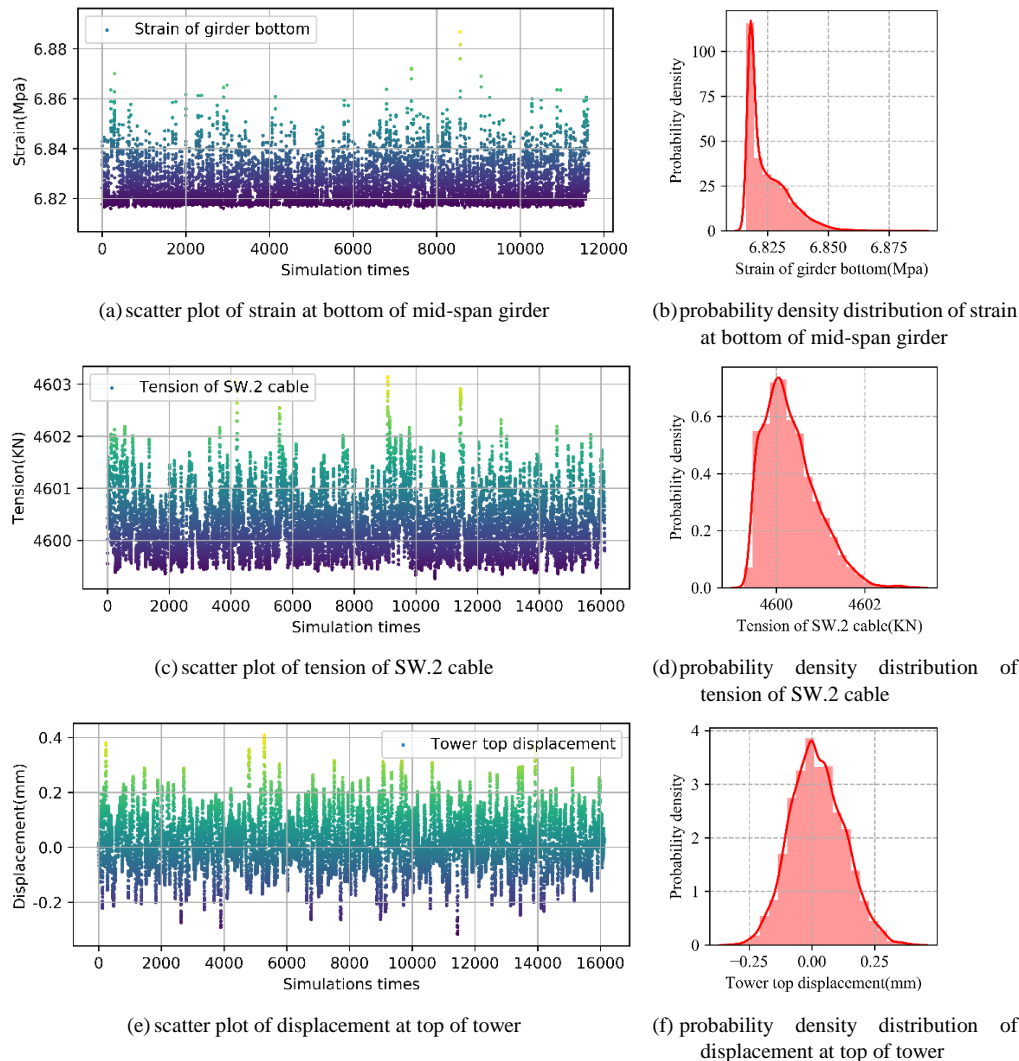
Fig.17. Simulation analysis of digital twin model of Yongjiang bridge under measured steady-state traffic load
