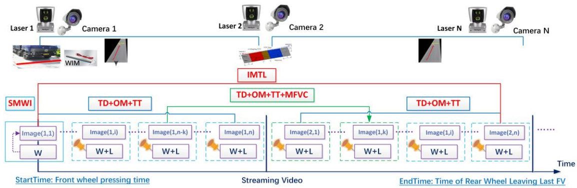
Fig. 7. Longitudinal distribution of each software module along bridge deck (Notes: W-Weight; L-Location)
