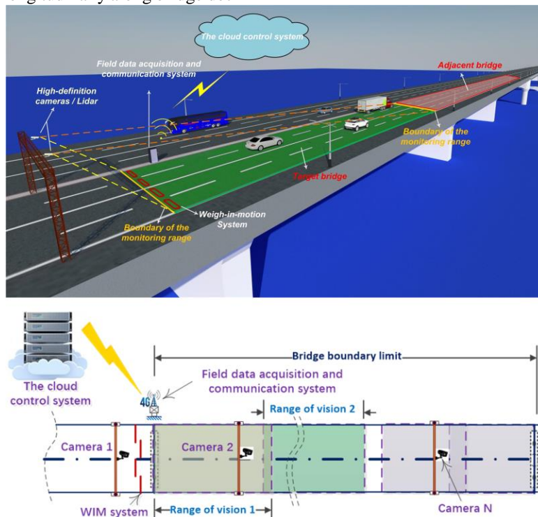
Fig. 3. Sensor layout of traffic load monitoring subsystem
