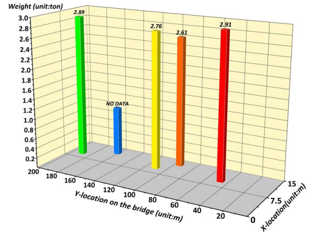
Fig. 13. Measured traffic flow load segment on full bridge deck of Yongjiang bridge (November 16, 2020)
