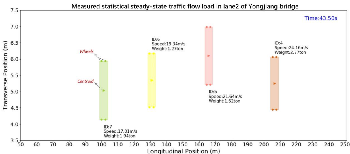
Fig. 14. Measured statistical steady-state traffic flow load on Yongjiang Bridge
