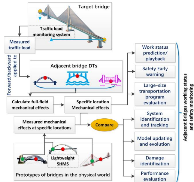
Fig. 5. Digital twin system on the adjacent bridges
