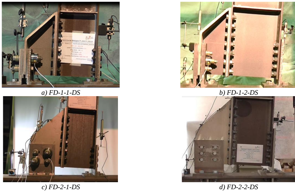
Figure 9 Deformed shape of the tested specimens at chord rotation equal to 0.05 rad
