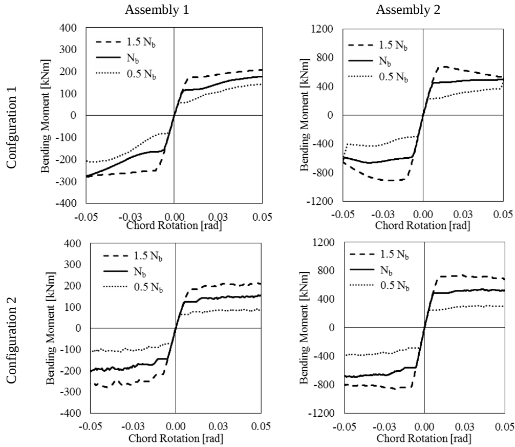
Figure 19 Influence of the clamping force on the bending moment capacity
