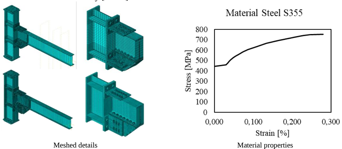
Figure 10. Features of FE model
