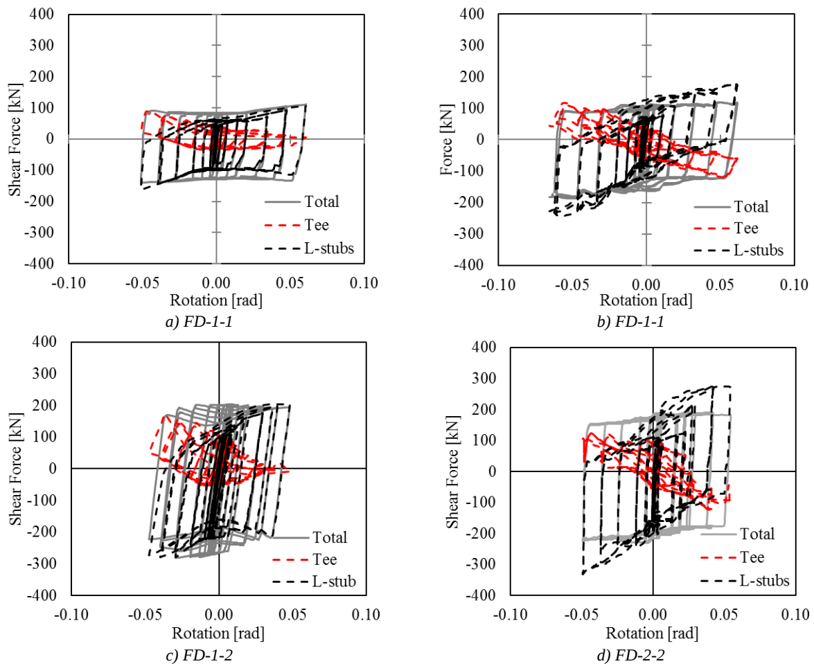
Figure 14 Shear force transferred by different components
