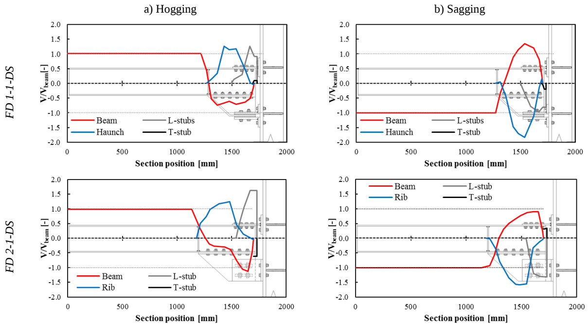
Figure 16 Distribution of shear in the connected elements at 0.04 rad damper rotation
