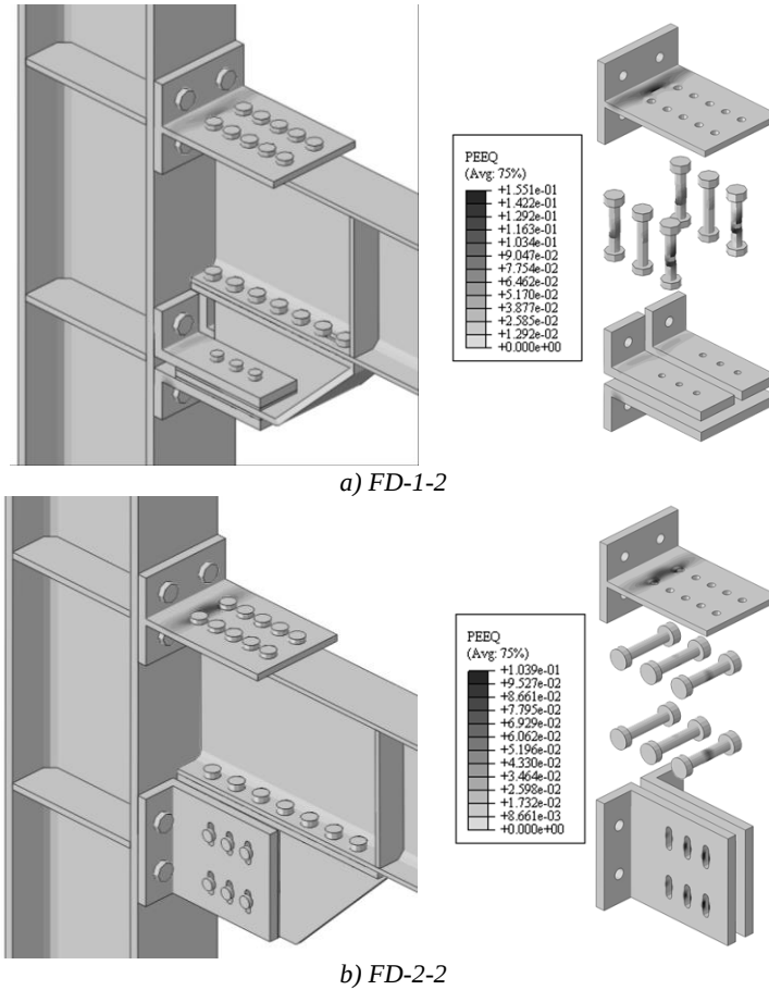
Figure 17 PEEQ Distribution at the end of the cyclic analysis for large joint assemblies
