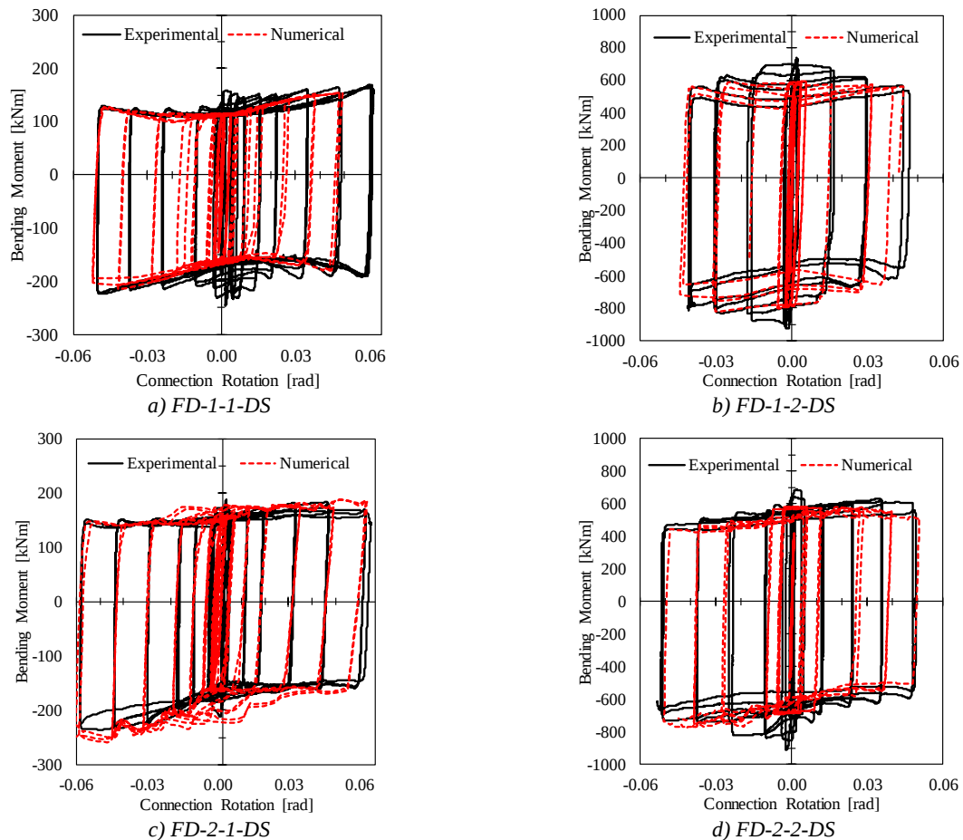
Figure 11 Experimental vs numerical results in terms of Bending Moment – Connection rotation
