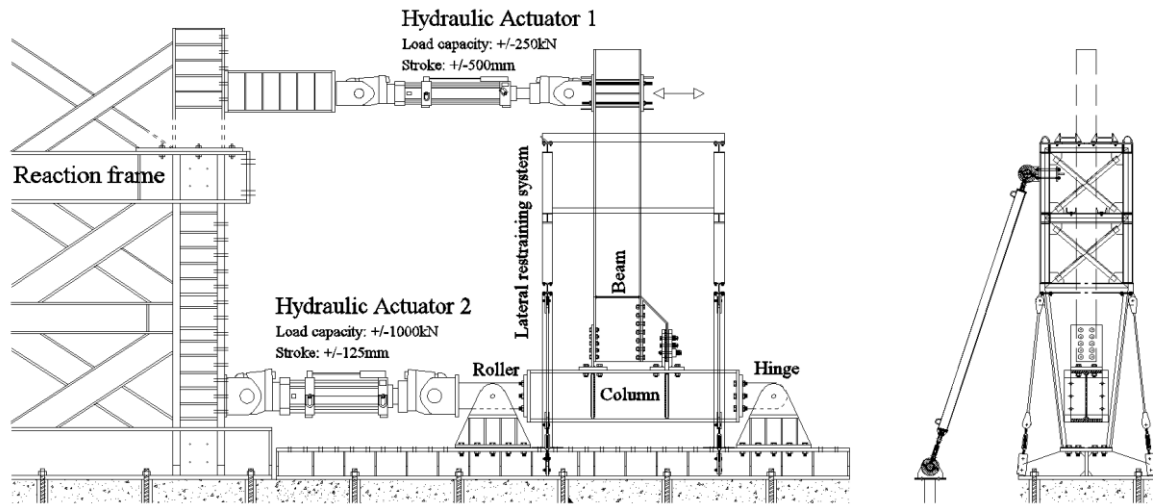
Figure 2 Experimental setup
