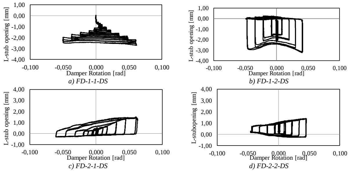
Figure 8 L-stub opening versus damper rotation
