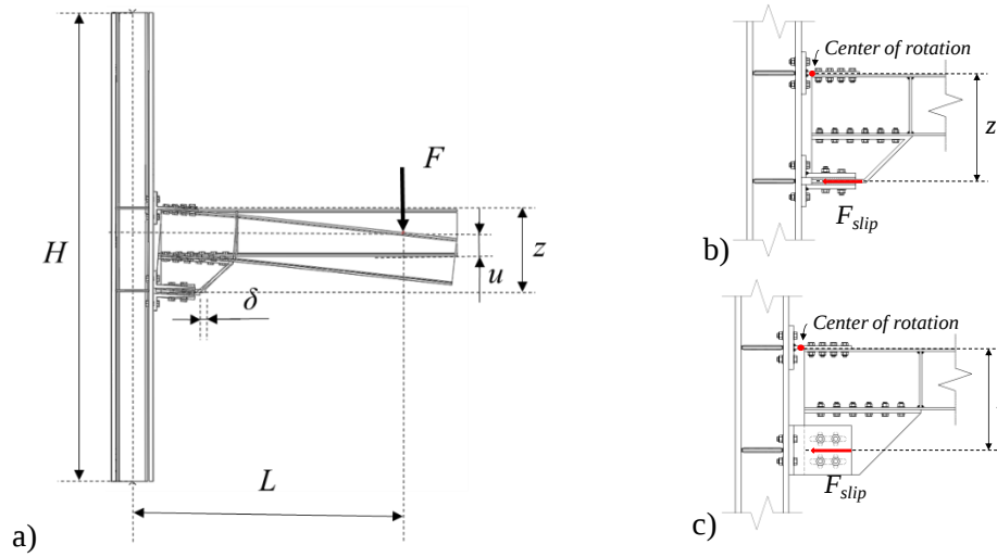
Figure 4 Monitored parameters: global (a) and local response (b,c)
