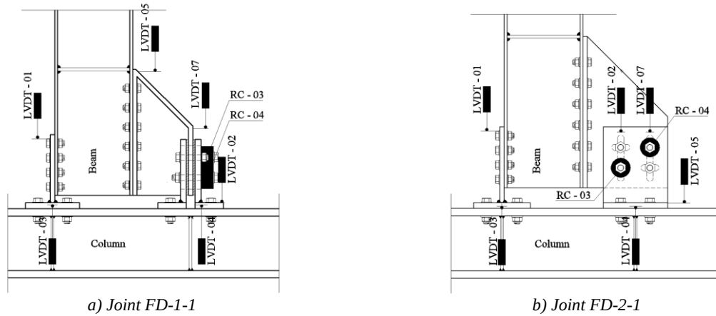
Figure 5 Layout of displacement transducers to measure the local response of joints
