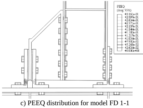
Figure 12 Experimental vs. numerical models after cyclic test up to 5%
