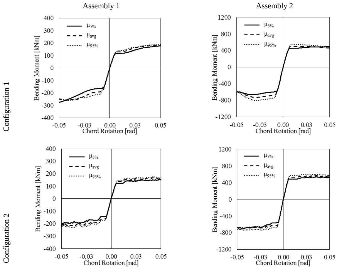
Figure 20 The influence of the friction coefficient on the bending moment resistance
