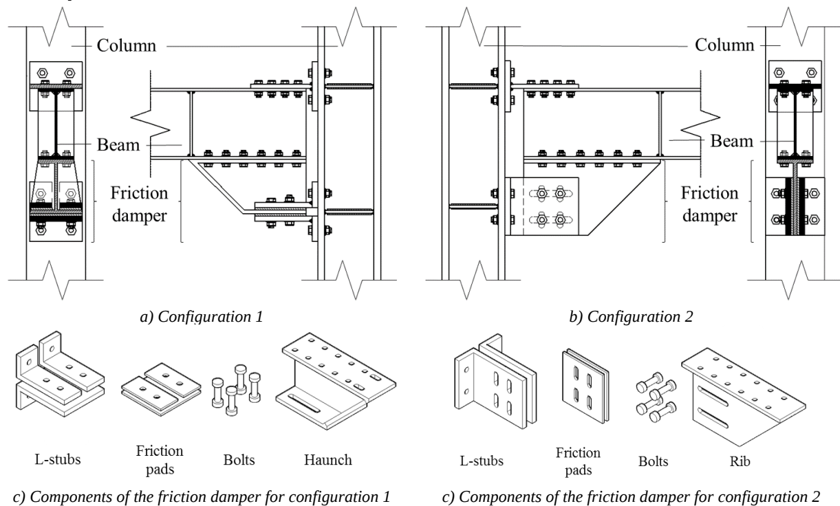
Figure 1 Typologies and features of the investigated joint configurations
