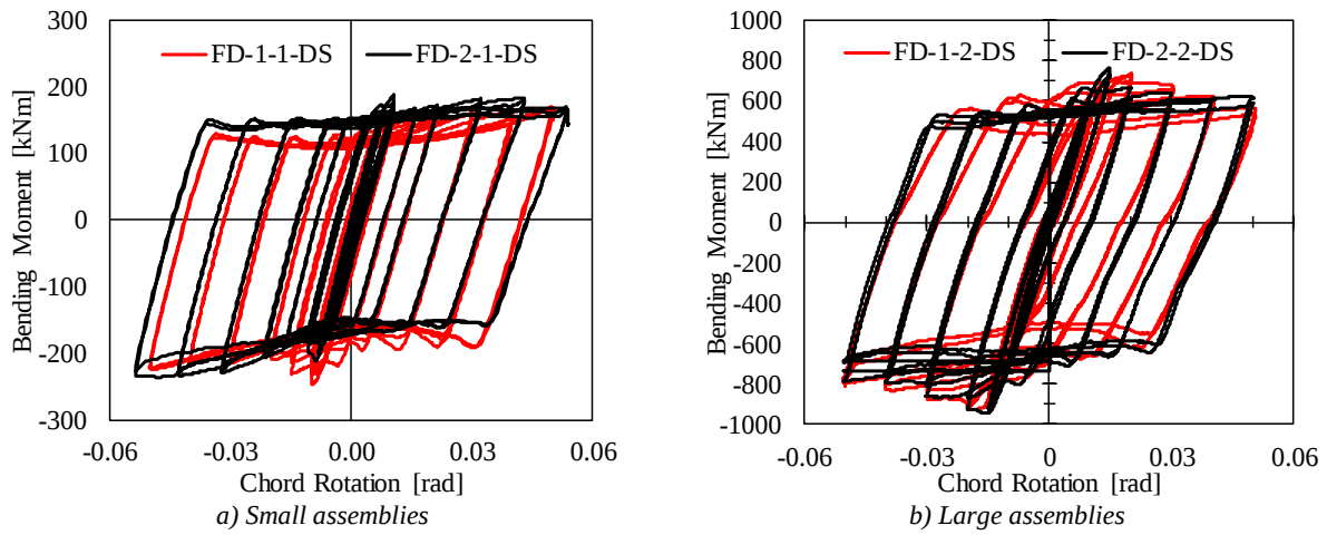
Figure 6 Comparison between the response of the 2 device configurations
