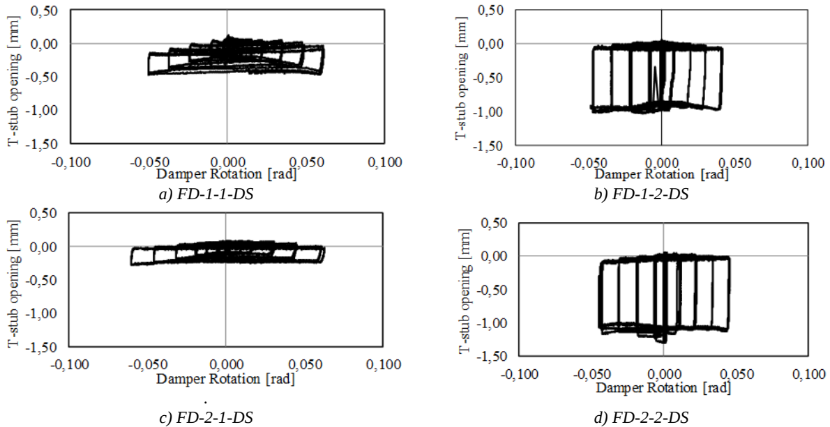
Figure 7 T-stub opening versus damper rotation
