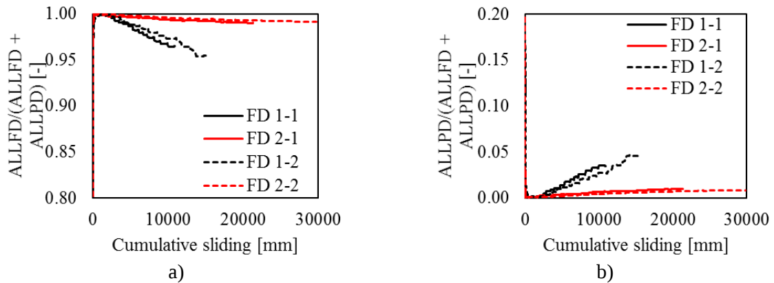
Figure 18 Normalised dissipated energy a) Friction energy and b) Plastic energy
