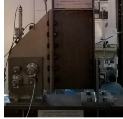
b) Experimental joint FD 2-1
