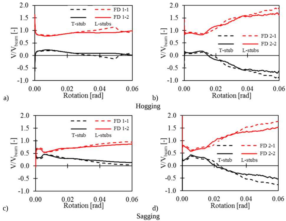
Figure 15 Shear force at the connection face
