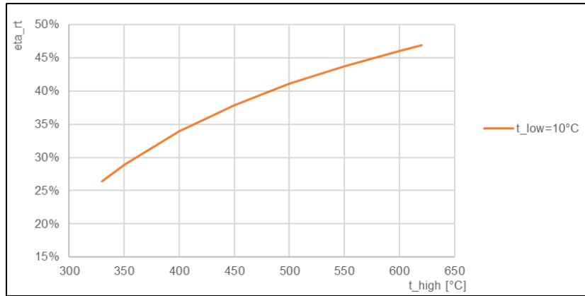
Figure 11: Effect of the high temperature on the systems round-trip efficiency (with a low temperature of 10 °C)
