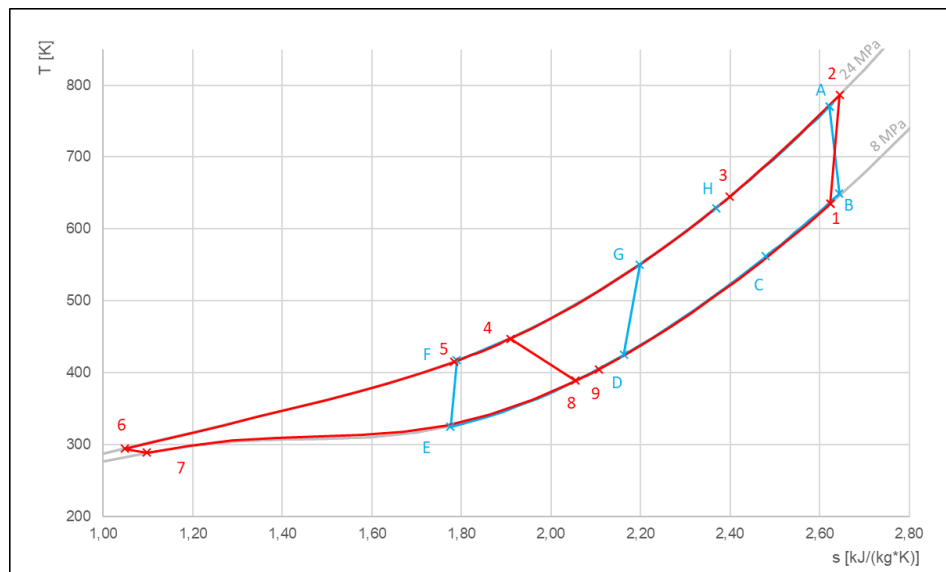
Figure 8: T-s diagram of the charging and discharging of the proposed PTES with recuperated and recompressed sCO 2 Brayton Cycle
