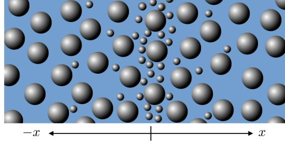
Figure 1: Schematic of a Gaussian pulse of hard-sphere tracer particles centred at x = 0 within a uniform suspension of larger host particles.
