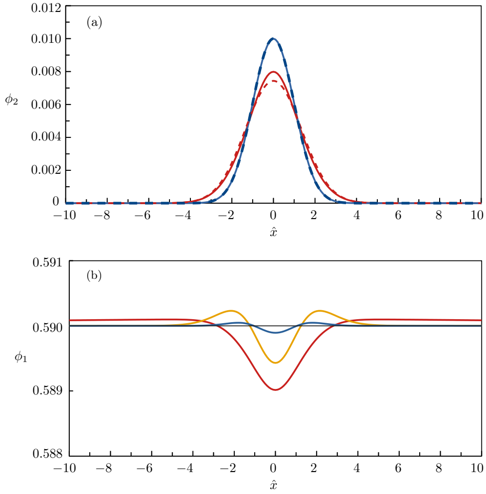
Figure 2: Plots of (a) tracer volume fraction \phi_2(\hat{x}) and (b) host matrix volume fraction \phi_1(\hat{x}) at times \hat{t} = 0.01 (blue), \hat{t} = 0.1 (orange) and \hat{t} = 100 (red) for the case \phi_1^0 = 0.55 , \phi_2^0 = 0.01 and \lambda = 0.75 . The dashed curves in (a) are the Gaussian \phi_2 profiles obtained in the absence of cross-diffusion.
