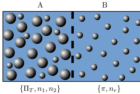
Figure 4: Illustration of osmotic equilibrium in a bidisperse hard-sphere suspension. The membrane separating compartments A and B is permeable to the fluid (blue) and smaller tracer particles but impermeable to the larger host particles. Because of excluded volume effects, the equilibrium tracer concentration n_2 in compartment A is less than the concentration n_r in the reservoir compartment B; \alpha = n_2/n_r is the equilibrium partition coefficient. \Pi_T is the total osmotic pressure of the mixture in A, while \pi is the osmotic pressure of the tracer suspension in B.
