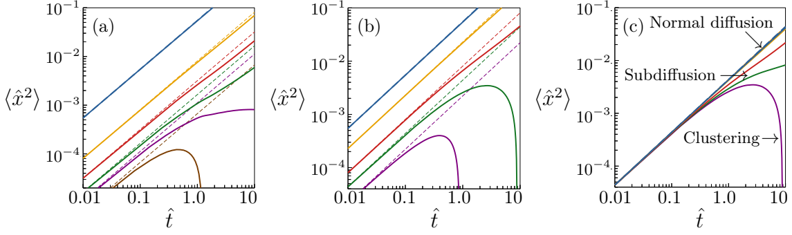
Figure 3: (a) Mean squared displacement \langle \hat{x}^2 \rangle computed from equation (16) for the case \phi_2^0 = 0.01 , \lambda = 0.75 and several initial host matrix volume fractions ( \phi_1^0 = 0.55 (blue); 0.59 (orange); 0.60 (red); 0.605 (green); 0.607 (purple); 0.61 (brown)). (b) Mean squared displacements for the case \phi_1^0 = 0.55 and \phi_2^0 = 0.01 and several particle size ratios ( \lambda = 0.75 (blue); 0.85 (orange); 0.95 (red); 1.0 (green); 1.05 (purple)). (c) Mean squared displacements for the case \phi_1^0 = 0.55 , \lambda = 1 and several tracer concentrations ( \phi_2^0 = 0.0005 (blue); 0.001 (orange); 0.005 (red); 0.008 (green); 0.01 (purple)). The dashed lines in (a)-(c) are the Gaussian MSDs \langle \hat{x}^2 \rangle = 2\hat{D}_{22}\hat{t} obtained in the absence of cross-diffusion effects.
