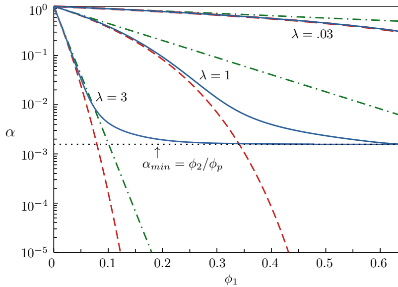
Figure 5: The equilibrium partition coefficient \alpha plotted versus \phi_1 for the case \phi_2 = .001 and several values of \lambda . The solid curves are from equation (40); the dashed curves are from Lekkerkerker's expression (31); the dot-dashed curves are from (30).
