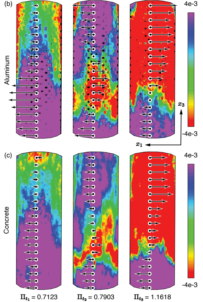
Fig. 5. Comparison of the experimental measurements of Fig. 4 in normalized \mu^N -scale. Shown are the dimensionless velocity and time \Pi groups \mu^N := \Pi_1 = v/\sqrt{\ell\mu g} , \Pi_t = t/\sqrt{\ell/\mu g} and dimensionless length corresponding to each of the Al/concrete systems compared for which \lambda_\ell = \ell^M/\ell^P = 0.23 and \lambda_\mu = \mu^M/\mu^P = 0.3 . (a) Comparison of the spine time records. (b) and (c) The normalized velocity fields for Al and concrete respectively shown for the same normalized times.
