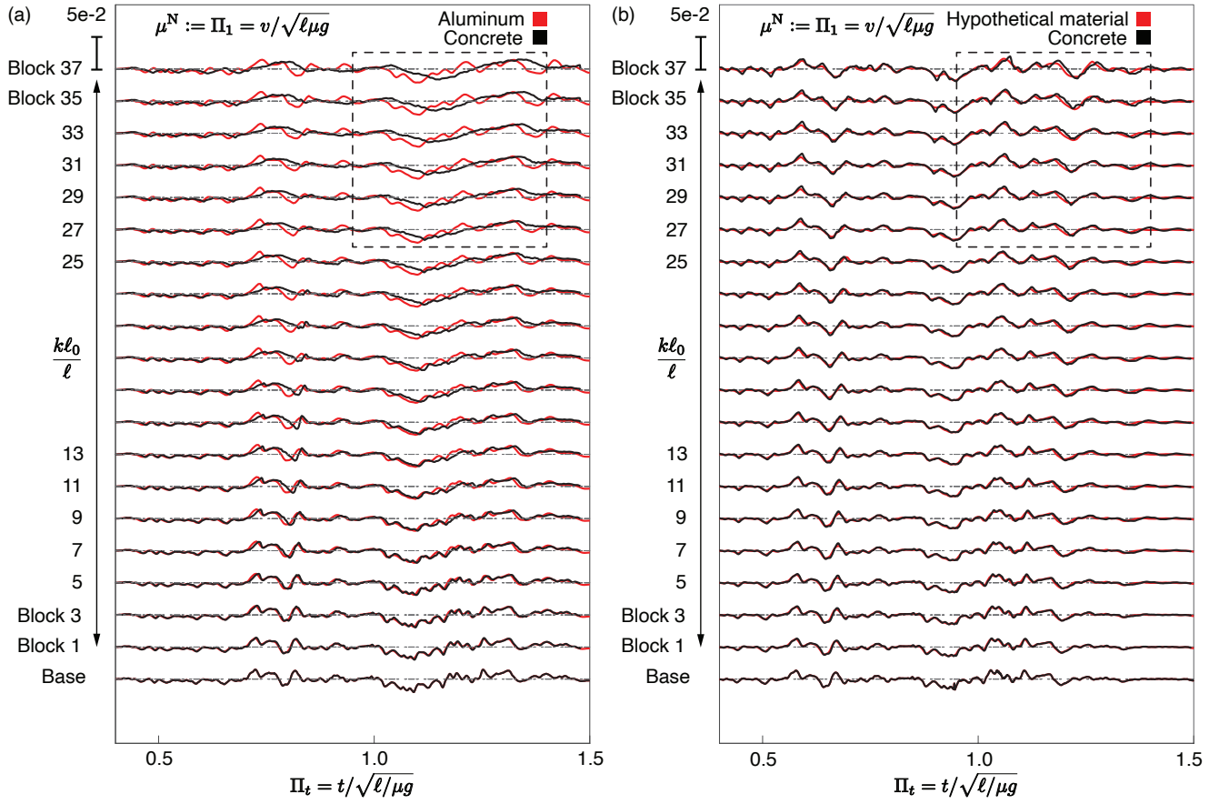
Fig. 6. Comparison of the results of LS-DEM simulations in normalized \mu^N -space. (a) An Al/concrete model/prototype pair ( \mu^M = 0.18 , \mu^P = 0.6 , \lambda_\mu = 0.3 , \lambda_\ell = 0.23 ) same as in the experimental comparison presented in Fig. 5. (b) A hypothetical material/concrete model/prototype pair ( \mu^M = 0.18 , \mu^P = 0.6 , \lambda_\mu = 0.3 , \lambda_\ell = 0.23 ) for which also c^M = c^P \sqrt{\lambda_\mu \lambda_\ell} ( c^M \sim 1,200 m/s, c^P \sim 4,600 m/s), satisfying the dimensionless requirement arriving from block elasticity.
