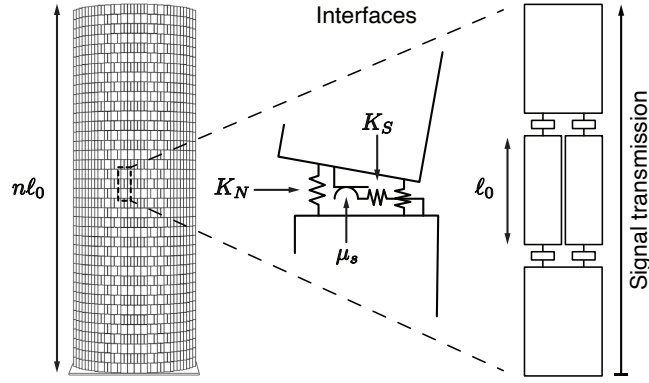
Fig. 7. The combination of elastic springs (normal and horizontal) and frictional element (horizontal) providing restoring forces between rigid blocks, as assumed in formulating the model for structural signal transmission. This model is consistent with LS-DEM methodology.
