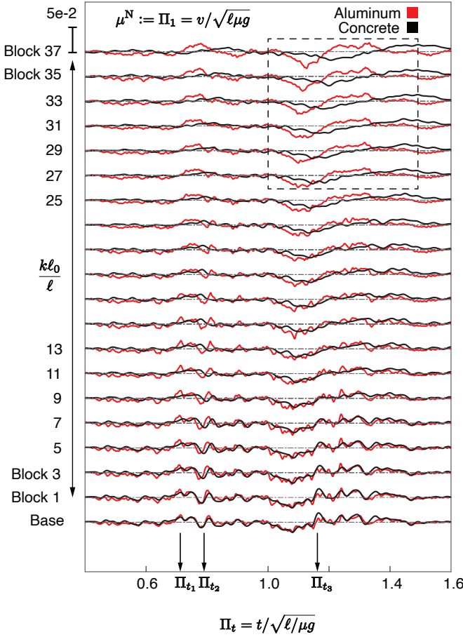
Fig. 5. Comparison of the experimental measurements of Fig. 4 in normalized \mu^N -scale. Shown are the dimensionless velocity and time \Pi groups \mu^N := \Pi_1 = v/\sqrt{\ell\mu g} , \Pi_t = t/\sqrt{\ell/\mu g} and dimensionless length corresponding to each of the Al/concrete systems compared for which \lambda_\ell = \ell^M/\ell^P = 0.23 and \lambda_\mu = \mu^M/\mu^P = 0.3 . (a) Comparison of the spine time records. (b) and (c) The normalized velocity fields for Al and concrete respectively shown for the same normalized times.
