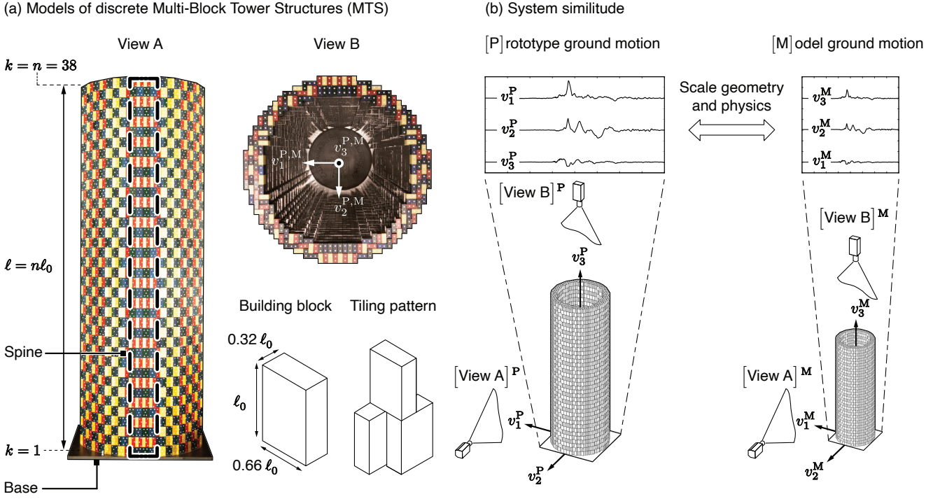
Fig. 2. An aluminum (Al) laboratory model (a) of a Multiblock Tower Structure (MTS) [1], or potential energy battery, used in large-capacity energy storage. Both model and prototype systems are composed of 7,144 blocks. The prototype tower may reach 160 m in height. The towers comprise 38 stories (188 blocks each) and is constructed during periods of peak energy harvesting by following a repeated tiling pattern of the type shown. The potential energy stored is recovered during periods of peak energy demand by deconstructing the tower. (b) Exploring the seismic response of such a discontinuous structure by using geometrically similar, scaled-down models in the laboratory necessitates the appropriate scaling of the ground velocity (or acceleration) time-histories both in amplitude and time as shown in (b). The identification of dimensionless numbers describing the physics of this dynamic problem informs the scaling and results in model/prototype similitude. The optical diagnostics are also scaled.
