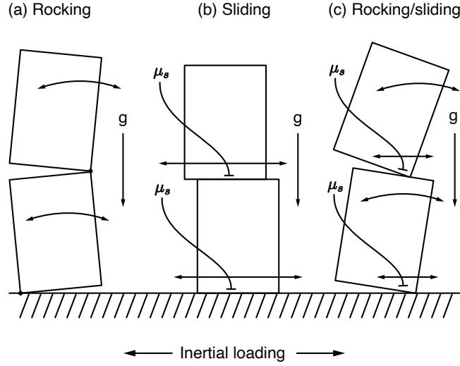
Fig. 3. Basic kinematics of rocking, frictional sliding and frictional rock/sliding of individual blocks within a multiblock structure.
