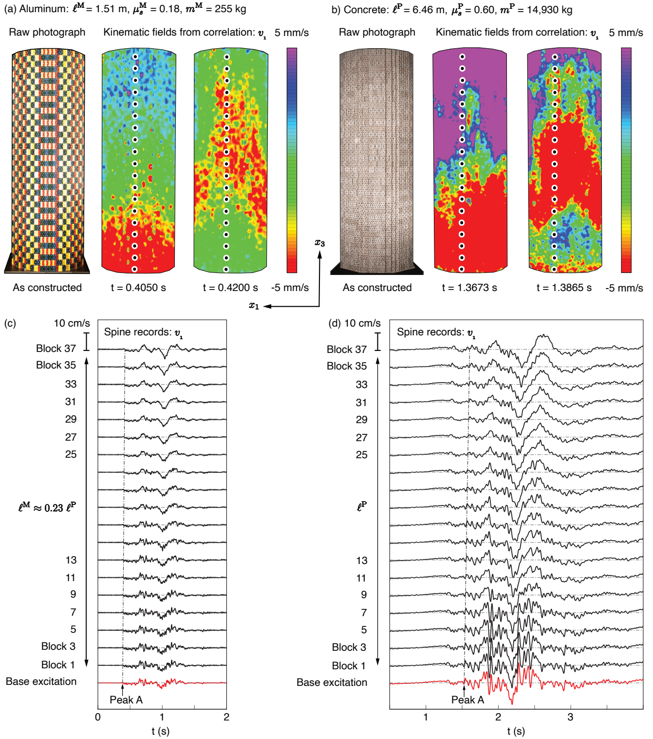
Fig. 4. High-speed optical measurements of the horizontal velocity component v_1 (color plots), enabled by Digital Image Correlation (DIC) for (a) an aluminum (Al) and (b) concrete model/prototype tower pair. (c) and (d) show velocity time histories of the imposed, scaled base excitations (red) and the resulting velocities (black) of individual blocks situated at 19 points (circles) up the heights of the 38 story towers. These histories are called the “spine records”.
