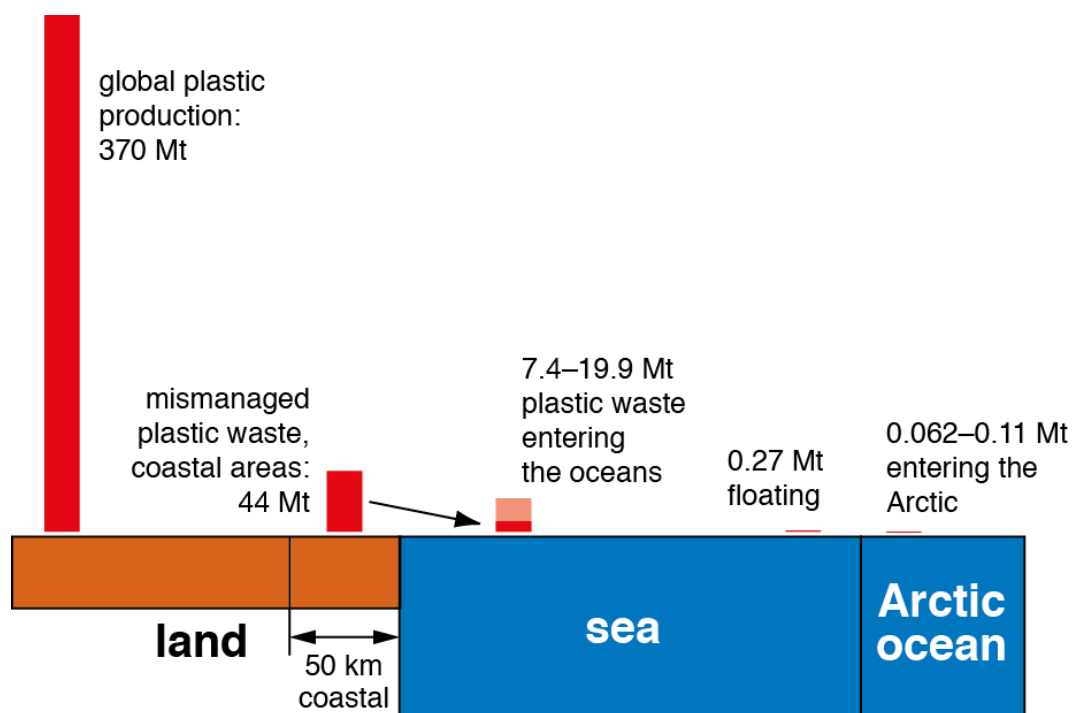
Figure 1: Plastic waste entering the oceans in 2019. Breakdown of data similar to the scheme by Jambeck et al. ( https://jambeck.engr.uga.edu/landplasticinput ). Data for 2019 obtained by scaling the data for 2010 (Jambeck et al. 2015) by the ratio of the global plastic production in 2019 and 2010 (370 Mt divided by 270 Mt equal to 1.37). Global plastic production for 2019 from Plastics Europe (2020). Amount of plastic floating on the surface of the oceans from Eriksen et al. (2014), van Sebille et al. (2015); amount of plastic entering the Arctic from Zarfl and Matthies (2010); see below, section on Mass balance of chemicals additives that can reach remote regions. Mt: million metric tons.
