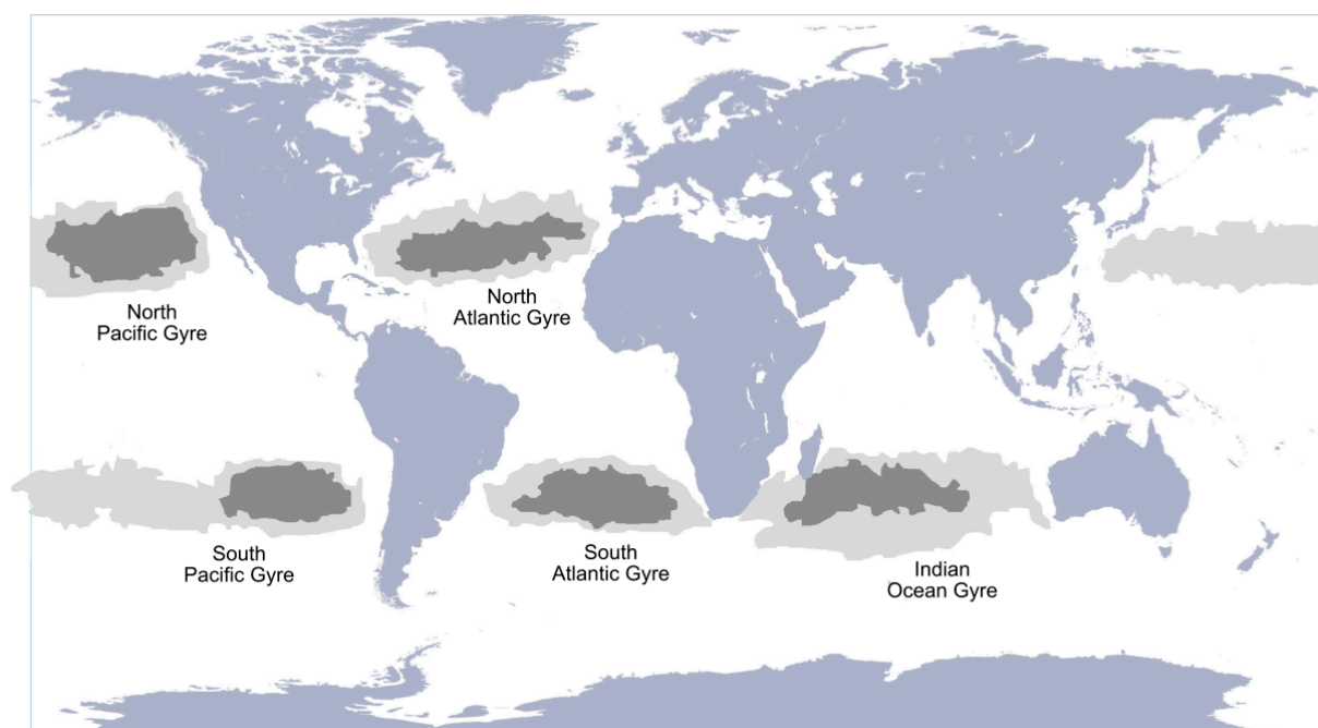
Figure 2: Location of the five major plastic gyres. Dark and light grey represent inner and outer accumulation zones, respectively; white areas are predicted as non-accumulation zones. The locations of the accumulation zones taken from C3zar et al. (2014); map created by the authors.
