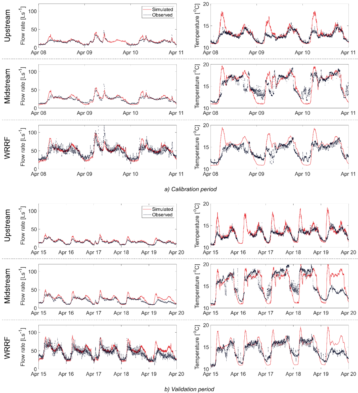
Figure 4: Calibration and validation of flows and temperatures at three locations (upstream, midstream, and at the WRRF) in the sewer network. a) Calibration period (Monday, April 8 to Wednesday, April 10, 2019). b) Validation period (Monday, April 15 to Friday, April 19, 2019). Note that the 19 th of April is a public holiday.
