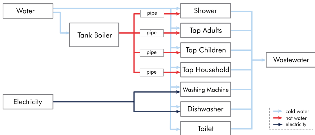
Figure 2. Reference household system modelled with the WaterHub modelling framework (Hadengue et al, 2020).
