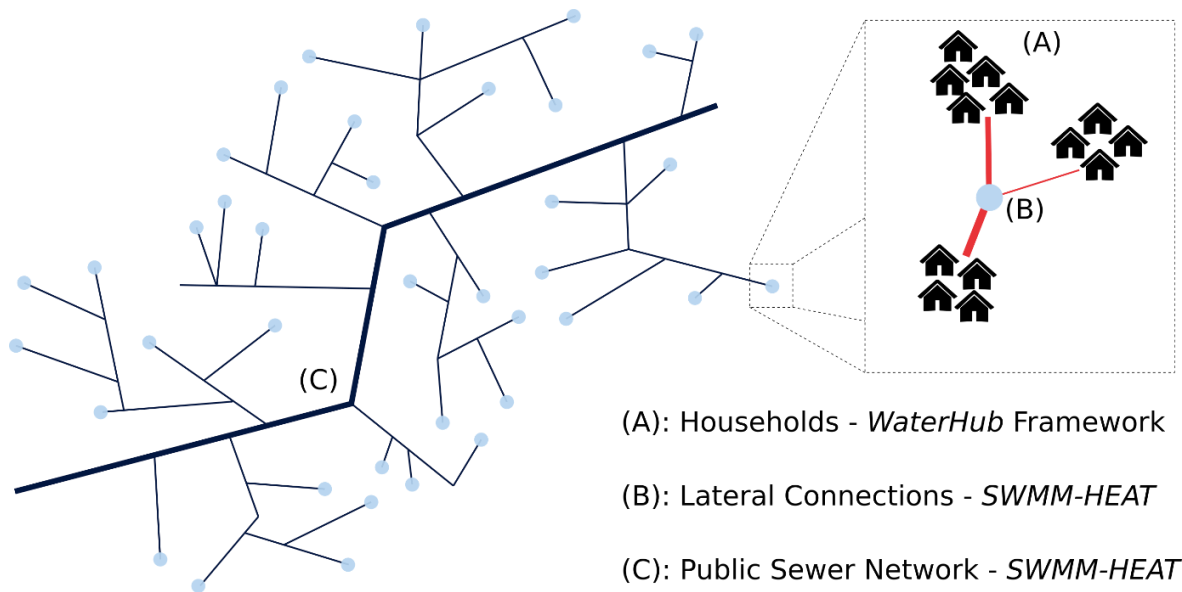
Figure 1. Schematic of the modelling framework, including three sub-models (A), (B) and (C) to simulate thermal-hydraulic dynamics of wastewater from the source (household) to the sink (WRRF).
