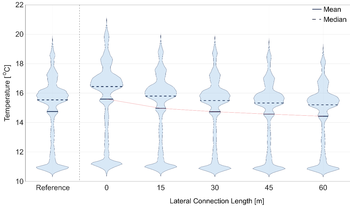
Figure 5. Temperature distributions at the WRRF Fehraltorf for increasing lateral connection lengths (sub-model B). The reference case – the validated model from Section 3.1 – includes randomized lateral connection lengths (very left distribution). The red line represents the trend of the mean distribution values.
