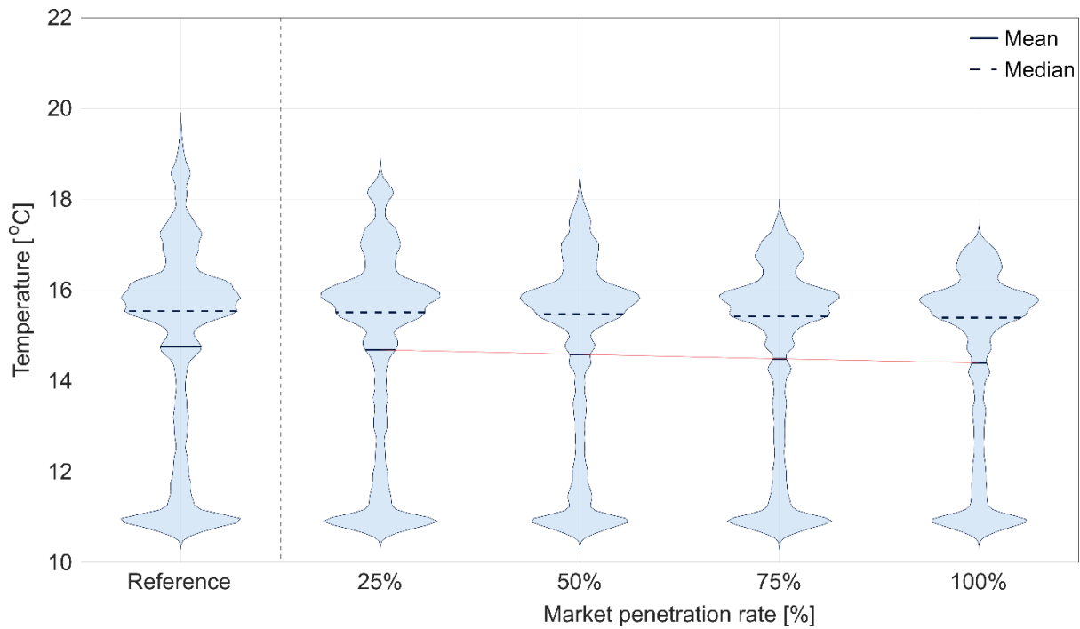
Figure 6. Temperature distributions at the WRRF Fehrltorf for various in-building heat recovery scenarios. The reference case – the validated model from Section 3.1 – is compared to increasing market penetration levels (25% to 100% penetration) of a shower drain heat recovery device. The red line represents the trend of the mean distribution values.
