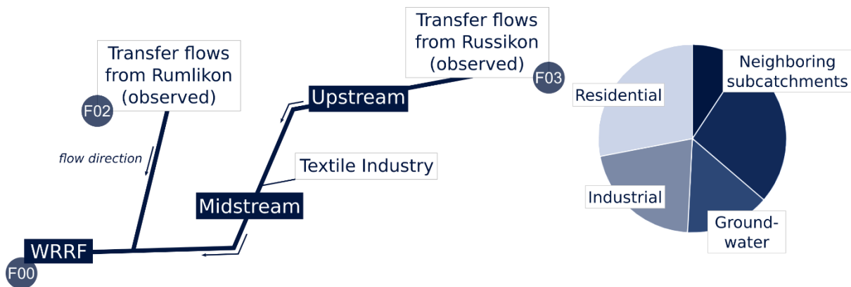
Figure 3. Schematic description of the Fehraltorf catchment with the three monitoring locations upstream, midstream and at the WRRF used for the calibration and validation process (see Section 2.2). We show transfer flows from the neighbouring sub-catchments Rumlikon and Russikon, as well as the main textile industry. The relative wastewater flow shares at the WRRF are shown on the right. F00, F02 and F03 designate the flow monitoring stations necessary to determine the groundwater infiltration rates.
