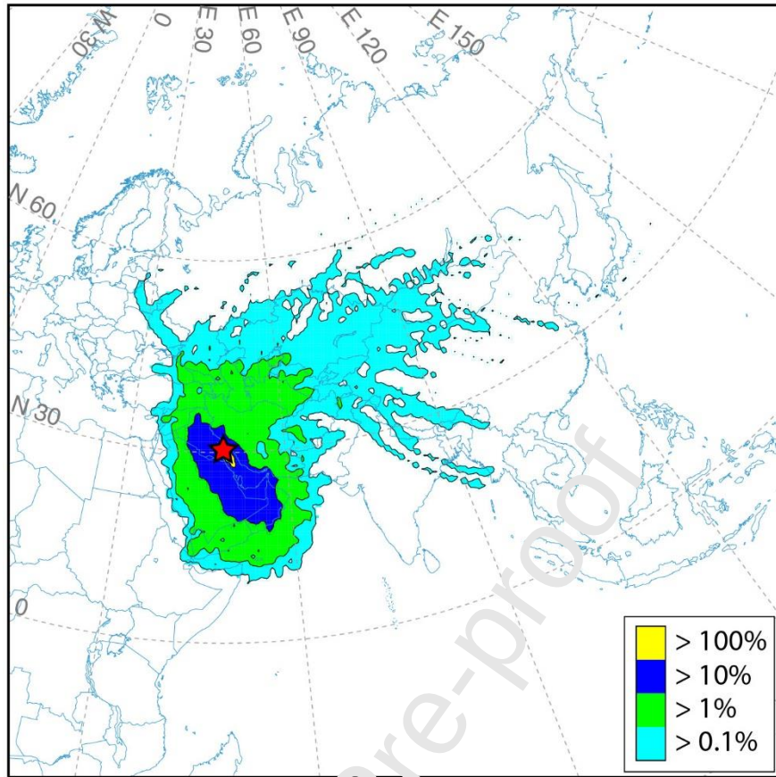
Figure 7. Forward trajectory frequency map for Shalamchah ( 30^{\circ}45' N and 48^{\circ} 15'E ) using HYSPLIT-4 during the cold periods of the years between 2007 and 2018.
