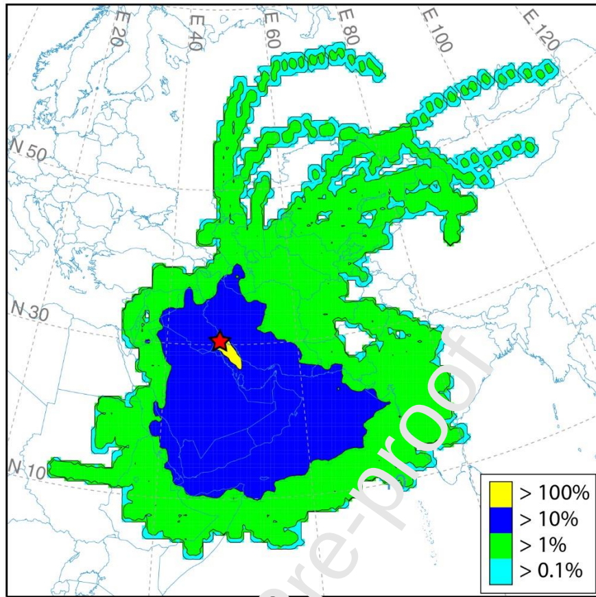
Figure 6. Forward trajectory frequency map for Shalamchek (30°45' N and 48° 15'E) using HYSPLIT-4 during the warm periods of the years between 2007 and 2018.
