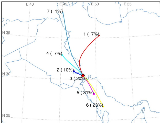
b) Trajectory cluster groups for cold period
