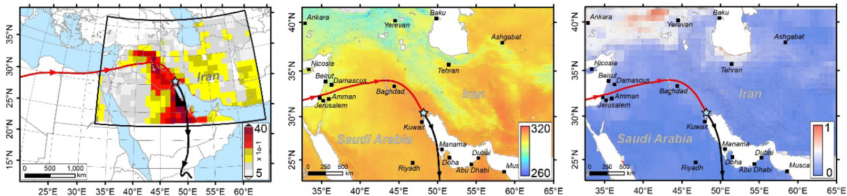
a) SDS event on 17/04/2010
