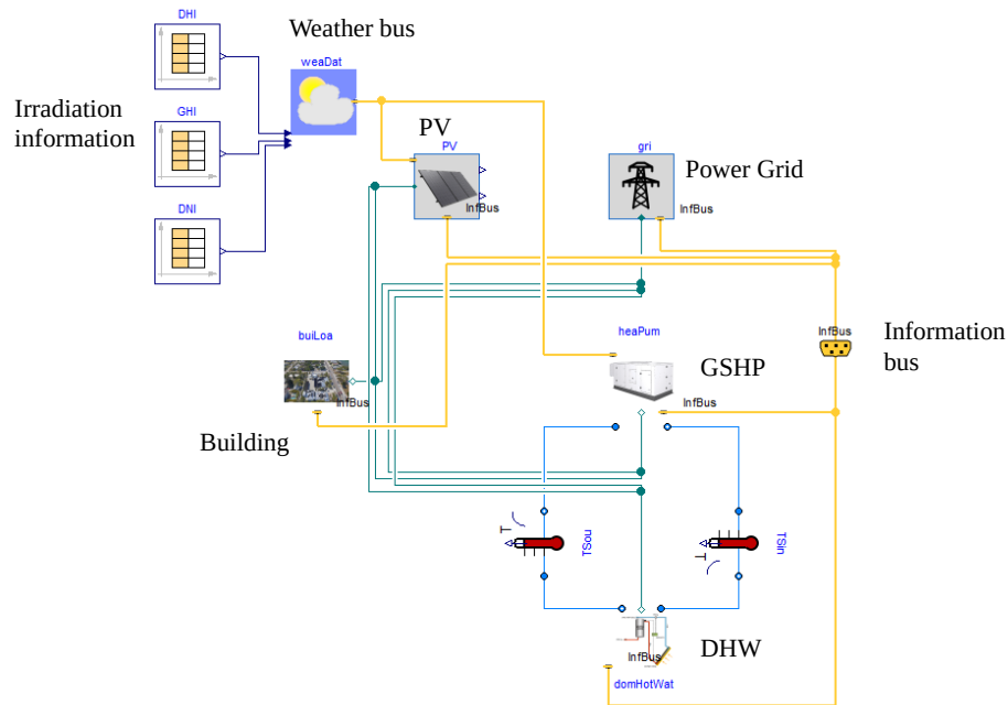
Figure 6. Diagram of top-level models for the HGV.
