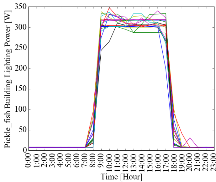
Figure 9. Electricity load profiles of lighting equipment in a retail building (each line represents one day of data).
