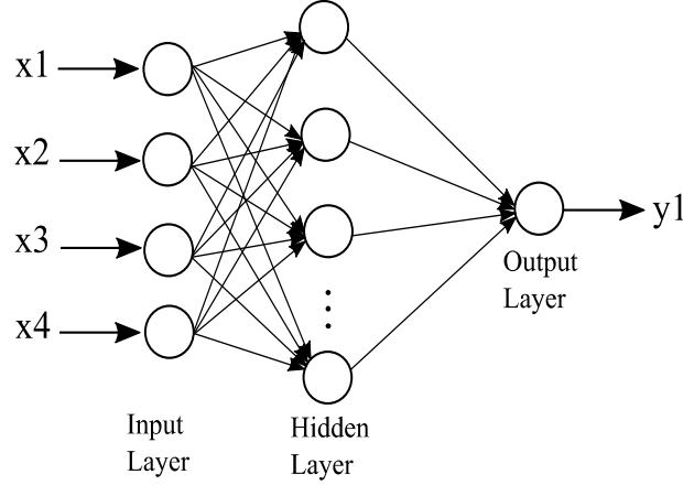
Figure 8. The structure of the neural network model.
