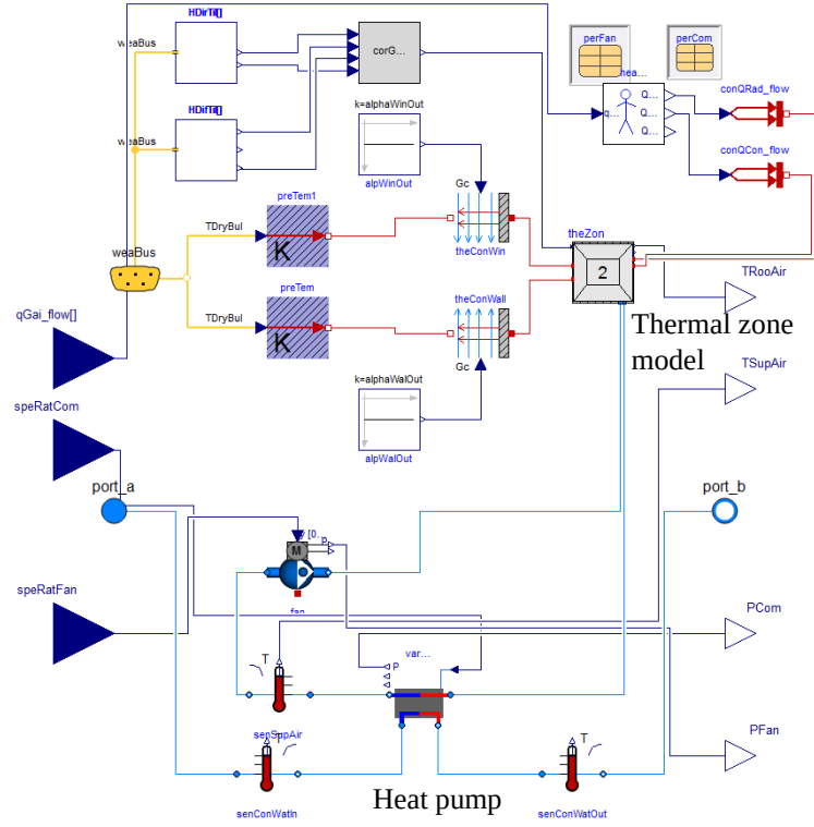
Figure 12. Diagram of Modelica models for the GSHP module.
