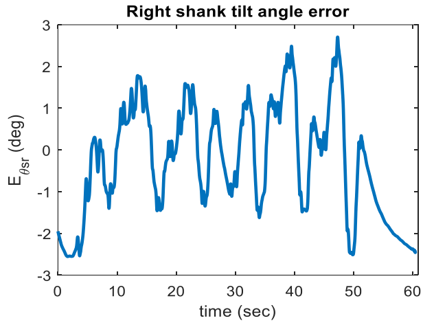
Fig. 14. Right leg tilt angle error of nonlinear observer compared to the IR camera measurement.
