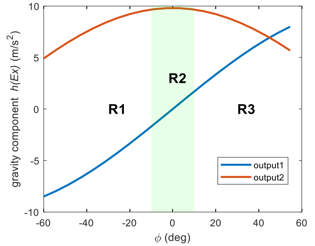
Fig. 3. Assumed constant-gain regions of the observer. In regions R1 and R3 both outputs are used but in region R2 only the first output is used.
