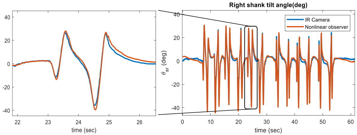
Fig. 9. Right shank tilt angle from IR camera and nonlinear observer.
