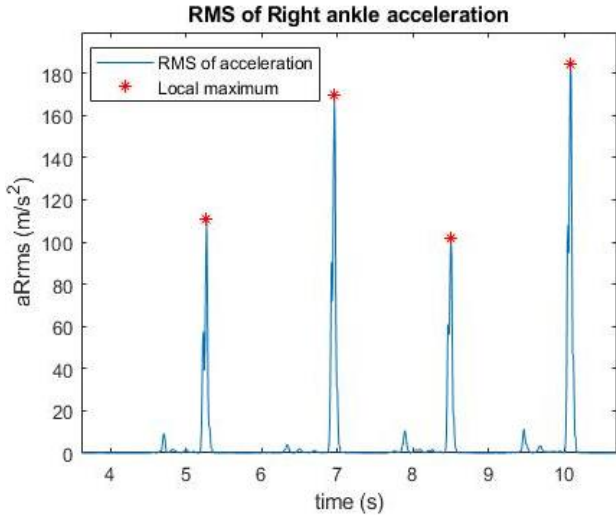
Fig. 4. An example of the RMS signal of the right shank acceleration and its local maximums that are used to identify the heel-strikes of each step
