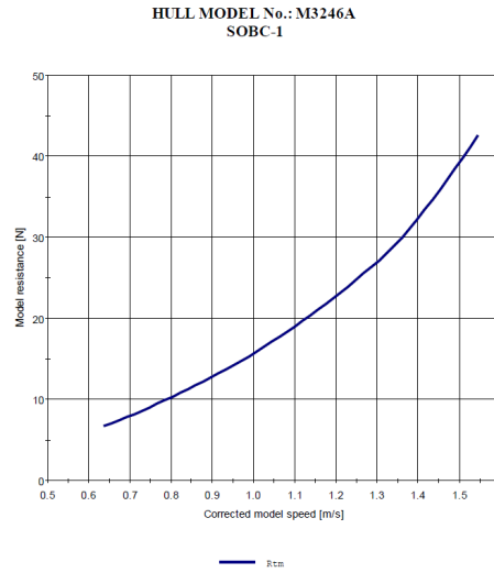
Figure B.15: Resistance test results
