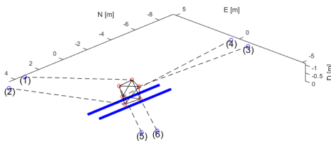
Figure 8: Placement of the actuators and attachment points. The Figure has a similar orientation as Figure 6. Actuator numbering in parentheses. The blue thick lines represent the sides of the ship’s deck. Coordinates are at model scale.
