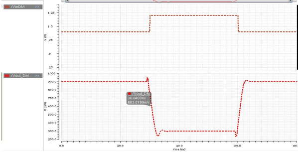
Fig. 20: Large input step = 300 mV
