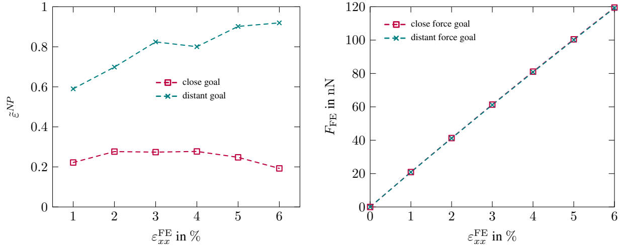
Figure 9: Components of the objective function used by the optimizer to determine mechanical property profiles inside the interphases: Normalized interparticle strain histories \tilde{\epsilon}^{NP} (left) for the close and distant cases and corresponding overall reaction force curves (right).
