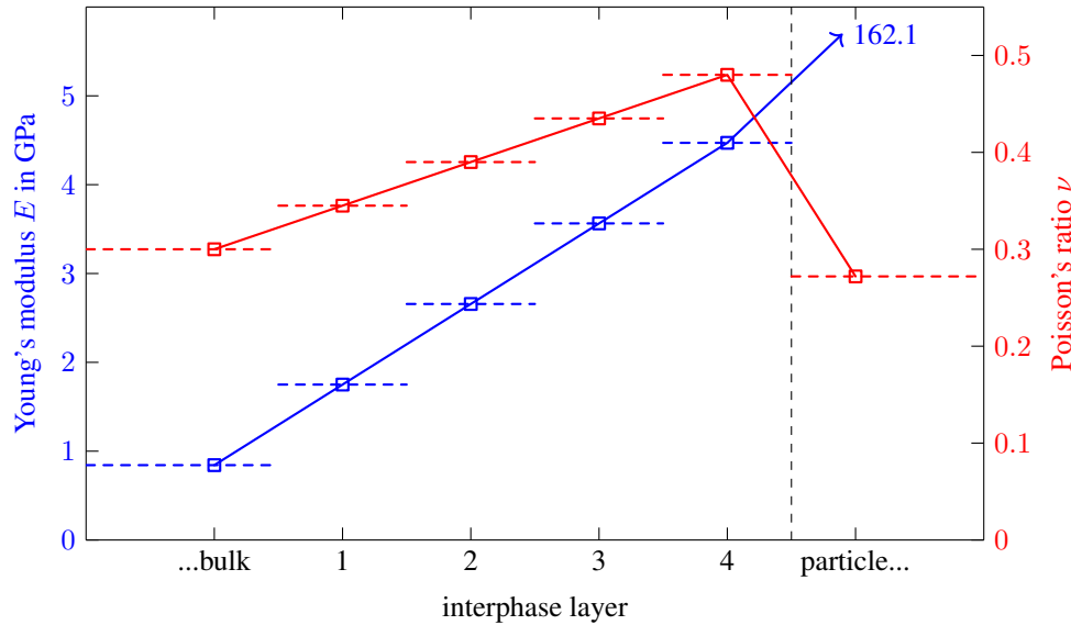
Figure 11: Optimal linear profiles for the elasticity parameters inside the interphases.
