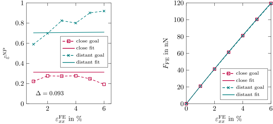
Figure 12: FE simulation results vs. Capriccio data for the close and distant cases with optimized linear profiles of the elasticity parameters inside the interphases: Profiles of normalized interparticle strain (left) and overall force (right).
