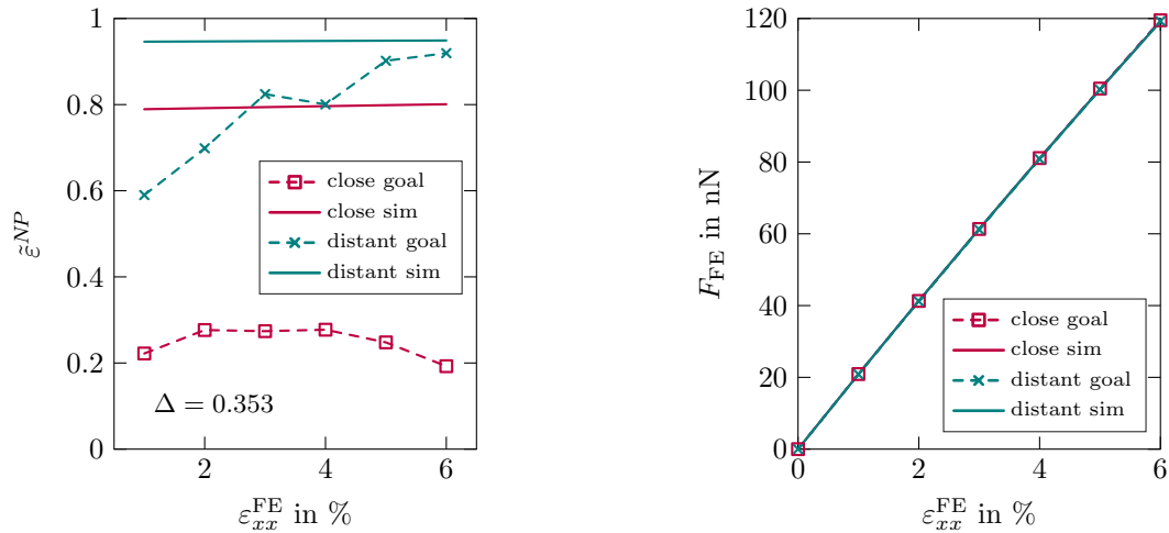
Figure 10: FE simulation results vs. Capriccio data for the close and distant cases, assuming homogeneous elastic material without interphases: Profiles of normalized interparticle strain (left) and overall force (right).
