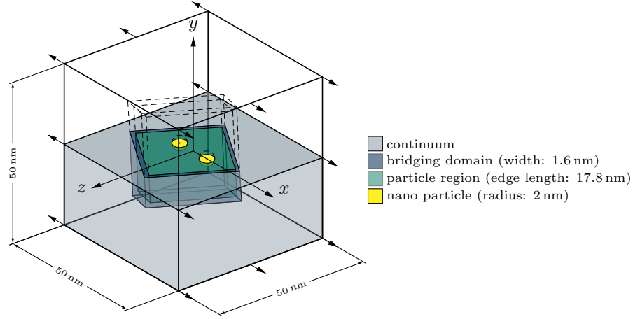
Figure 4: MD-FE simulation setup: A particle region comprising two nanoparticles and a polystyrene matrix, as well as its surrounding bridging domain are integrated into a continuum cuboid in such a way that the nanoparticles are aligned on the x -axis and their center coincides with the coordinate origin.
