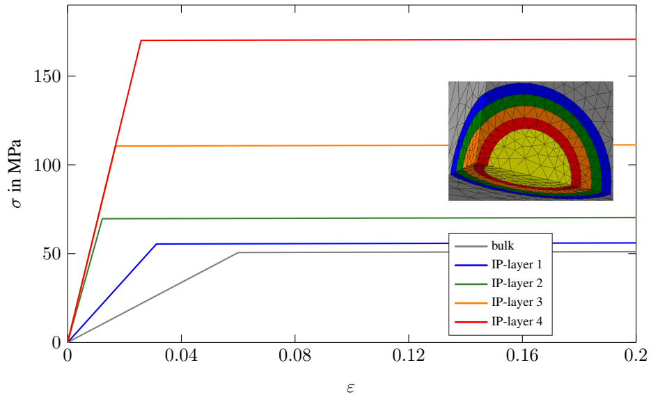
Figure 21: One-dimensional stress-strain curves for elastoplastic material with exponentially saturating profiles.
