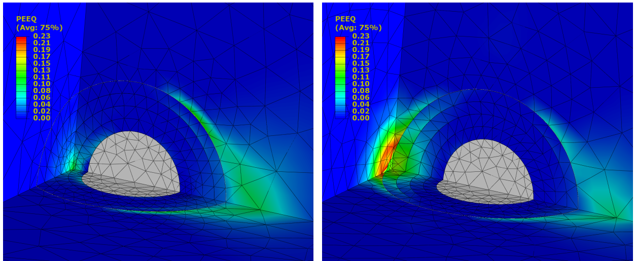
Figure 17: Equivalent plastic strain distributions around the particles at maximum overall strain \varepsilon^{FE} = 6\% for the close (left) and distant (right) situation.
