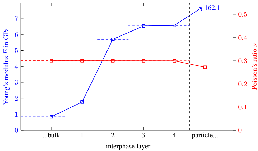
Figure 19: Optimal profiles for the elasticity parameters inside the interphases.
