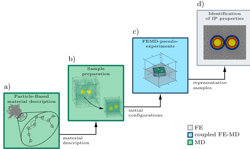
Figure 2: Graphical outline: The behavior of the investigated polymer is prescribed via a particle-based material description, which enables the preparation of our samples. The resulting initial configurations are used in subsequent, coupled MD-FE pseudo-experiments. Representative samples are chosen to identify interphase properties in an FE framework.
