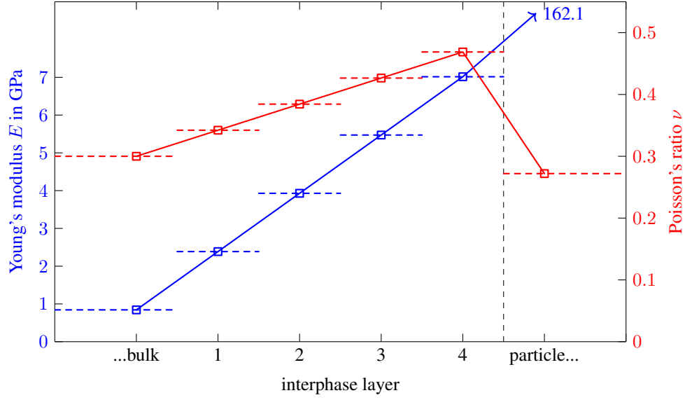
Figure 15: Optimal linear profiles for the elasticity parameters inside the interphases.
