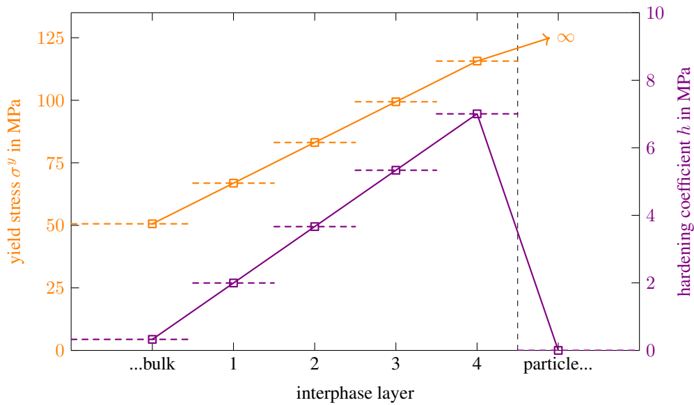
Figure 16: Optimal linear profiles for the plasticity parameters inside the interphases.
