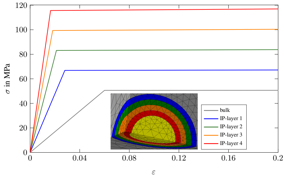
Figure 18: One-dimensional stress-strain curves for bulk polymer and the four interphase layers as resulting from the optimization of elastoplastic material behavior with linear property gradients.
