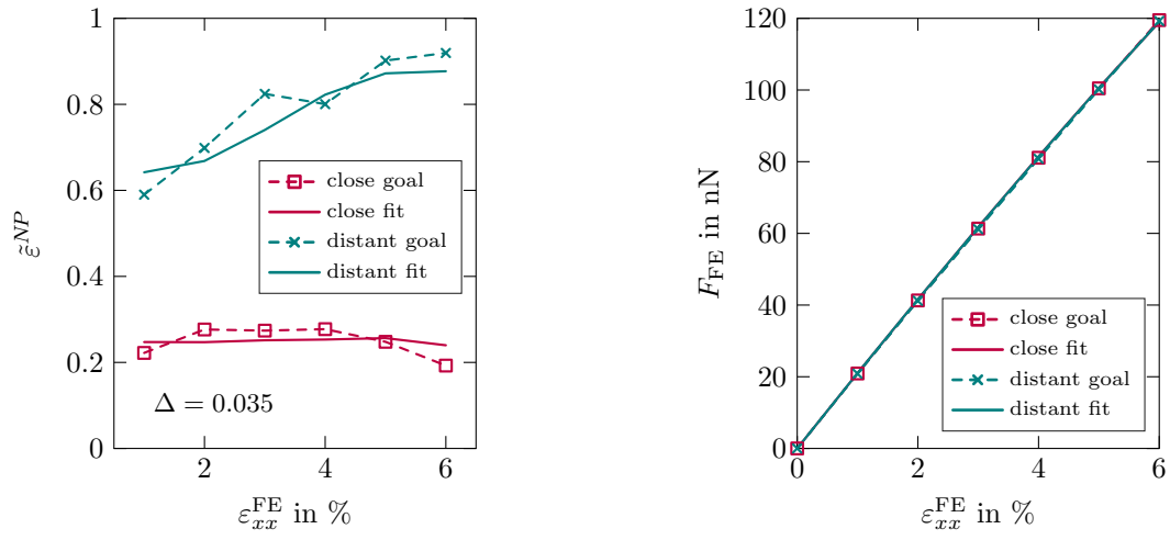
Figure 22: FE simulation results vs. Capriccio data for the close and distant cases with optimized exponential saturation profiles of the elastoplastic parameters inside the interphases: Profiles of normalized interparticle strain (left) and overall force (right).
