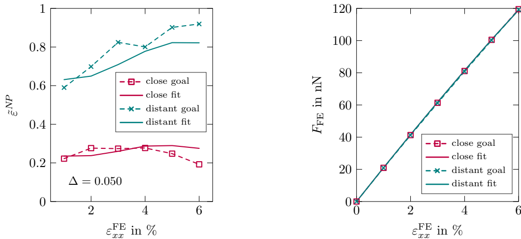
Figure 14: FE simulation results vs. Capriccio data for the close and distant cases with optimized linear profiles of the elastoplastic parameters inside the interphases: Profiles of normalized interparticle strain (left) and overall force (right).
