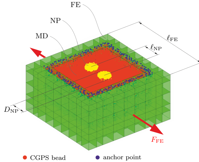
Figure 5: Deformed pseudo-experimental setup: Two spherical silica nanoparticles of diameter D_{NP} = 4 nm inside a polystyrene matrix, enclosed by anchor points and surrounding FE mesh, with deformed edge length \ell_{FE} , resulting external force F_{FE} and interparticle distance \ell_{NP} , depicted in 'ideal' conformation (no rotation of MD-box required).
