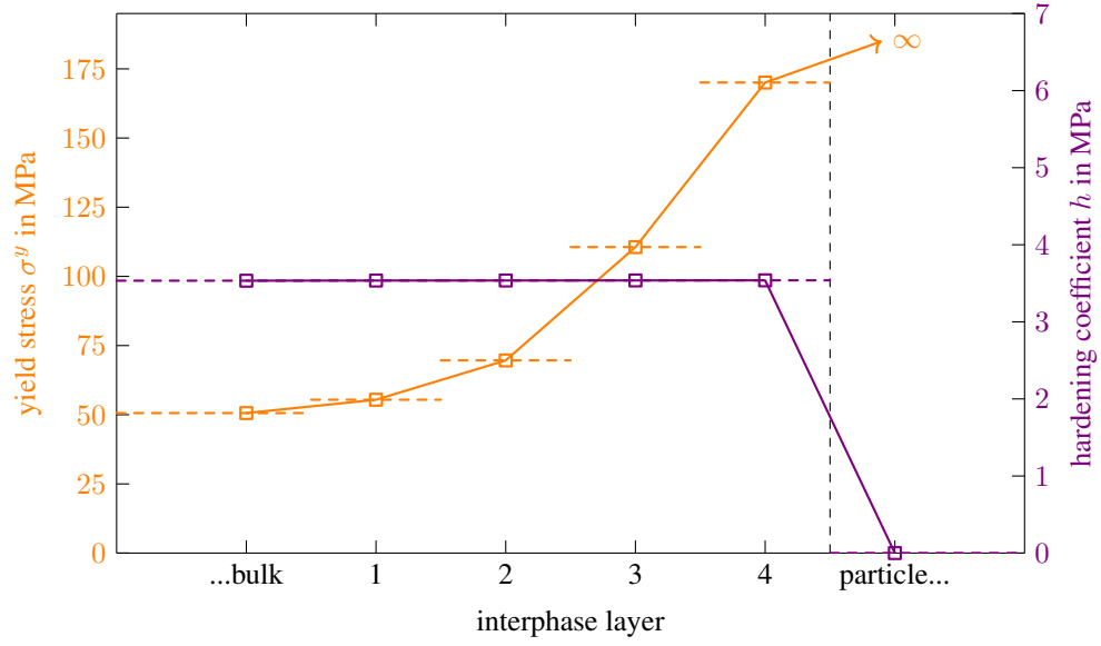
Figure 20: Optimal exponential saturation profiles for the interphase plasticity parameters.
