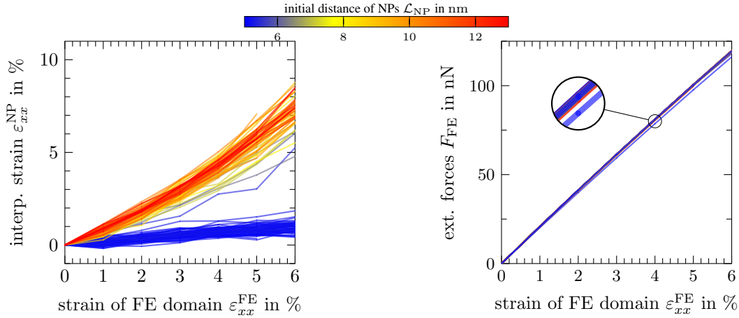
Figure 6: Influence of initial distance of NPs on uniaxial pseudo-experiments: Resulting external forces in deformation direction F_{\text{FE}} (right) and interparticle strain \varepsilon_{xx}^{\text{NP}} (left), versus strain of FE domain \varepsilon_{xx}^{\text{FE}} , respectively.
