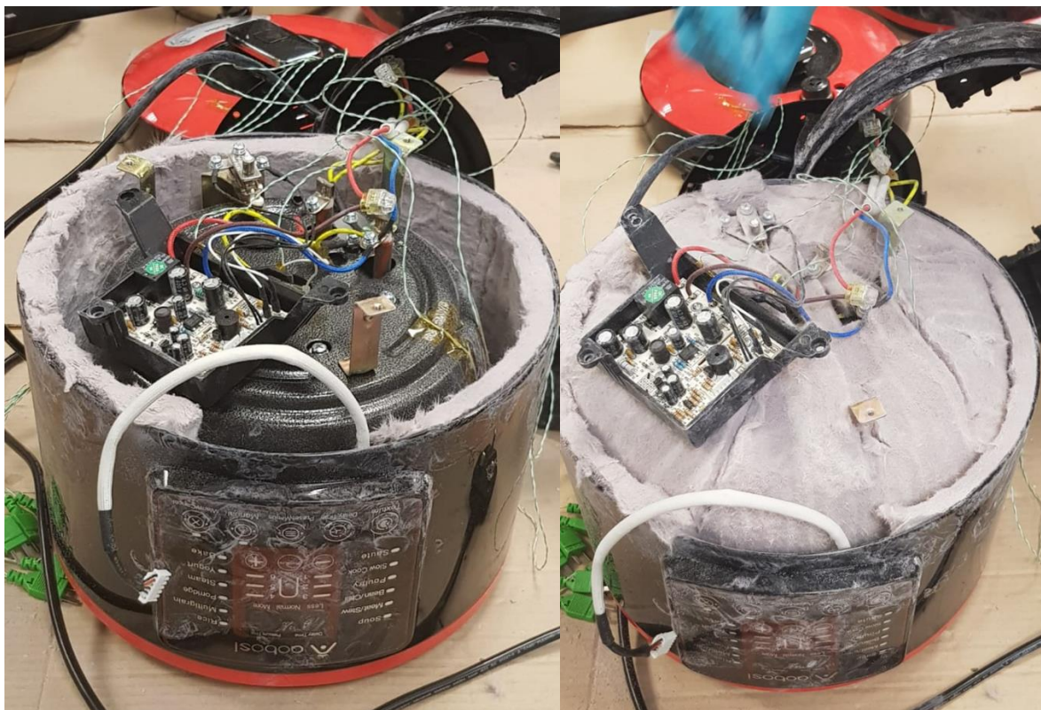
Figure 2 During installation. Handling Pyrogel XTE insulation required full PPE - photographs of view from beneath the EPC with base support and cover removed. Other Aspen Aerogels products have different handling qualities.
