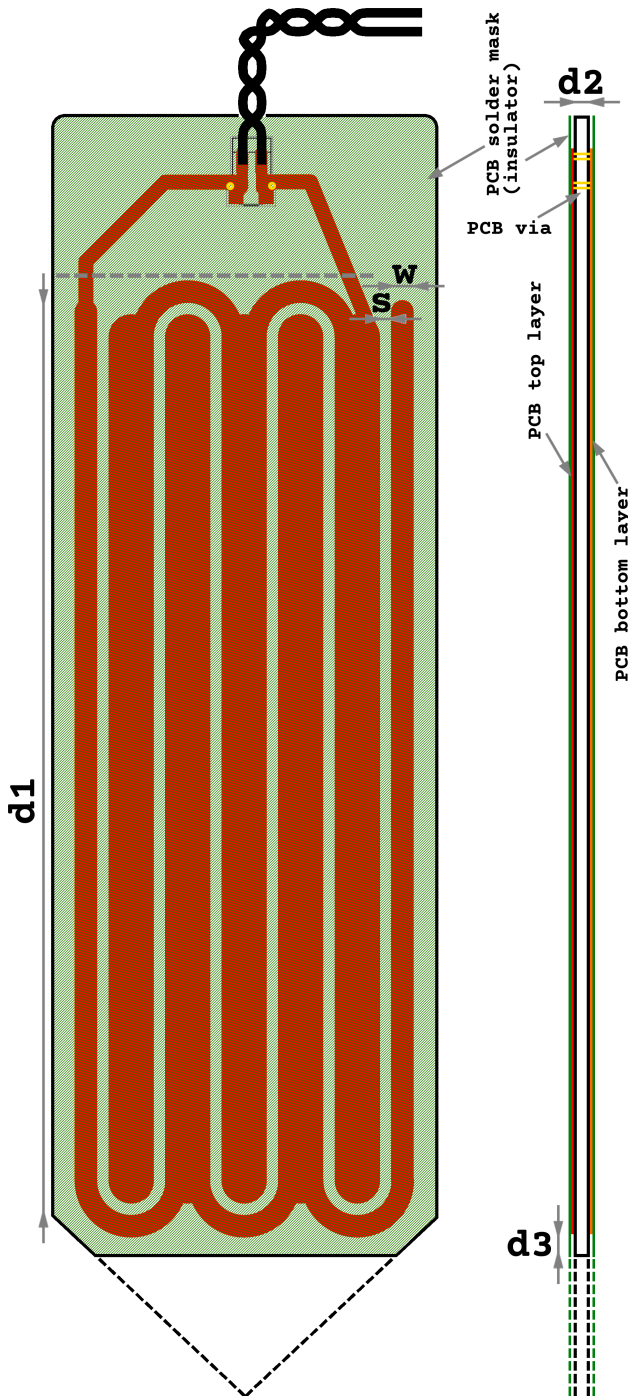
Figure 42: Diagram of 2-sided PCB (both layers have the same shape) of water (or fluid) level sensor or soil moisture sensor (with dashed line edge).
