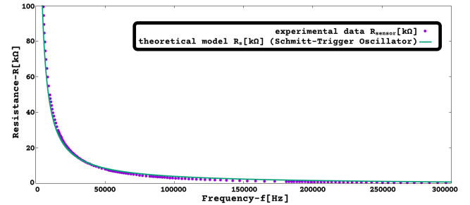
Figure 12: R_s(f) [kΩ], frequency in [0Hz, 300kHz] (Schmitt-trigger oscillator, Multiple-Sensor Interface with resistive sensor).
