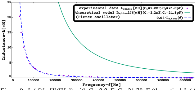
Figure 9: L_s(f) [mH]([Hz]) with C_1=2.2\text{nF} , C_2=21.78\text{pF} (theoretical L_s(f) as a Pierce osc.).
