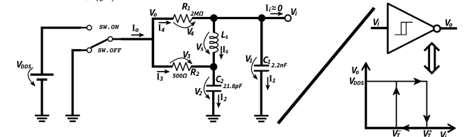
Figure 24: Multi-Sensor Int., inductive sensor (Schmitt-trigger osc.)
