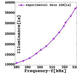
Figure 3: Plot experimental data with line, LDR light (brightness) sensor connected on Multiple-Sensor Interface; example of a calibration table exclusively from experimental data.
