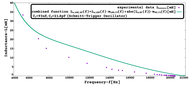
Figure 38: L_{s,LMF,HF}(f) [mH], with C_1=93\text{nF} , C_2=21.78\text{pF} , frequency in [4500Hz, 21500Hz] (Sch-trig. osc., Multi-Sensor w. inductive sensor)
