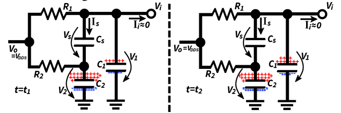
Figure 33: Schematic of RC network of the Schmitt-trigger osc. with a representation of electrical charge on C_1 , C_2 at t=t_1 and t=t_2 .
