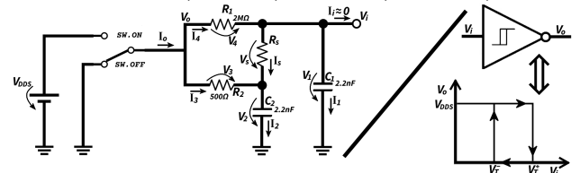
Figure 11: Multi-Sensor Int., resistive sensor (Schmitt-trigger osc.)
