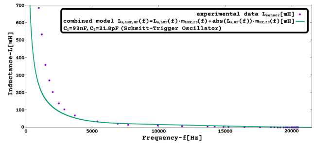
Figure 41: L_{s,LMF,HF}(f) [mH] versus frequency[0Hz, 21500Hz], with C_1=93\text{nF} , C_2=21.78\text{pF} (Sch-Trig. osc., Multi-Sensor w. inductive sensor)
