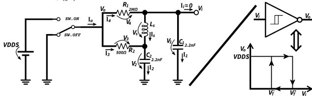
Figure 24: Multi-Sensor Int., inductive sensor(Schmitt-trigger osc.)
