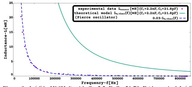
Figure 9: L_s(f) [mH]([Hz]) with C_1=2.2nF , C_2=21.78pF (theoretical L_s(f) as a Pierce Osc.).
