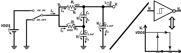
Figure 13: Multi-Sensor Int., capacitive sensor (Schmitt-trigger osc.)
