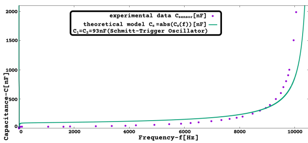
Figure 39: C_s [nF] versus frequency[0Hz, 10500Hz] by |C_s(f)| , with C_1=C_2=93\text{nF} (Schmitt-Trigger osc., Multi-Sensor with capacitive sensor)
