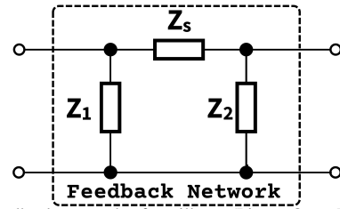
Figure 37: Feedback network of oscillator (Pierce Osc., Multiple-Sensor Int. with inductive sensor).
