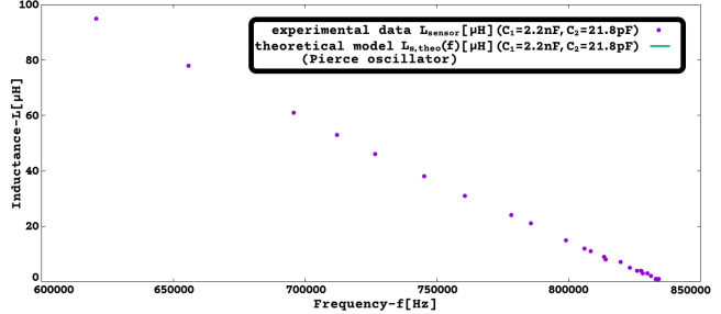
Figure 10: Experimental data of L_s in [0\mu H; 100\mu H] , with C_1=2.2nF , C_2=21.78pF (theoretical L_s(f) as a Pierce Osc. is out of plot range).
