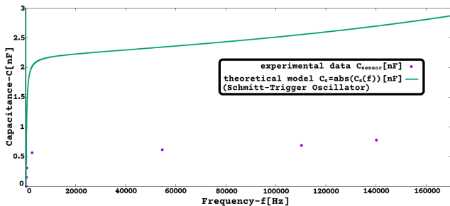
Figure 16: C_s [nF] versus frequency[0Hz, 170kHz] by |C_s(f)| (Schmitt-Trigger osc., Multi-Sensor with capacitive sensor)
