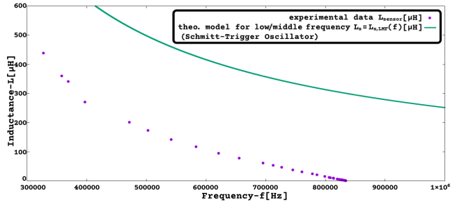
Figure 29: L_{s,LMF}(f) [ \mu H] versus frequency[300kHz, 1MHz] (Sch-Trig. Osc., Multi-Sensor Int. with inductive sensor, LMF approx. model).
