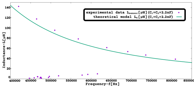
Figure 8: Frequency jump of L_s(f) [ \mu H ]([Hz]) with C_1=C_2=2.2nF (Pierce Osc., Multi-Sensor Int. with inductive sensor).
