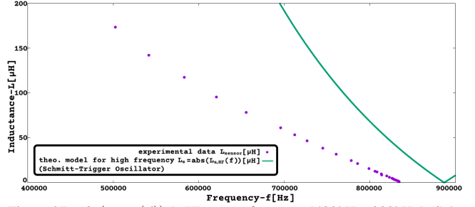
Figure 27: abs(L_{s,HF}(f)) [ \mu H] versus frequency[400kHz, 900kHz] (Sch-Trig. Osc., Multi-Sensor Int. with inductive sensor, HF approx. model).
