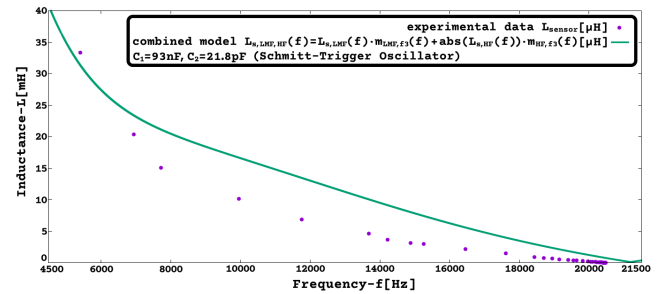
Figure 42: L_{s,LMF,HF}(f) [ \mu\text{H} ] versus frequency[4500Hz, 21500Hz], with C_1=93\text{nF} , C_2=21.78\text{pF} (Sch-Trig. osc., Multi-Sensor w. inductive sensor)
