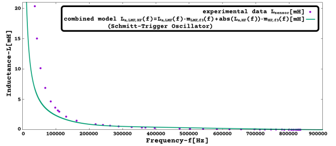
Figure 31: L_{s,LMF,HF}(f) [mH] versus frequency[0Hz, 900kHz] (Sch-Trig. Osc., Multi-Sensor Int. with inductive sensor, LMF and HF combined approx. model, with C_1 = 2.2\text{nF} , C_2 = 21.78\text{pF} ).
