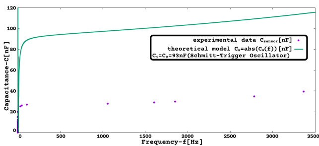
Figure 40: C_s [nF] versus frequency[0Hz, 3500Hz] by |C_s(f)| , with C_1=C_2=93\text{nF} (Schmitt-Trigger osc., Multi-Sensor with capacitive sensor)
