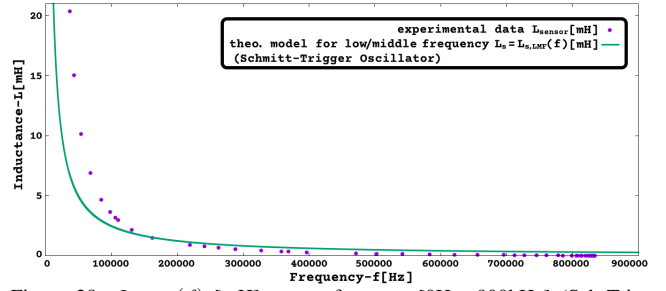
Figure 28: L_{s,LMF}(f) [mH] versus frequency[0Hz, 900kHz] (Sch-Trig. Osc., Multi-Sensor Int. with inductive sensor, LMF approx. model).
