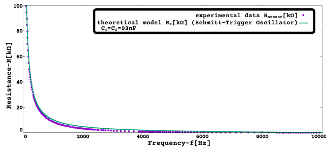
Figure 38: R_s [kΩ] versus frequency[0Hz, 10kHz], with C_1=C_2=93\text{nF} (Schmitt-Trigger Osc., Multiple-Sensor Int. with resistive sensor).
