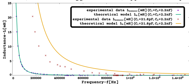
Figure 7: L_s(f) [mH]([Hz]) with C_1=C_2=2.2nF and C_1=21.78pF , C_2=2.2nF (Pierce Osc., Multi-Sensor Int. with inductive sensor)
