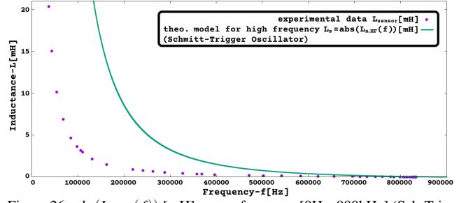
Figure 26: abs(L_{s,HF}(f)) [mH] versus frequency[0Hz, 900kHz] (Sch-Trig. Osc., Multi-Sensor Int. with inductive sensor, HF approx. model).
