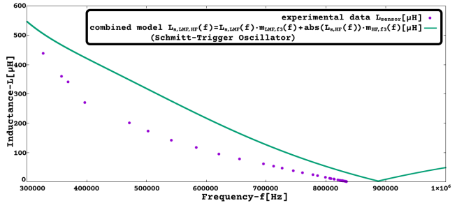
Figure 32: L_{s,LMF,HF}(f) [ \mu\text{H} ] versus frequency[300kHz, 1MHz] (Sch-Trig. Osc., Multi-Sensor Int. with inductive sensor, LMF and HF combined approx. model, with C_1 = 2.2\text{nF} , C_2 = 21.78\text{pF} ).
