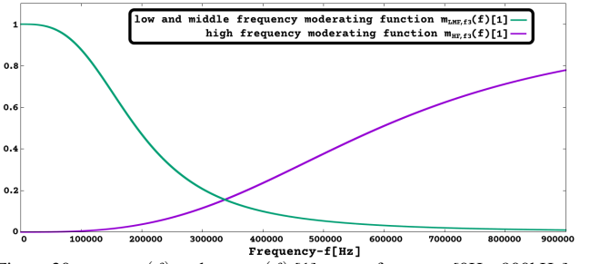
Figure 30: m_{LMF,f3}(f) and m_{HF,f3}(f) [1] versus frequency[0Hz, 900kHz].
