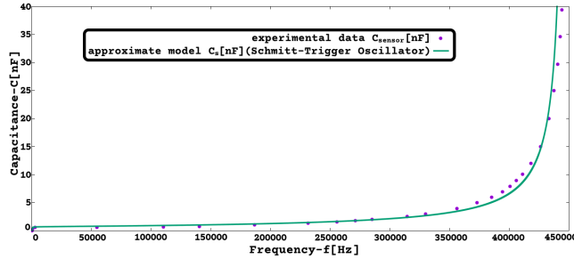
Figure 22: C_s [nF] versus frequency [0Hz, 450kHz] by approximate model ( C_{approx} , R_{approx} ; Multi-Sensor Int. with capacitive sensor)
