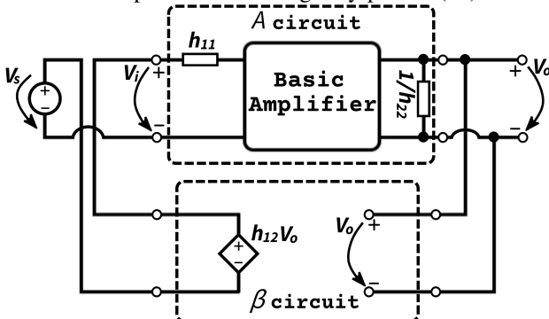
Figure 35: Simplified representation of oscillator circuit (Pierce osc.)
