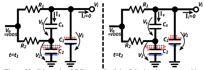
Figure 33: Schematic of RC network of the Schmitt-trigger osc. with a representation of electrical charge on C_1 , C_2 at t=t_1 and t=t_2 .
