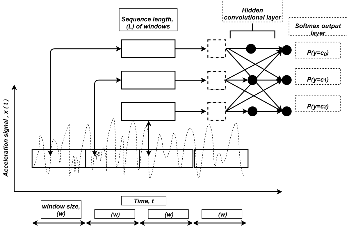
FIG. 2: Extracting data sequences of windows from the vibration data using 1D-CNN architecture.
