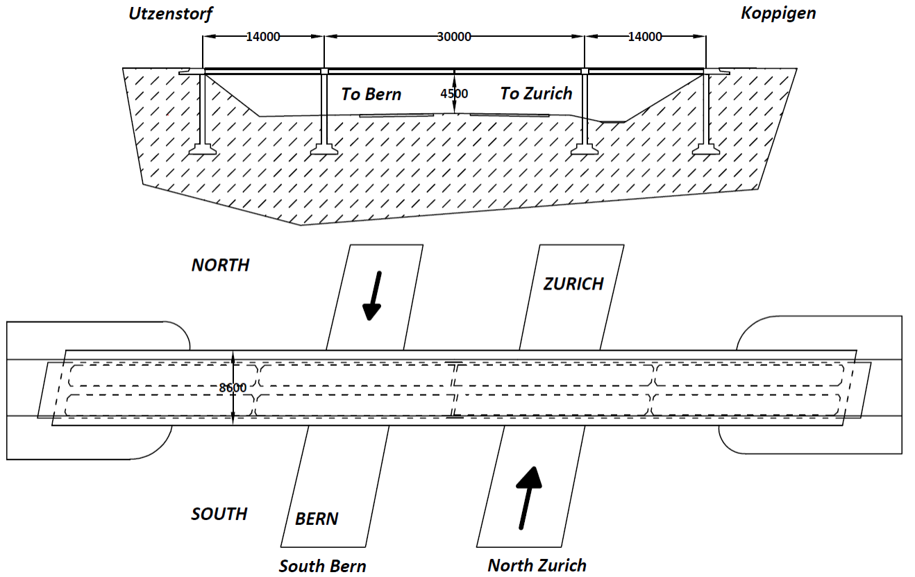
FIG. 4: Schematic of the Z24 bridge.
