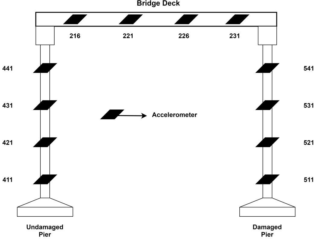
FIG. 9: Schematic showing sensor location and its numbers used in the analysis.
