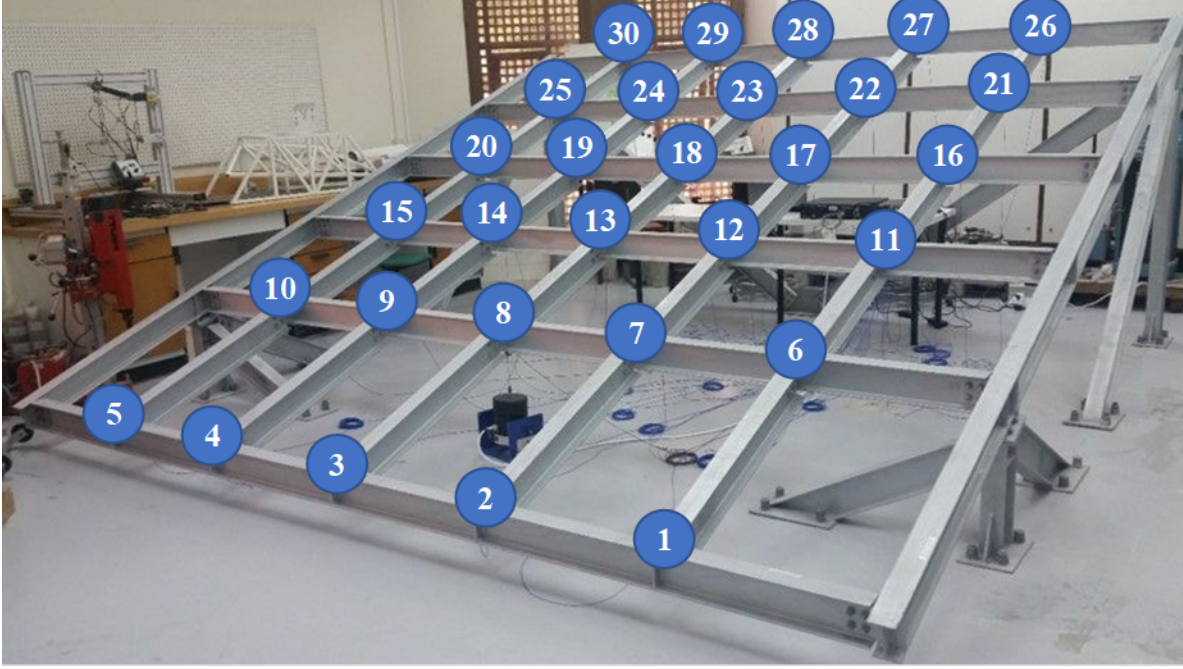
FIG. 4: QUGS testbed, where the joints are numbered from 1 to 30 (Abdeljaber et al. 2017).
