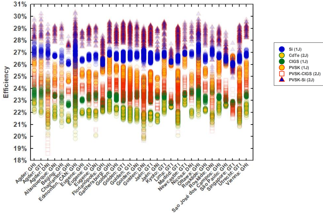
Figure 5. Efficiency as a function of location and orientation for cells with one or two junctions. Results for the III-V multijunctions are included in Appendix D. Each data point is a weekly sum sampled at 10-minute intervals (except for Chajnantor, CHL: 60-minute intervals).
