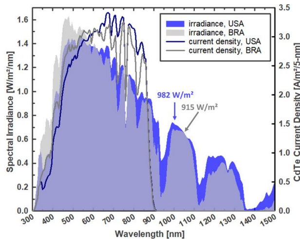
Figure 8. Spectral irradiance and the resulting current density for cadmium telluride from selected weekly summations in Albuquerque (USA) and Sao José dos Campos (BRA). Cadmium telluride has a spectral response range of ~300-900 nm. The two current density lines form equal areas.
