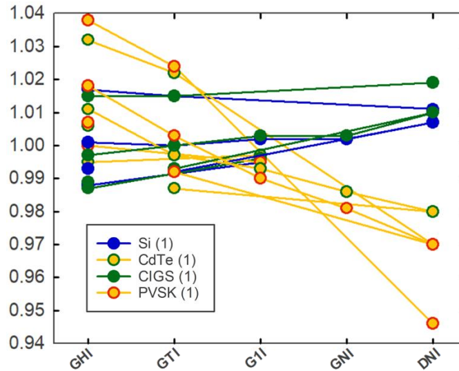
Figure 13. Comparison of relative median efficiency of single-junction cells for sites with more than one sensor orientation: Agder, NOR; Eugene, USA; Golden, USA; Roskilde, DEN.
