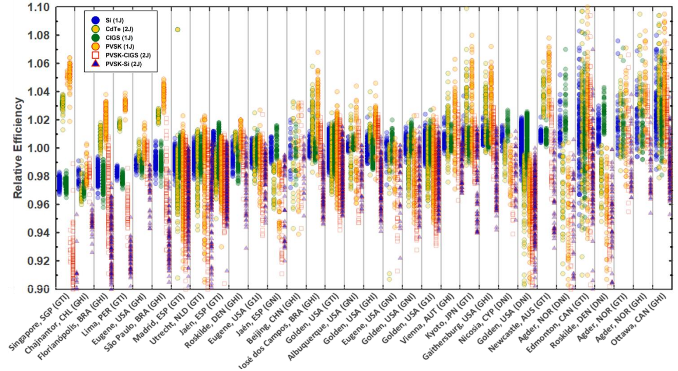
Figure 6. Relative efficiency vs. location and orientation for cells with one or two junctions. Data is sorted by increasing median efficiency of silicon. Location names are approximate. Each data point is a weekly sum from spectral irradiance sampled at 10-minute intervals (except for Chajnantor, CHL: 60-minute intervals).
