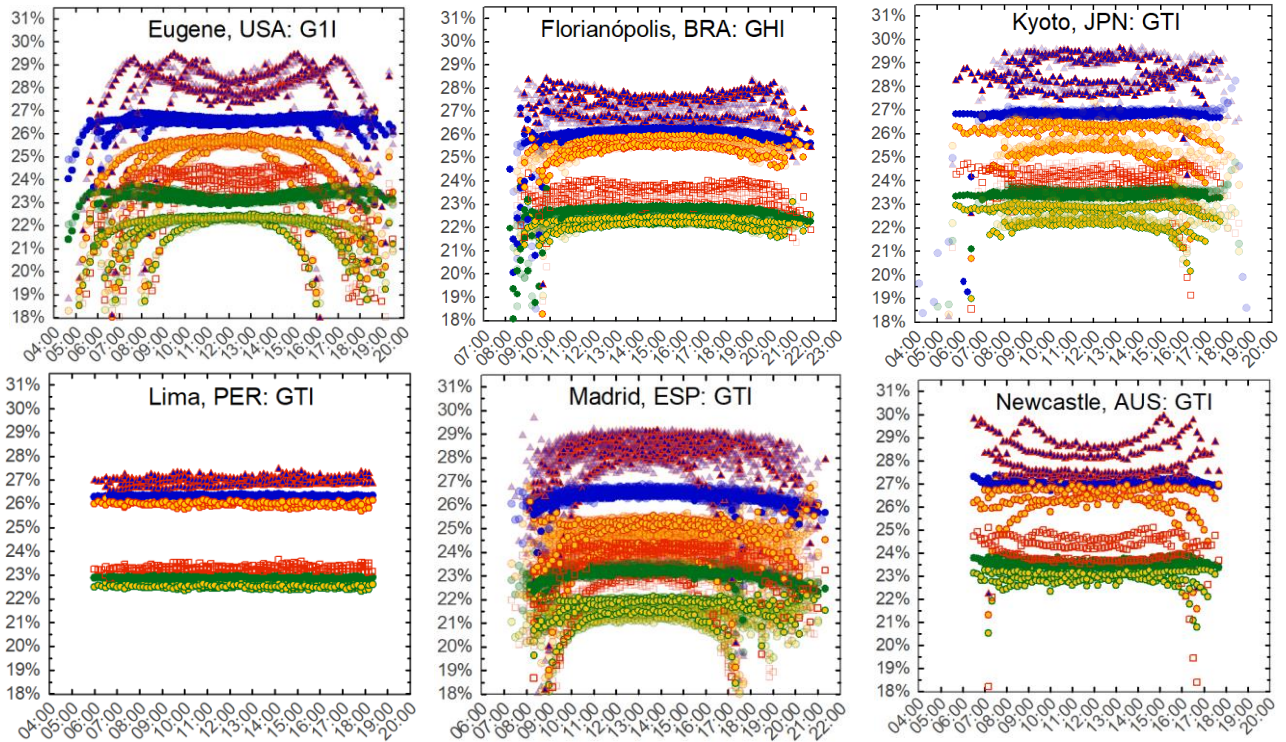
Figure 8. Sample seasonal and diurnal efficiency variations for cells with one or two junctions. Seasonal changes are delineated using one month of data for March, June, September, and December. Where available, data from additional years is semi-transparent in the background. Each data point is a monthly sum. Results for all locations are shown in Appendix F. (Refer to Figure 7 for the legend.)
