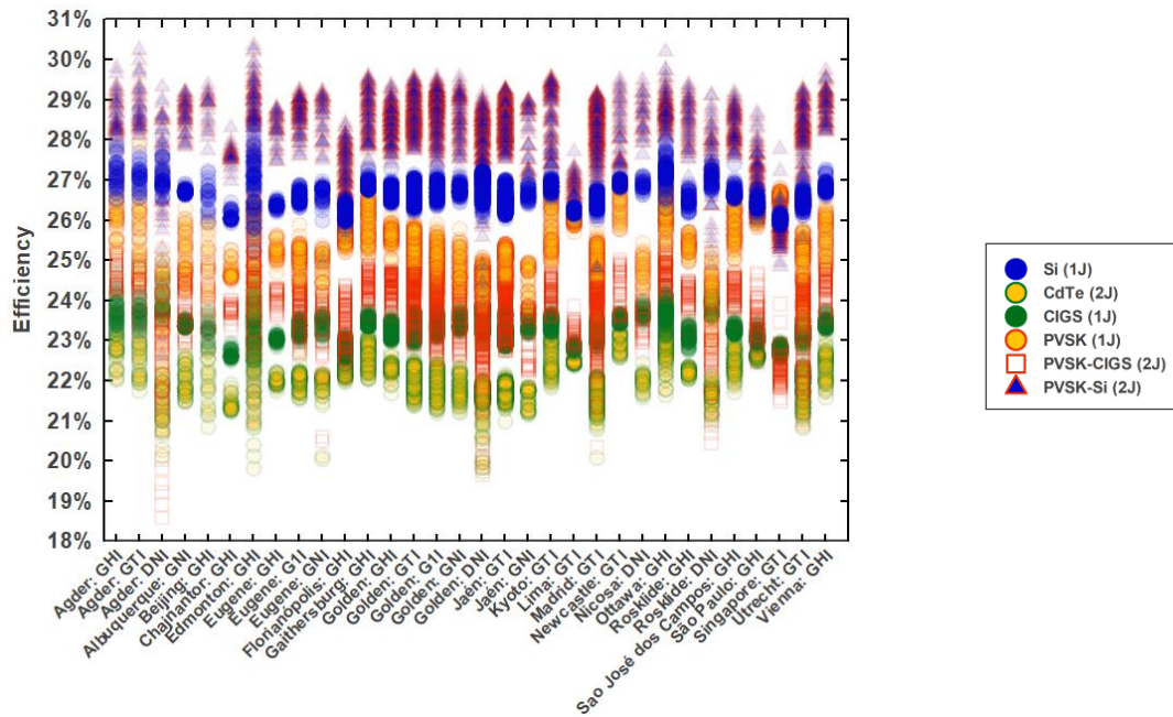
Figure 6. Efficiency as a function of location and orientation for cells with one or two junctions. Results for the III-V multijunctions are included in Appendix D. Each data point is a weekly sum sampled at 10-minute intervals (except for Chajnantor: 60-minute intervals).
