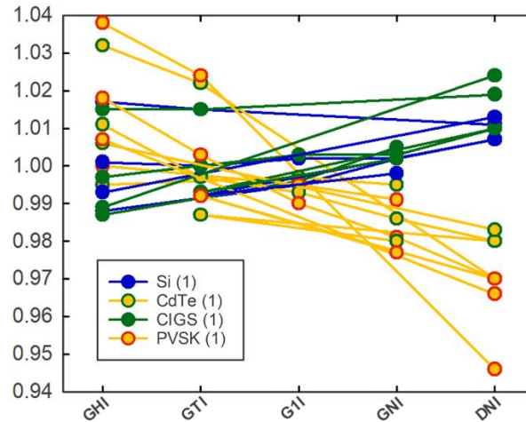
Figure 13. Comparison of relative median efficiency of single-junction cells for sites with more than one sensor orientation: Agder, NOR; Eugene, USA; Golden, USA; Jaén, ESP; Roskilde, DEN.
