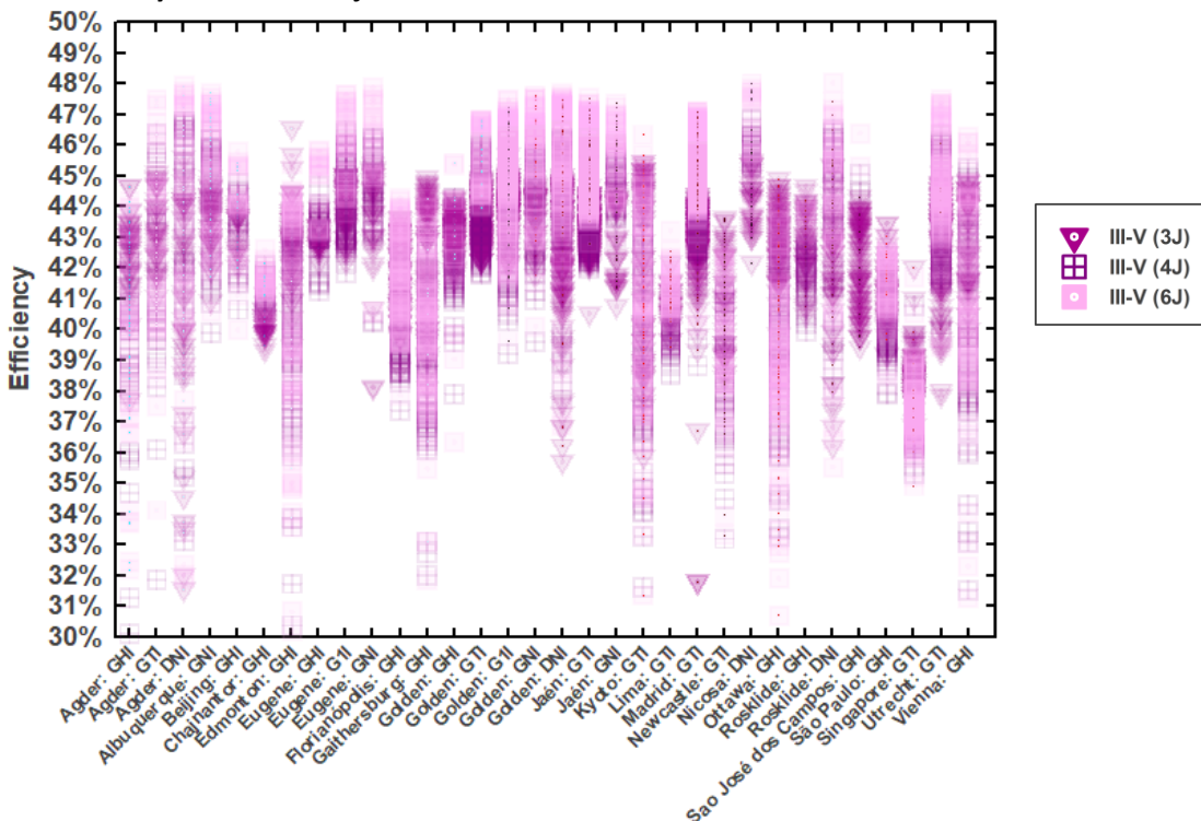
Figure 10. Efficiency as a function of location and orientation for III-V multijunction cells.
