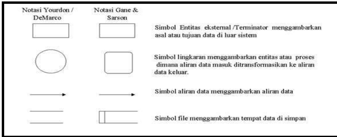
Gambar 1. Simbol-simbol DFD
