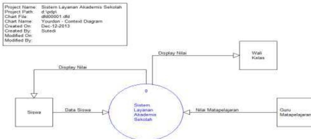
Gambar 6. Context diagram
