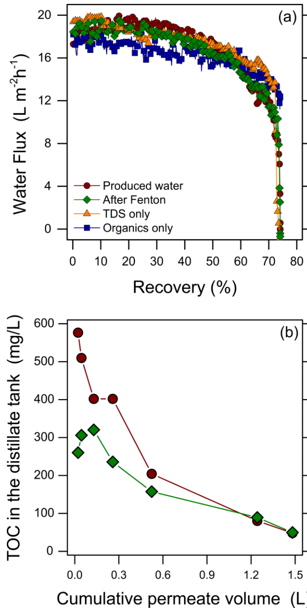
332 Figure 2 (a) Results of MD filtration tests with different feed solutions: (red circles) synthetic 333 produced water, (blue squares) only the organic content of the synthetic produced water, 334 (orange triangles) only the TDS content of the synthetic produced water, and (green 335 diamonds) the resulting feed after the thermal Fenton oxidation. (b) TOC concentration in the 336 distillate tank (initial volume 1 L) as a function of cumulative permeated volume; the lines 337 connecting the data points are only intended as guides for the eye.
