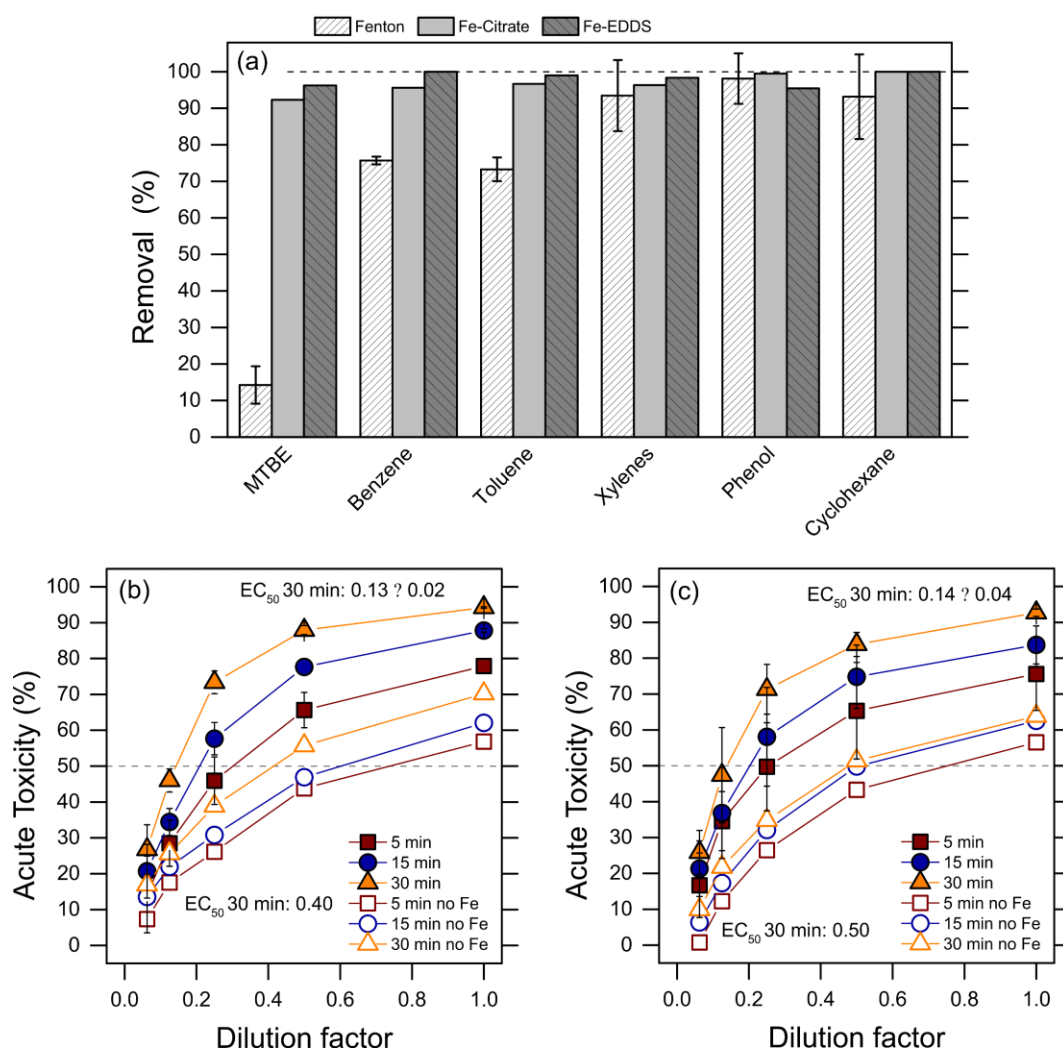
Figure 4 (a) Comparison of the organics removal rate by traditional Fenton and modified Fenton reactions with citrate and EDDS as iron ligands. Residual toxicity of the final effluent
