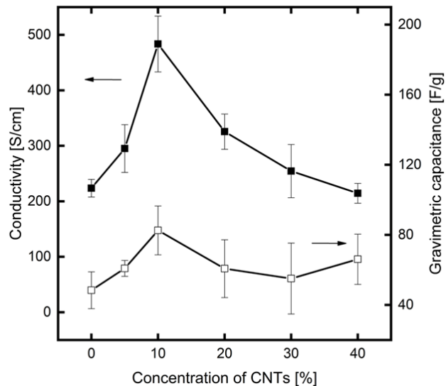
Figure 3. Conductivity and Capacitance of PEDOT:PSS and PEDOT:PSS/CNT composite flat sheets with CNT loadings between 0 wt.% and 40 wt.% (Each point represents the mean value of at least three independent measurements. The error bars represent the respective standard deviation).
