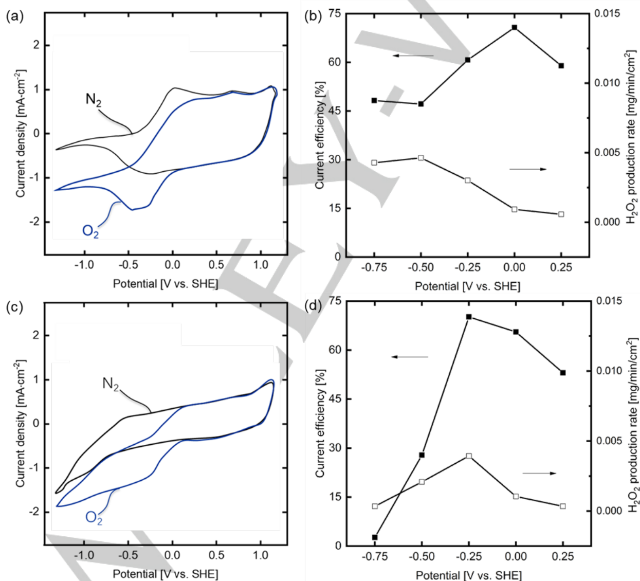
Figure 4. Cyclic voltammetry of flat sheet electrodes under N 2 and O 2 gassing: (a) PEDOT:PSS; (c) 40 wt.% PEDOT:PSS/CNT composite. Current efficiency and H 2 O 2 production rate calculated from potentiostatic experiments at 5 different potentials: (b) PEDOT:PSS; (d) 40 wt.% PEDOT:PSS/CNT composite.
