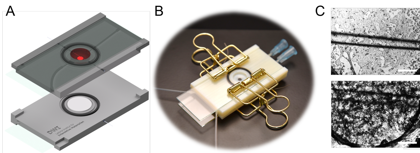
Figure 5: (A) CAD model of the bioreactor displaying the two half cells with a membrane in between. The two glass slides on top and below serve as current-injecting electrodes, and the wires through the upper and lower cultivation chambers are the voltage pick-up electrodes. (B) Image of the assembled bioreactor. (C) Microscopy images of Caco-2 cells cultivated in the bioreactor after one day (upper image) and after 10 days (lower image). The shadows from left to right are the platinum wires serving as voltage pick-up electrodes. The scale bar represents 500 \mu\text{m} .
