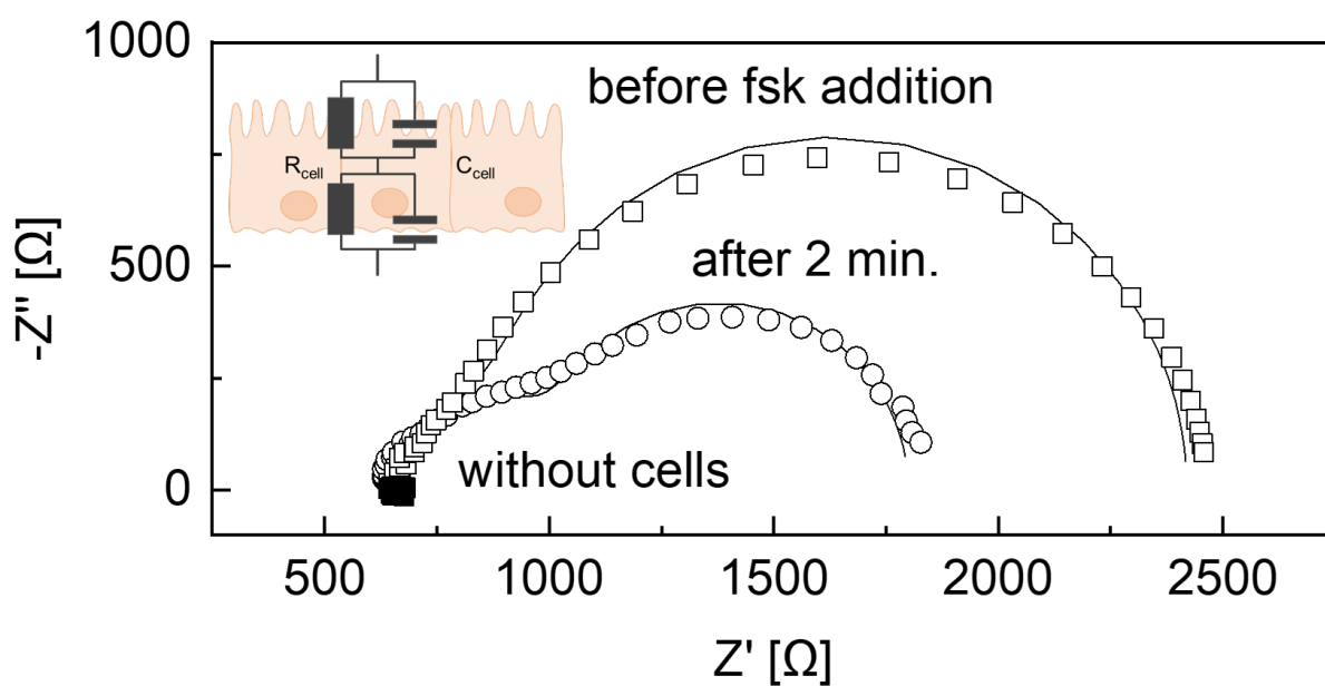
Figure 3: EIS measurement of a Caco-2 layer between 10 Hz and 30 kHz in Nyquist plot representation before and two minutes after the contact with forskolin. The data were fitted with the equivalent circuit in the graph taking the different apical and basolateral sides into account. For comparison, an EIS spectrum without cells is presented showing only the medium resistance.
