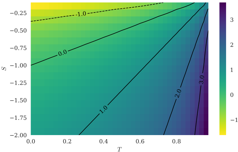
Figure 3. Risk dominance ( R ) contours as a function of variable payoffs S and T .
