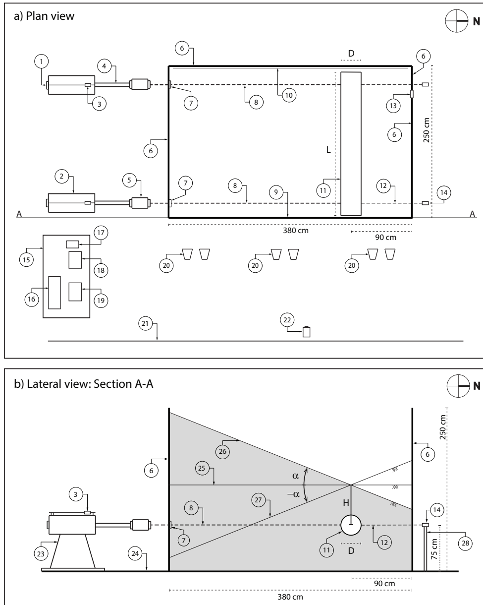
Fig. 3. Plan and lateral view of the testing equipment—identification is described in Table 2
