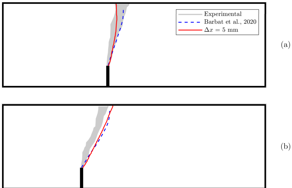
Figure 13: Experimental and numerical crack paths for the mixed mode fracture tests ( d = 320\text{mm} ). Notch eccentricity \mu d : (a) 0.3125d , and (b) 0.625d
