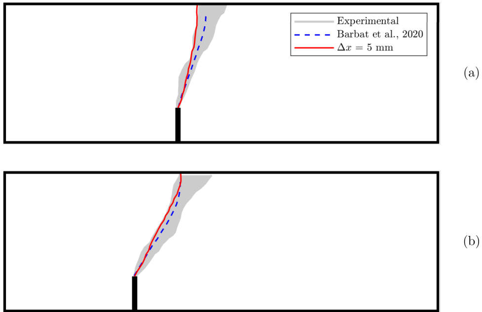
Figure 12: Experimental and numerical crack paths for the mixed mode fracture tests ( d = 160\text{mm} ). Notch eccentricity \mu d : (a) 0.3125d , and (b) 0.625d
