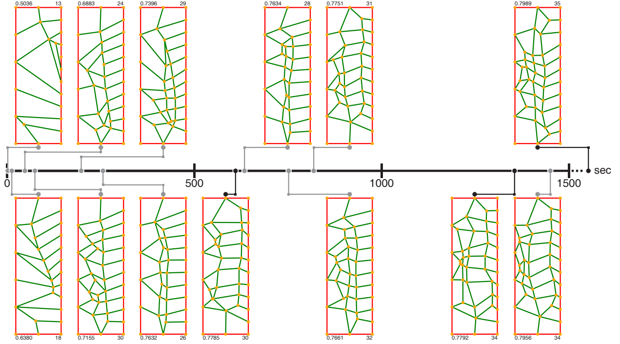
Figure 8: Mesh methods with 3 residual blocks and the MCTS method in a "11 \rightarrow 5" seed-density-changing boundary. DPPO results are linked with grey lines, while MCTS results are linked with black lines.
