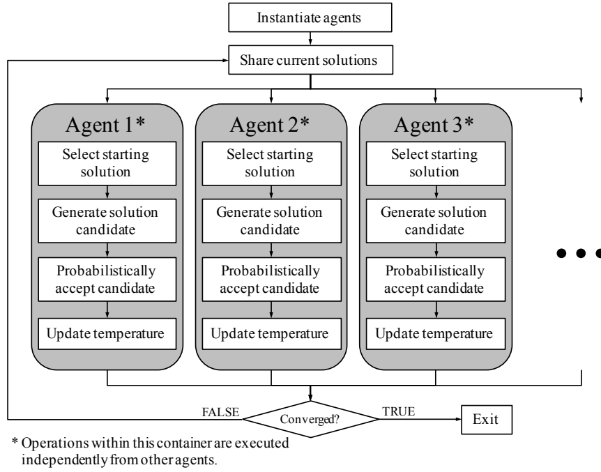
Figure 2. Flowchart for the HSAT algorithm.
