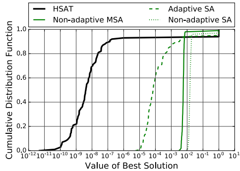
(a) Cumulative distribution of terminal solutions. (b) Geometric mean of best solution found over time.
