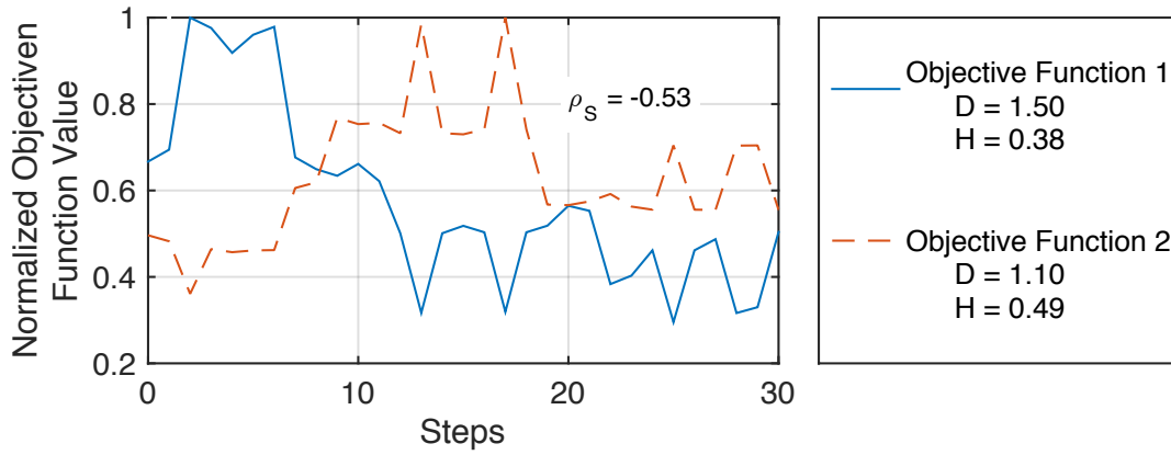
FIGURE 3. RANDOM WALK EXAMPLE.
