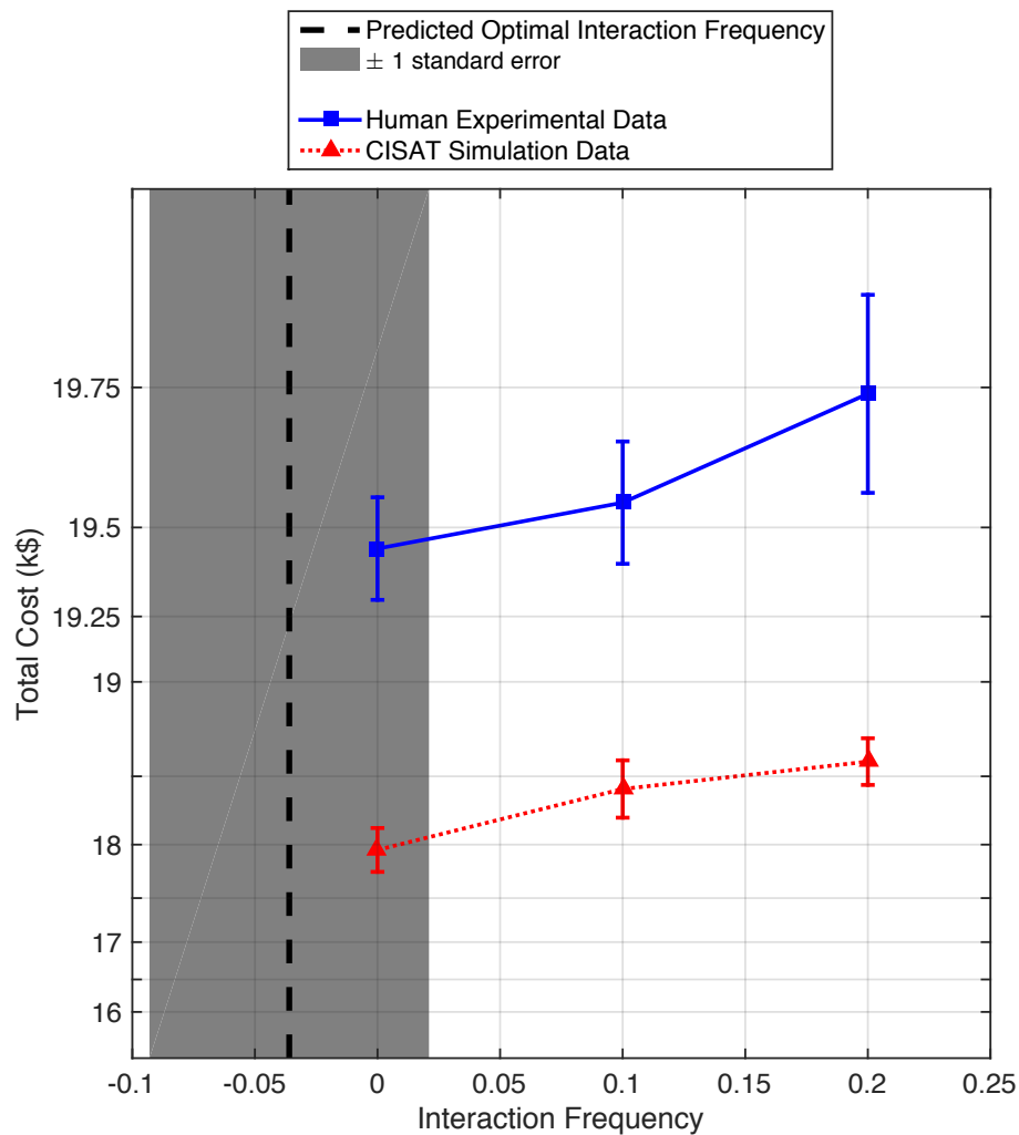
FIGURE 9. QUALITY OF BEST SOLUTIONS WITH RESPECT TO TOTAL COST. ERROR BARS INDICATE \pm 1 STANDARD ERROR.
