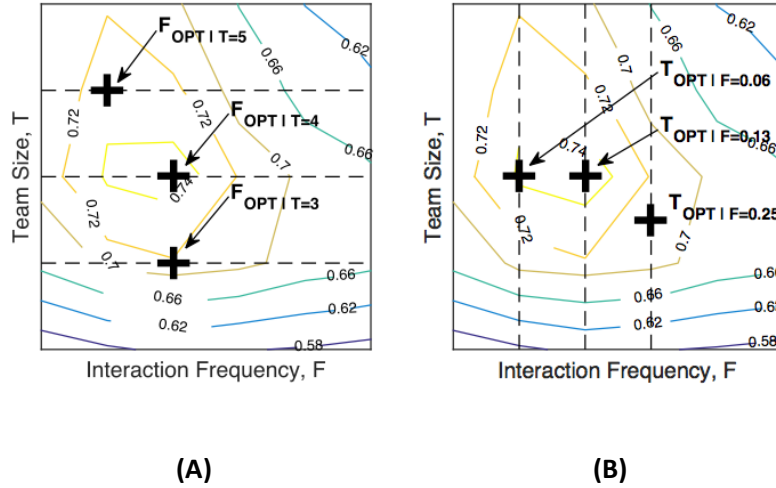
FIGURE 4. DETERMINING THE OPTIMAL TEAM CHARACTERISTICS FOR (A) CASE A AND (B) CASE B.
