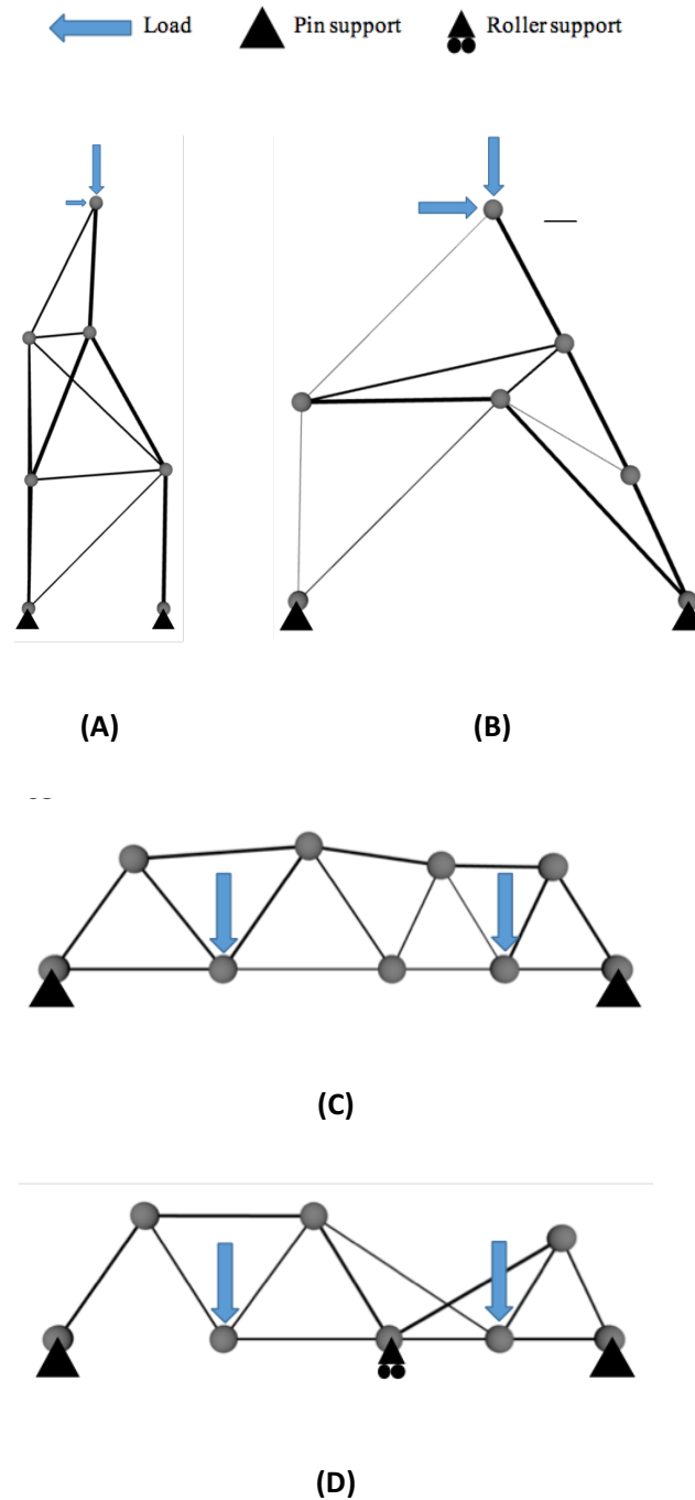
FIGURE 1. EXAMPLE SOLUTIONS TO STRUCTURAL DESIGN PROBLEMS, SHOWING REQUIRED LOADS AND SUPPORTS: (A) NARROW-BASE TOWER LAYOUT, (B) WIDE-BASE TOWER LAYOUT, (C) SINGLE-SPAN BRIDGE LAYOUT, (D) DOUBLE-SPAN BRIDGE LAYOUT.
