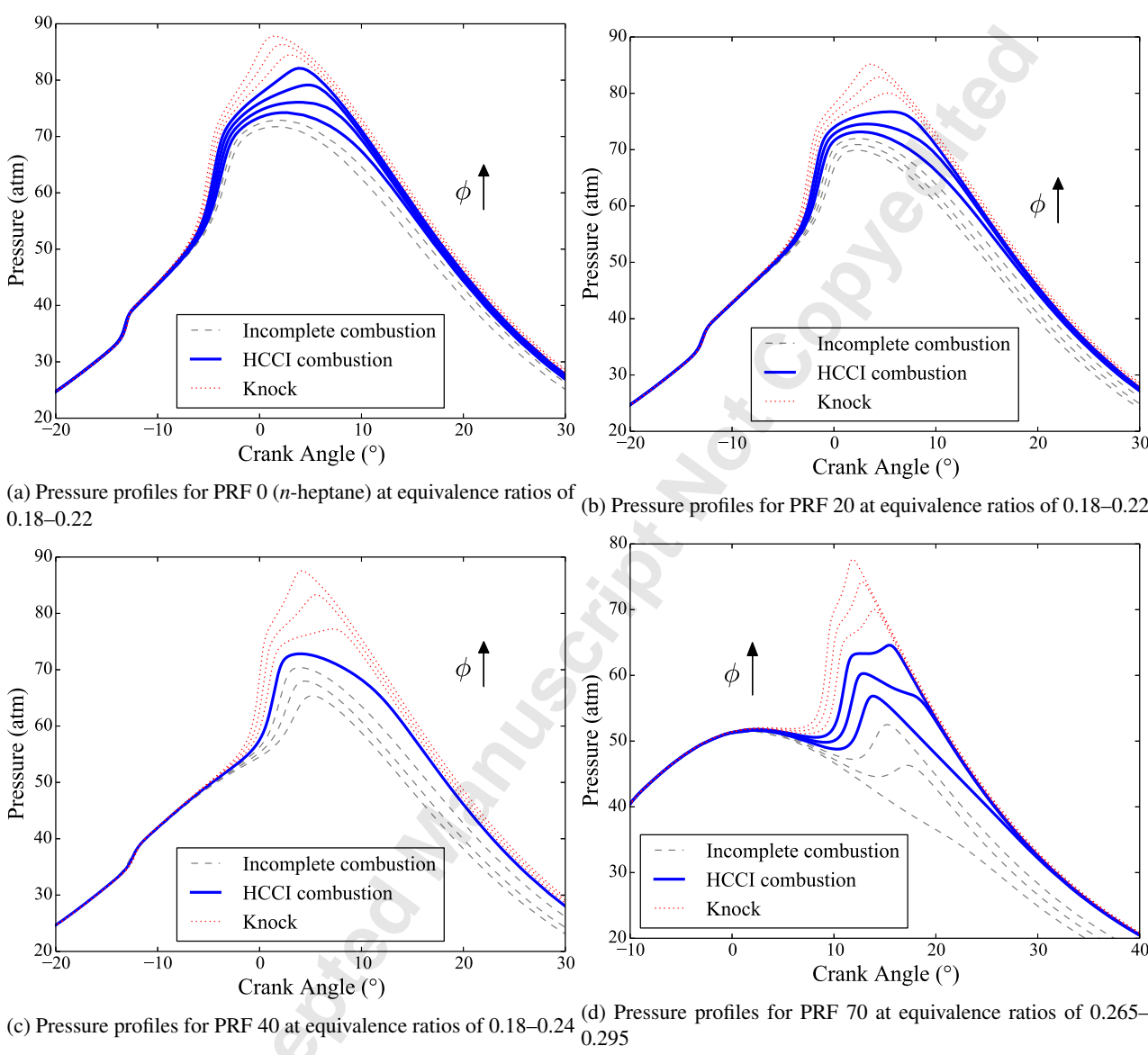
Figure 5: Pressure profiles for the fuels at 1200 rpm and various equivalence ratios
