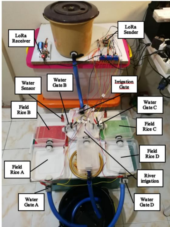
Figure 15. Prototype of smart farm irrigation system
