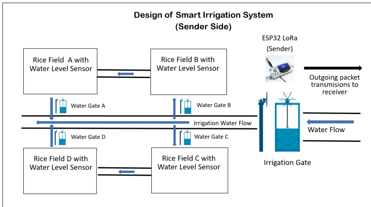
Figure 5. Irrigation system design
