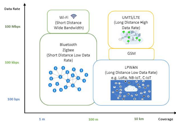
Figure 4. Comparisons of communication coverage and data rate in wireless technologies [17]
