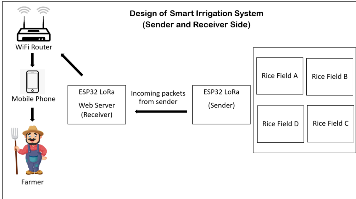
Figure 5. Monitoring system design
