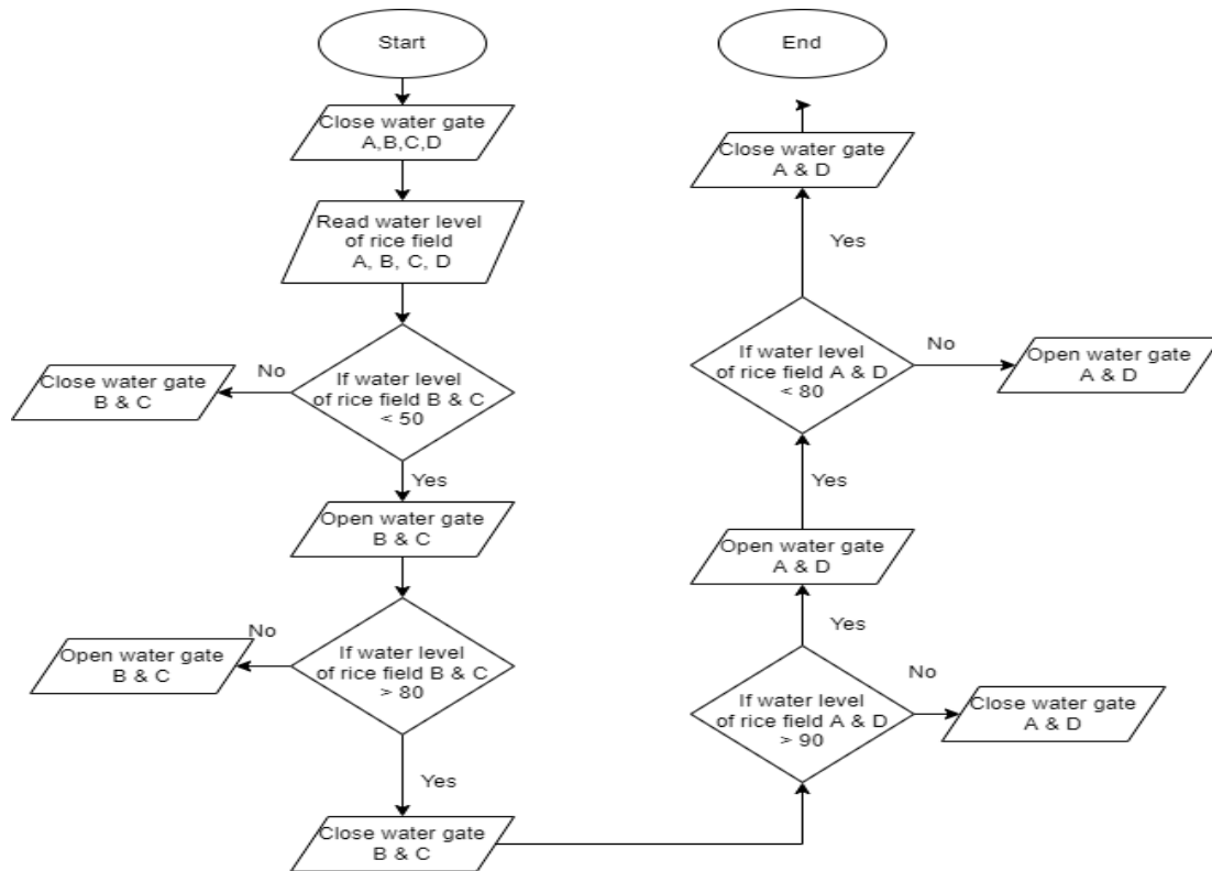
Figure 12. The flowchart of smart irrigation system at the sender
