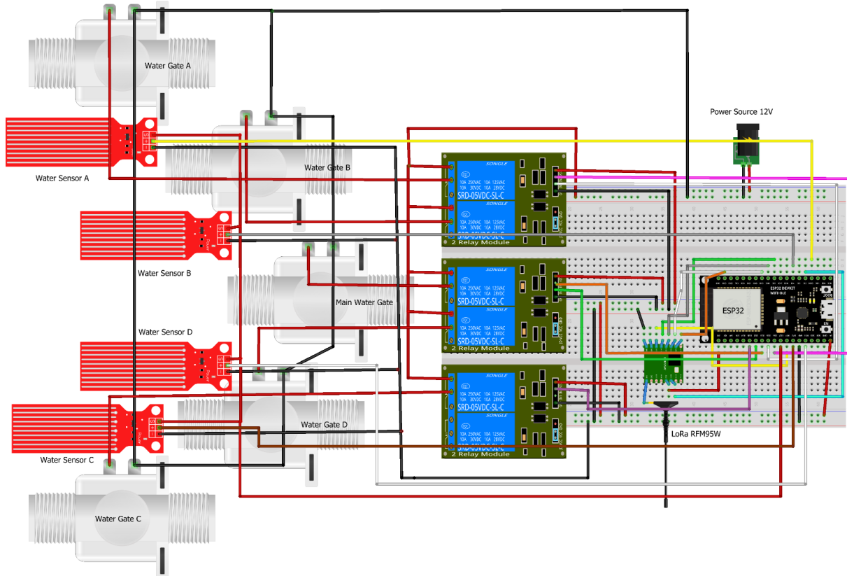
Figure 11. Schematic of smart irrigation system at the sender
