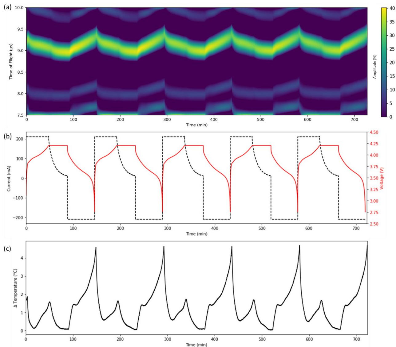
Figure 8 five cycles at 1C of a 210 mAh pouch cell. (a) colourmap illustrating the change in position and amplitude of the 'first echo' time-of-flight peak (b) the voltage change and applied current (c) cell temperature variations while being cycled
