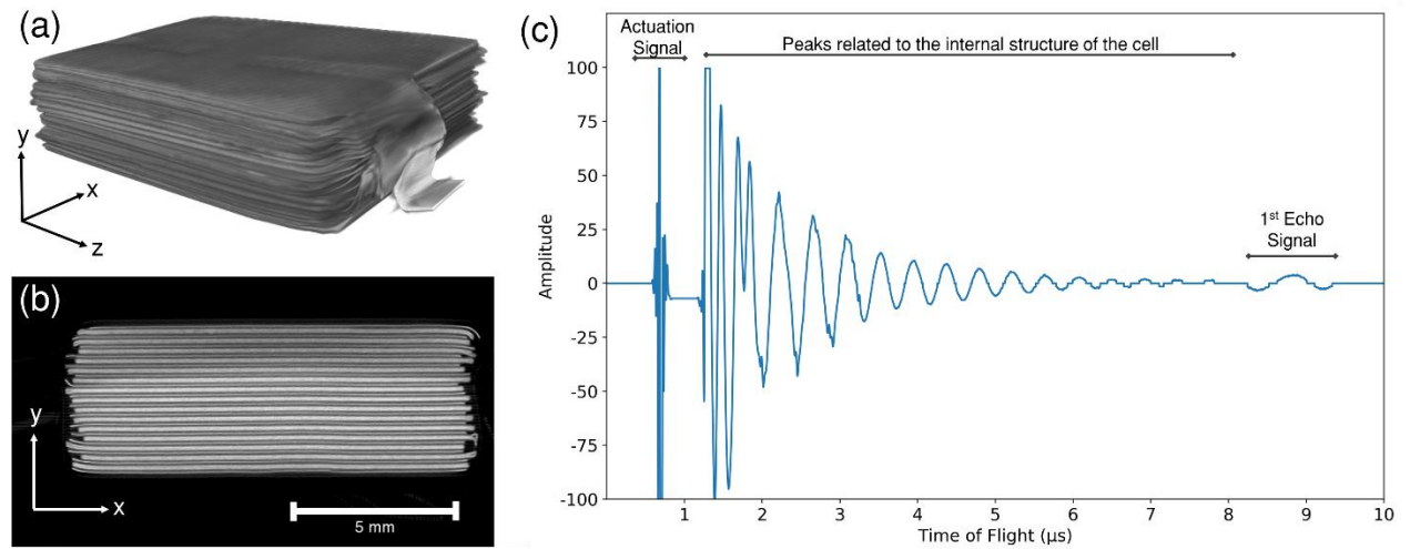
Figure 1(a) 3D volume rendering of the internal electrode stack structure of the 210 mAh cell under study. (b) An orthogonal slice of the electrode stack showing the alternating layered electrodes. (c) A typical acoustic signal obtained by probing a 210 mAh pouch cell using an ultrasonic pulse-echo technique.
