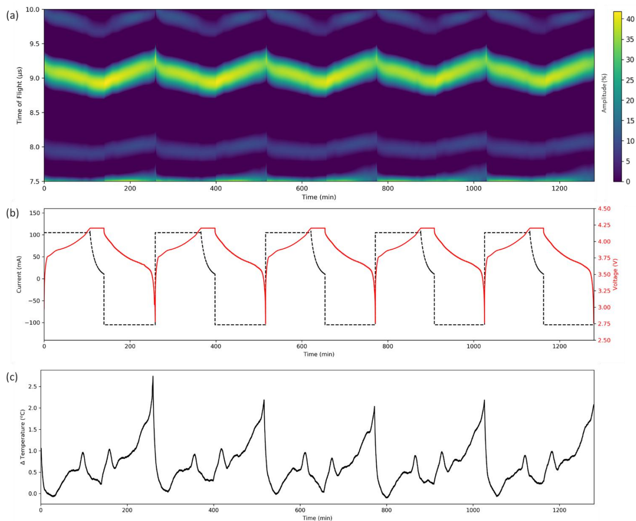
Figure 7 Five cycles at C/2 of 210 mAh pouch cell. (a) colourmap illustrating the change in position and amplitude of the 'first echo' time-of-flight peak (b) the voltage change and applied current (c) cell temperature variations while being cycled.
