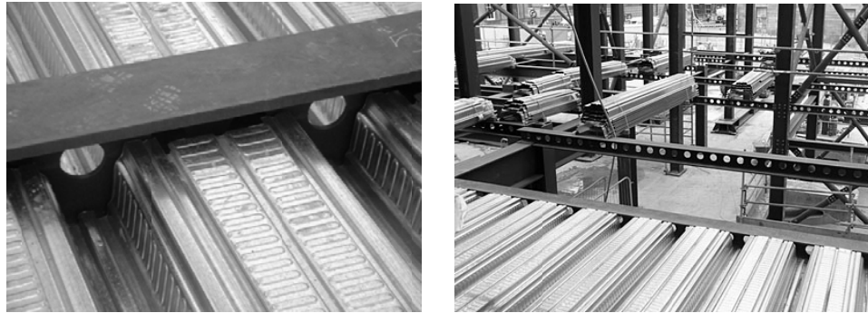
Figure 2. USFB construction adopted by Westok Ltd.
