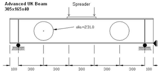
Figure 3. Test specimen configuration.
