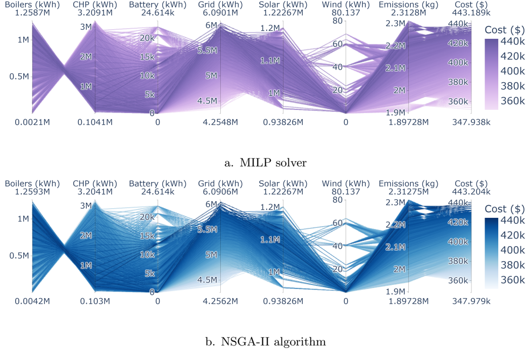
Figure 8: Comparison of parallel coordinates plot showing the variation in the optimum operation planning of energy components in a year to minimize the operating cost and CO_2 emissions for the 10,000 generated scenarios. These variations are almost identical when using the MILP solver versus the NSGA-II algorithm.
