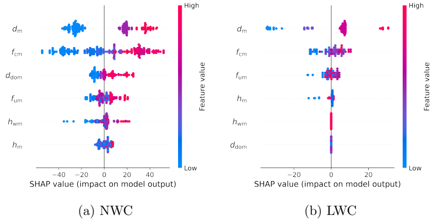
Figure 4: SHAP summary plots for LightGBM models
