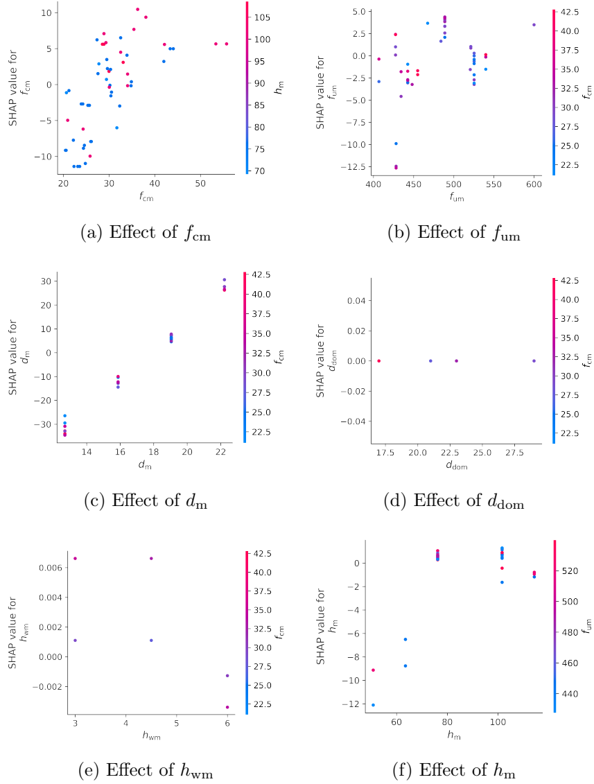
Figure 6: SHAP dependence plots for LightGBM LWC model
