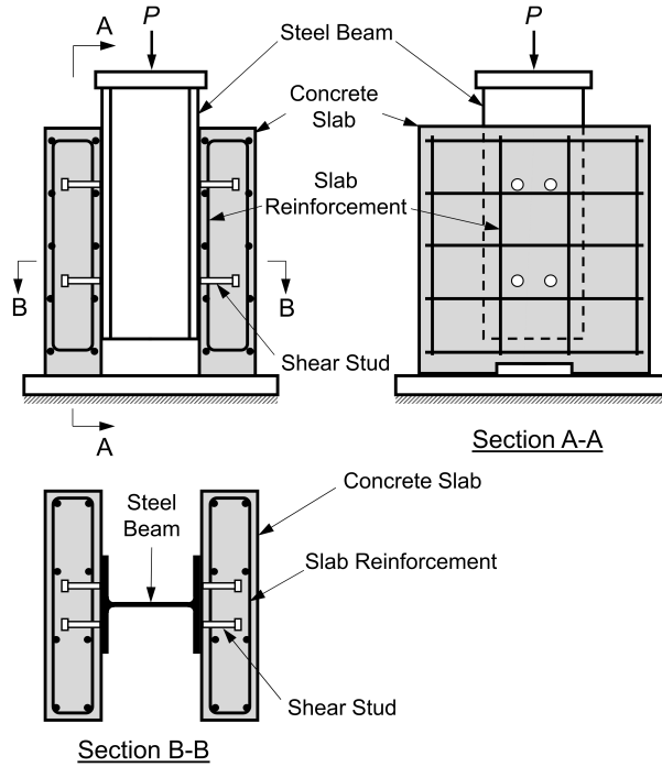
Figure 1: Standard push-out test according to Eurocode 4
