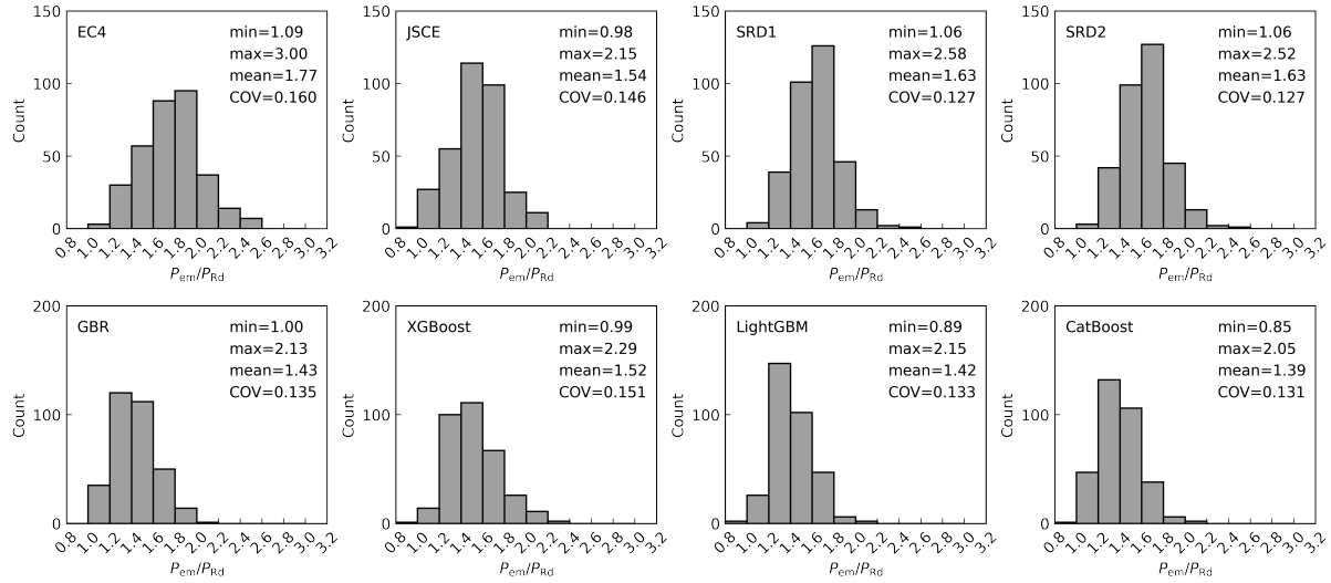
Figure 7: Test-to-prediction ratio distributions per the existing design models and ML models for the combined NWC and LWC database
