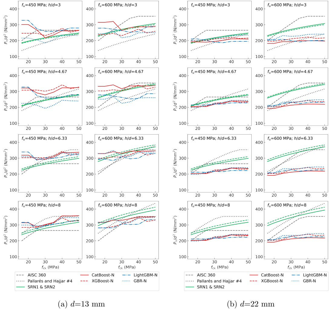
Figure 12: Comparisons of nominal shear resistances of studs in LWC predicted by the existing and proposed models
