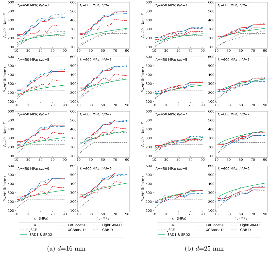
Figure 9: Comparisons of design shear resistances of studs in NWC predicted by the existing and proposed models
