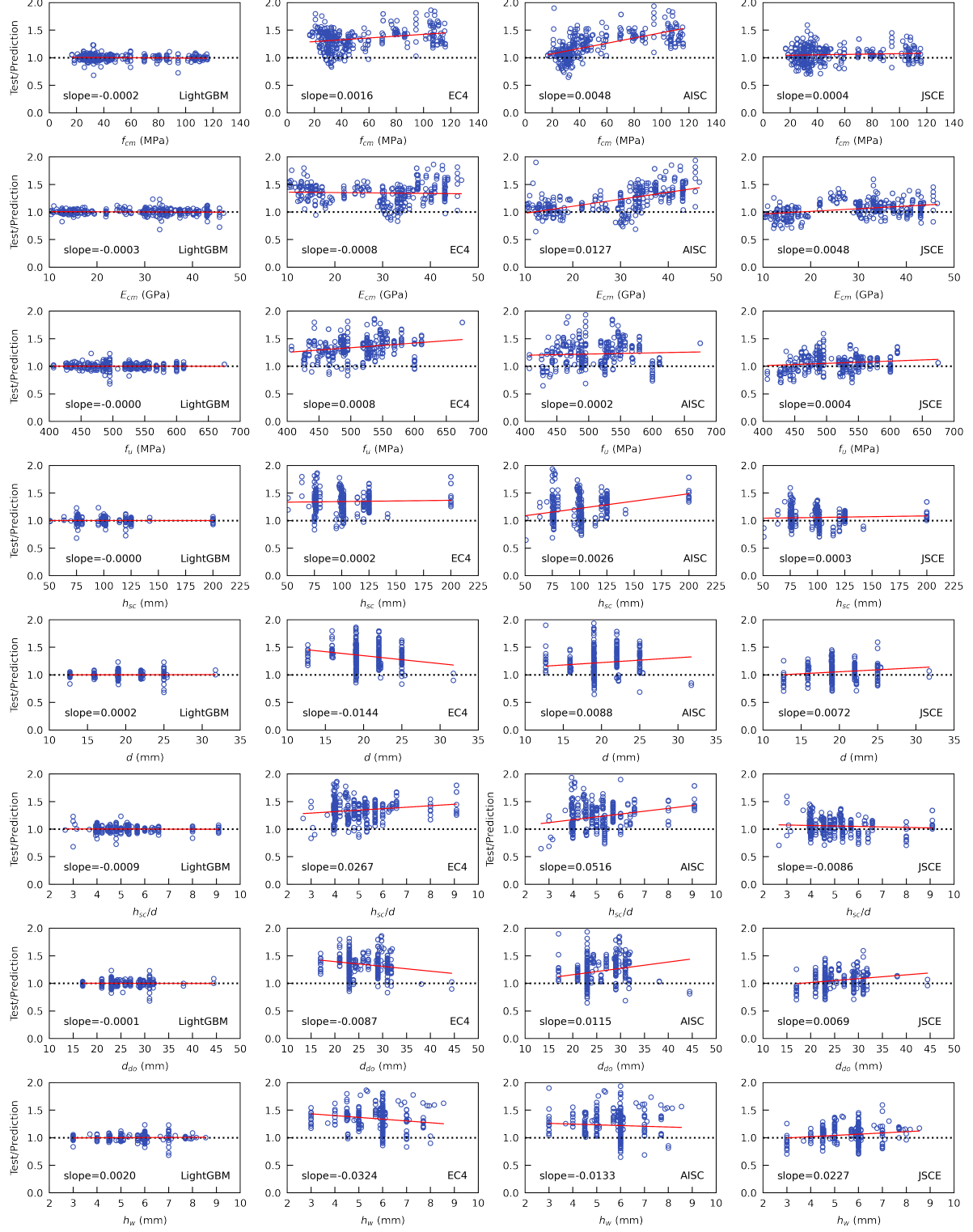
Figure 8: Test-to-prediction ratios versus variables for the LightGBM model and existing design models for the combined NWC and LWC database ( n = 322 tests)
