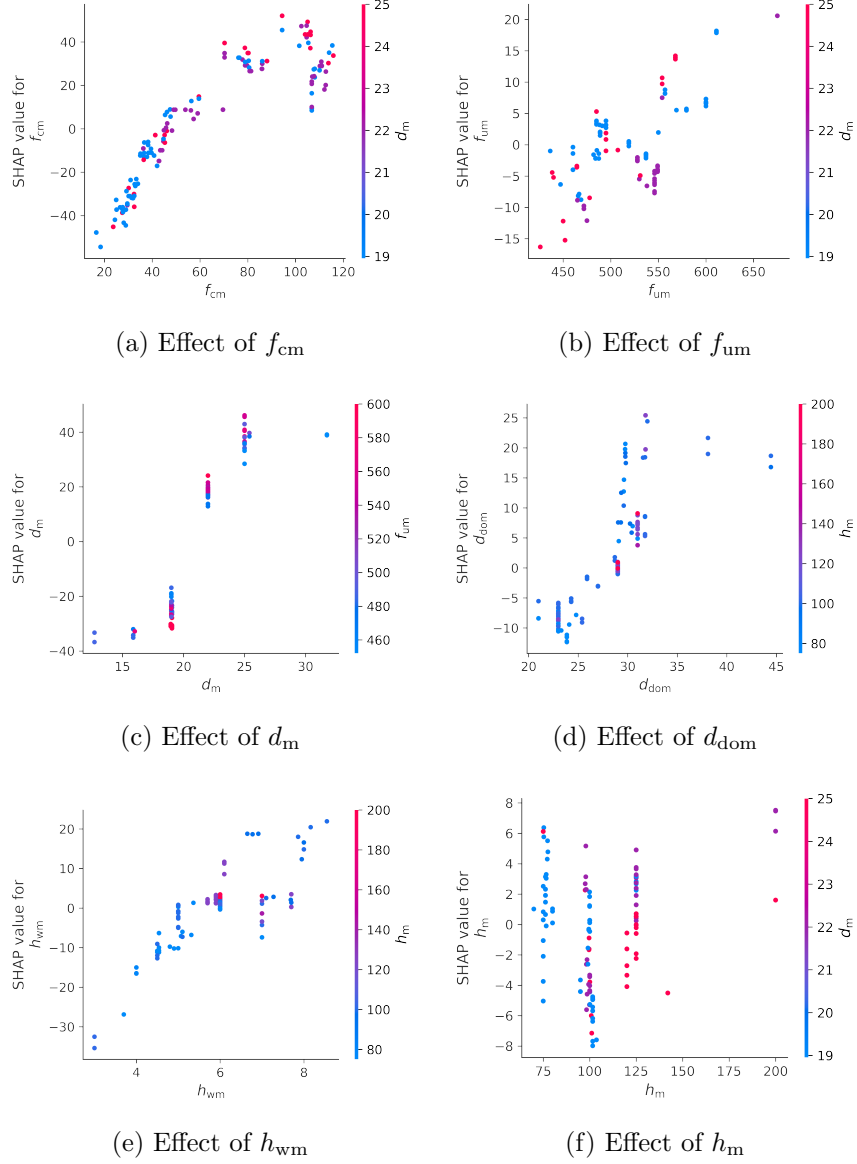
Figure 5: SHAP dependence plots for LightGBM NWC model
