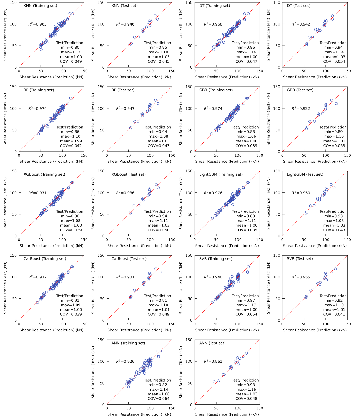
Figure 3: Performance of ML models for predicting the nominal (mean) shear resistance of studs in LWC slabs
