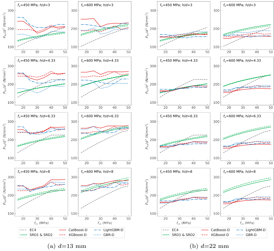
Fig. 12: Comparisons of design shear resistances of studs in LWC predicted by the existing and proposed models
