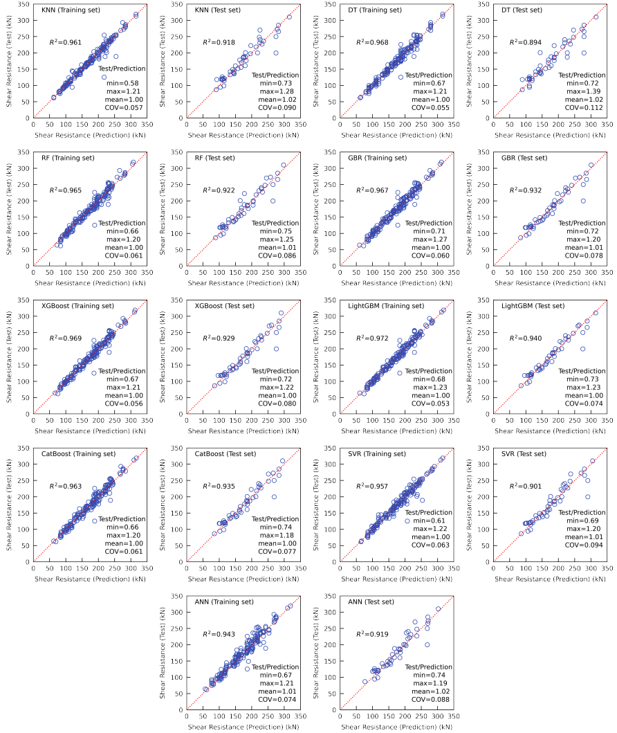
Fig. 3: Performance of ML models for predicting the nominal (mean) shear resistance of studs in NWC slabs
