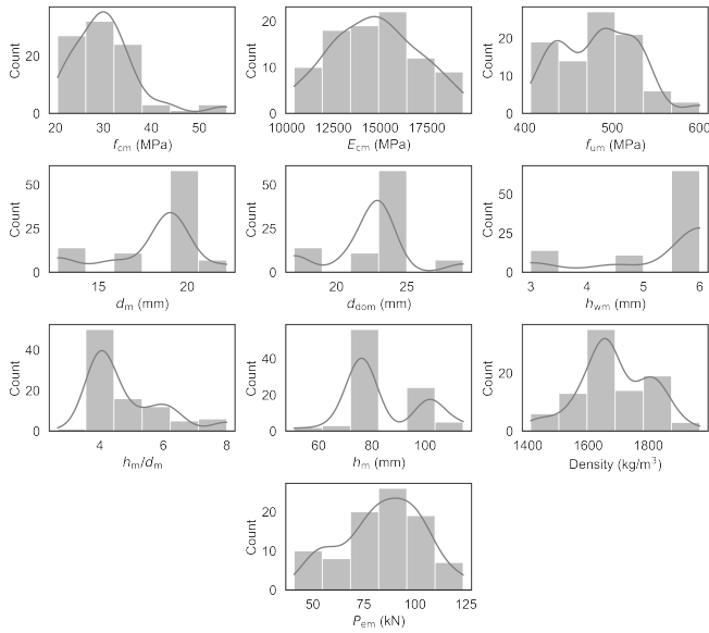
Fig. 2: Distributions of variables in the LWC database
