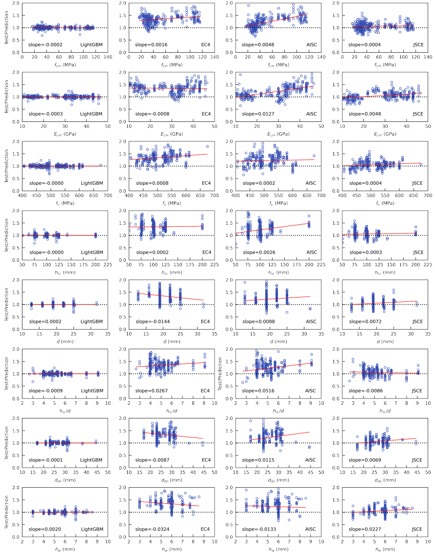
Fig. 9: Test-to-prediction ratios versus variables for the LightGBM model and existing design models for the combined NWC and LWC database
