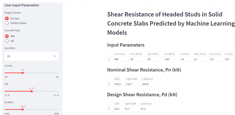
Fig. 14: GUI of the interactive web application
