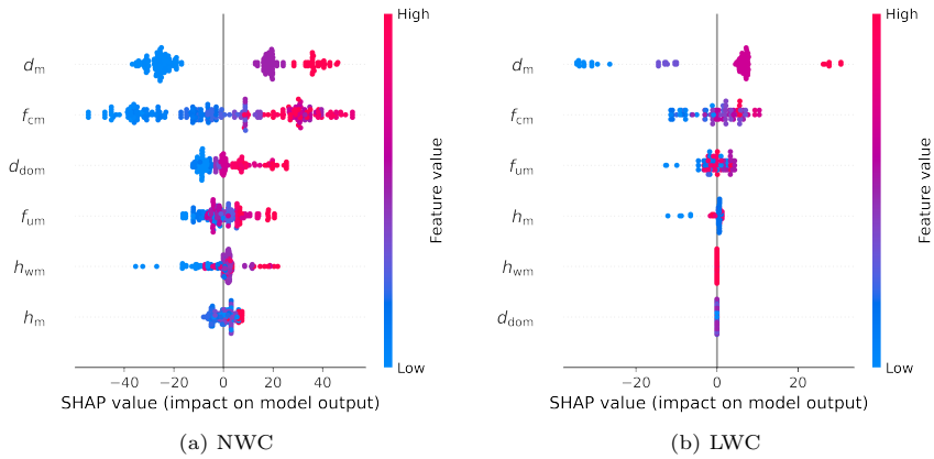
Fig. 5: SHAP summary plots for LightGBM models
