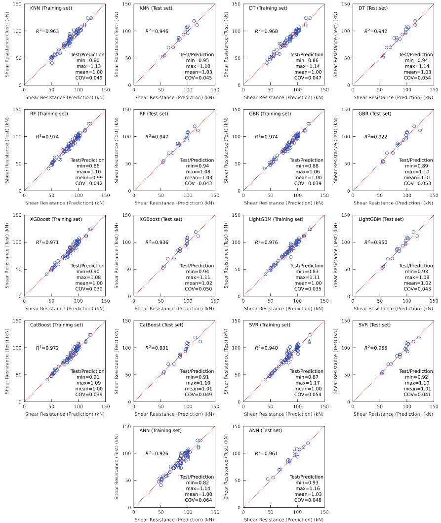
Fig. 4: Performance of ML models for predicting the nominal (mean) shear resistance of studs in LWC slabs
