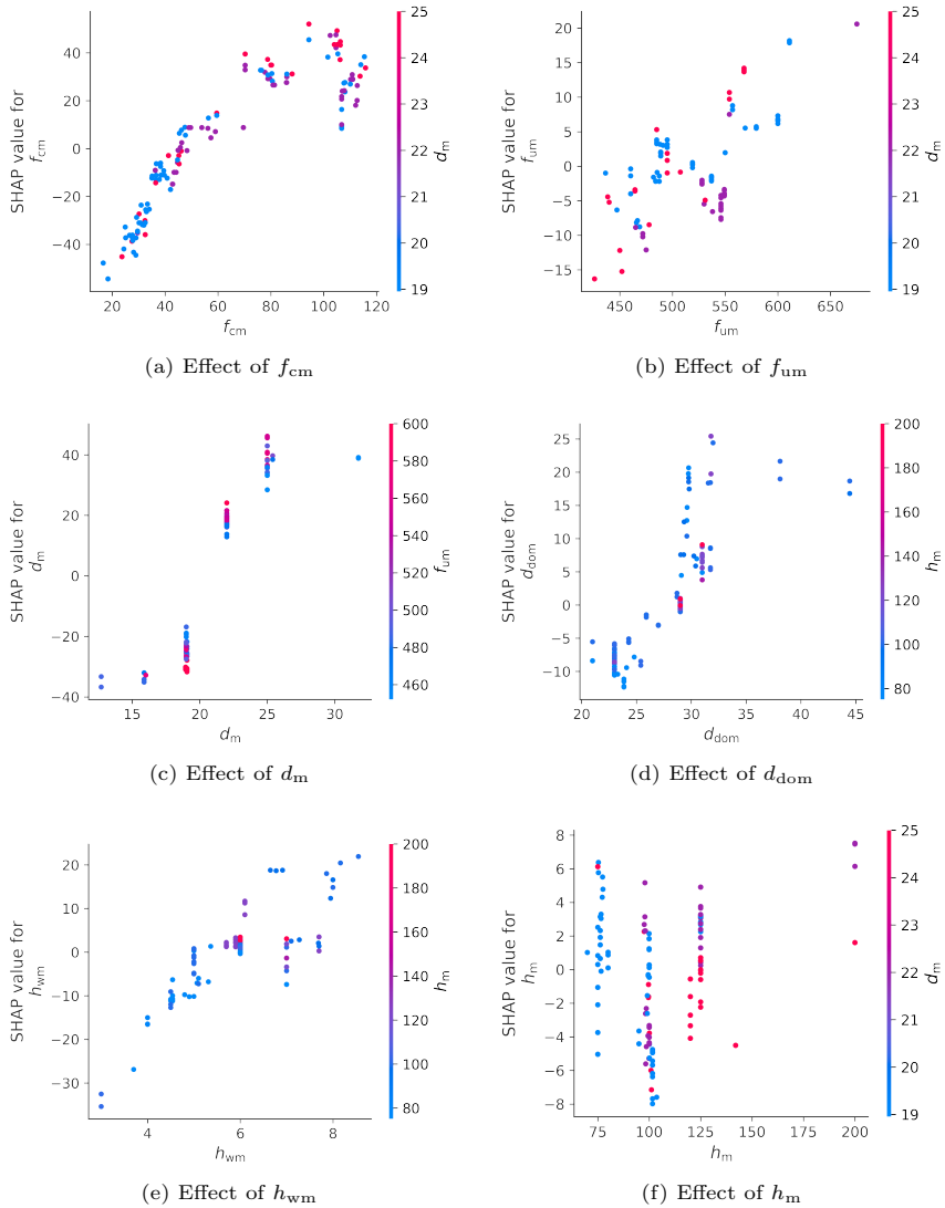
Fig. 6: SHAP dependence plots for LightGBM NWC model
