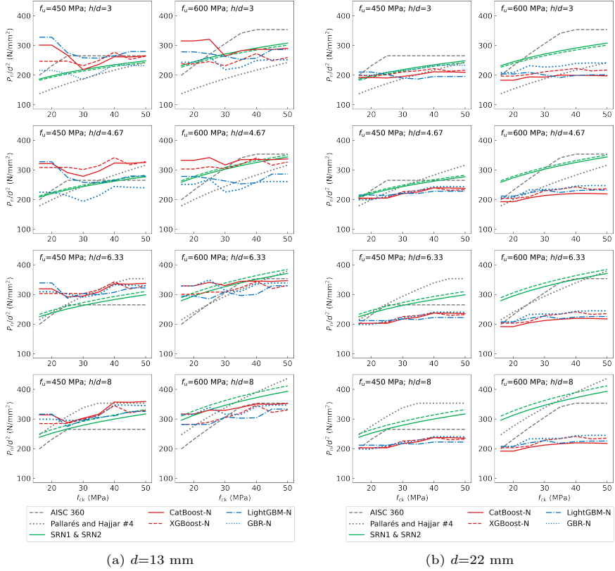
Fig. 13: Comparisons of nominal shear resistances of studs in LWC predicted by the existing and proposed models
