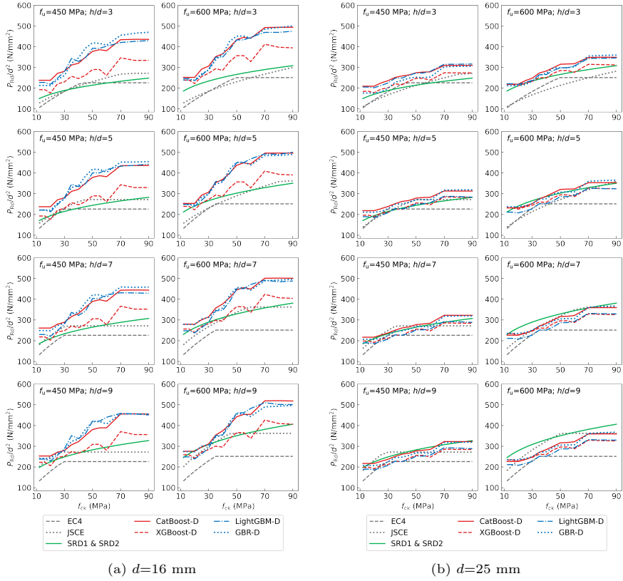
Fig. 10: Comparisons of design shear resistances of studs in NWC predicted by the existing and proposed models
