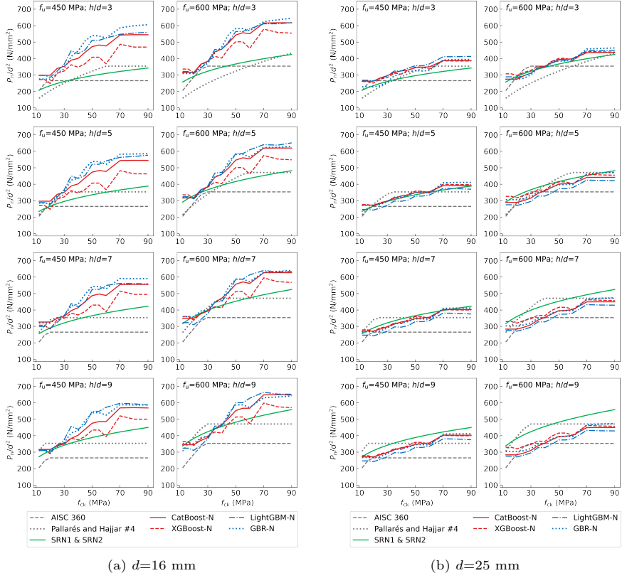
Fig. 11: Comparisons of nominal shear resistances of studs in NWC predicted by the existing and proposed models
