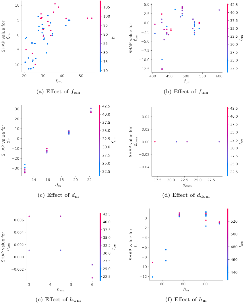
Fig. 7: SHAP dependence plots for LightGBM LWC model
