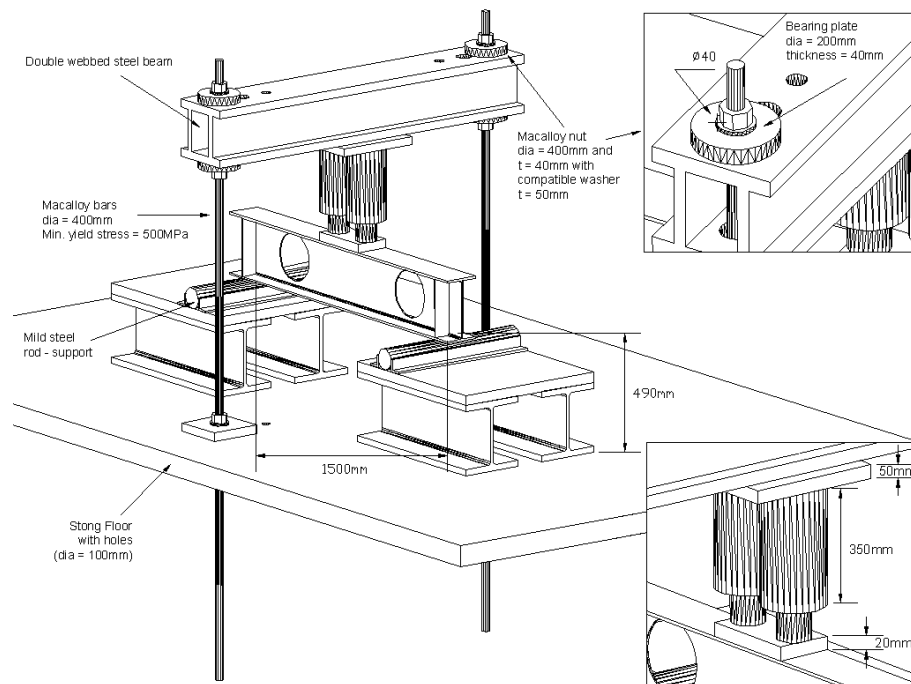
Figure 3. Experimental rig arrangement.
