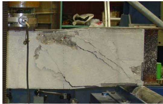
Figure 8. USFB No.2 at Failure point.
