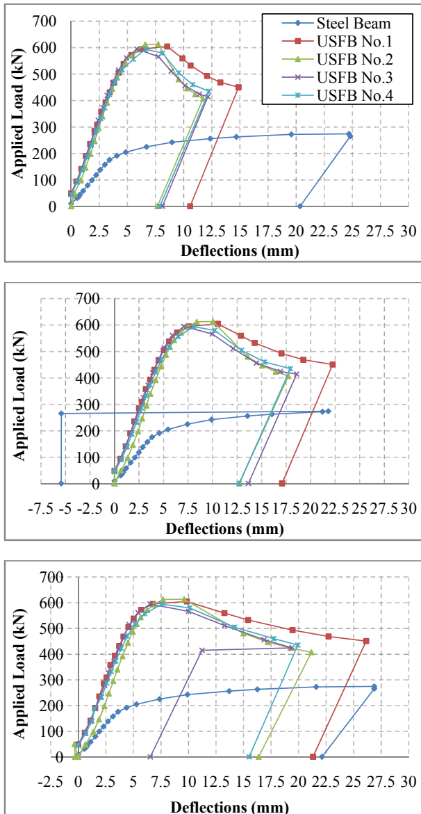
Figure 6. Load vs. Deflection curves for Bare Steel and USFBs for left, middle and right dial gauges.
