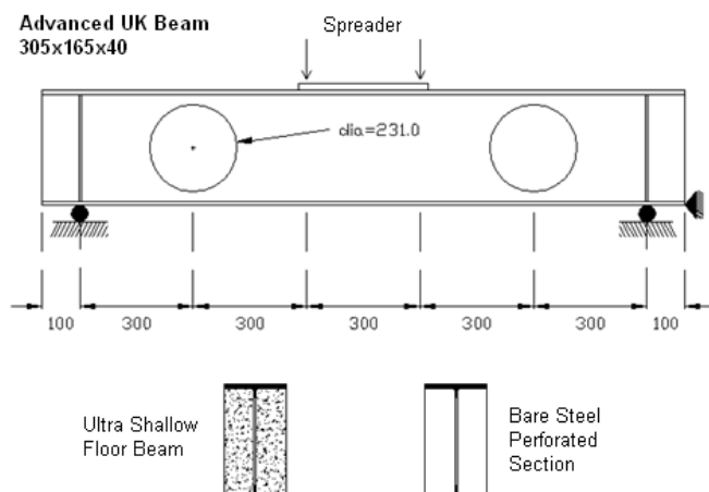
Figure 2. Specimen (all dimensions are in mm).
