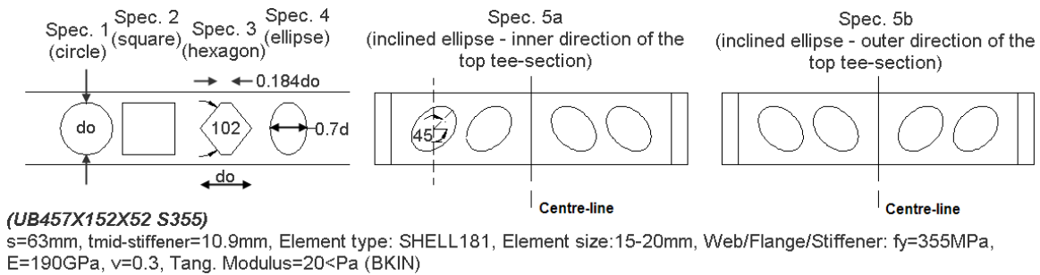
Fig. 8. Testing specimens and material properties
