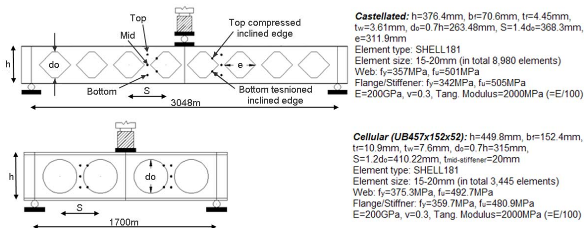
Fig. 1. Testing arrangements, section properties and material properties
