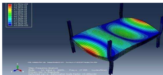
5 th natural frequency, f_{05}=27.96 Hz
