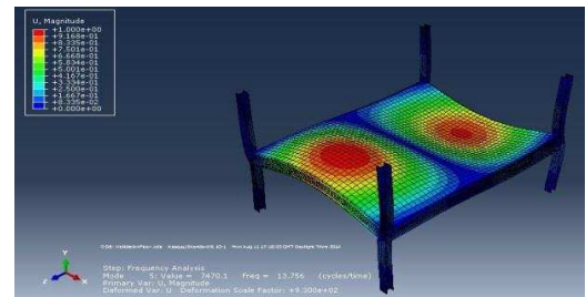
2 nd natural frequency, f_{02}=13.76 Hz
