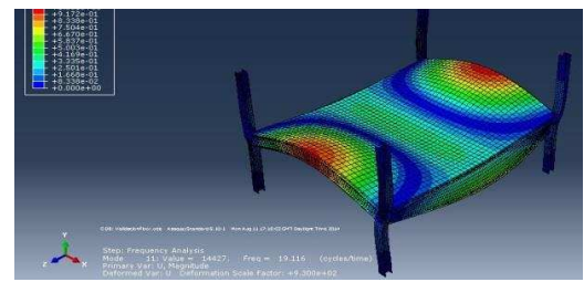
4 th natural frequency, f_{04}=19.12 Hz
