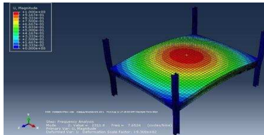
1 st natural frequency, f_{01}=7.65 Hz
