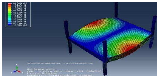
3 rd natural frequency, f_{03}=14.95 Hz
