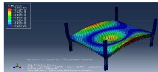
6 th natural frequency, f_{06}=28.74 Hz
