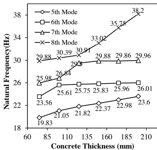
Fig. 9: Concrete Influence on Higher Modes
