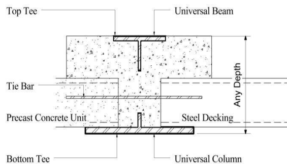
Fig. 2: Concept of Novel Composite Slab with USFB
