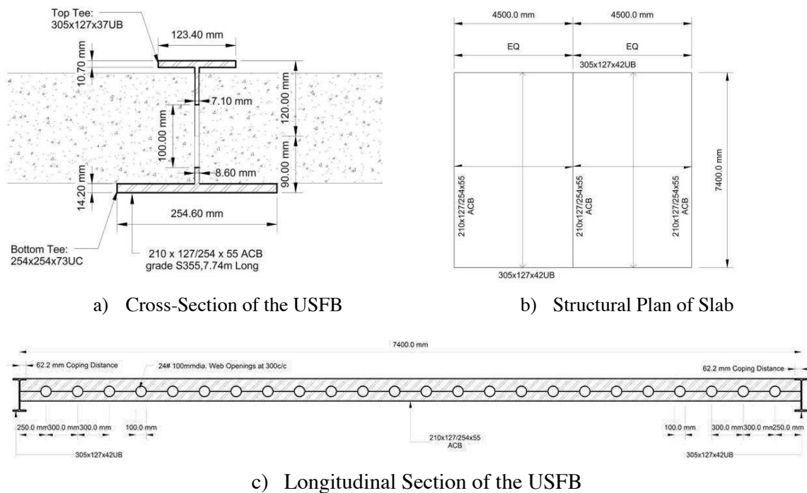
Fig. 3: Structural Model of the Composite Slab
