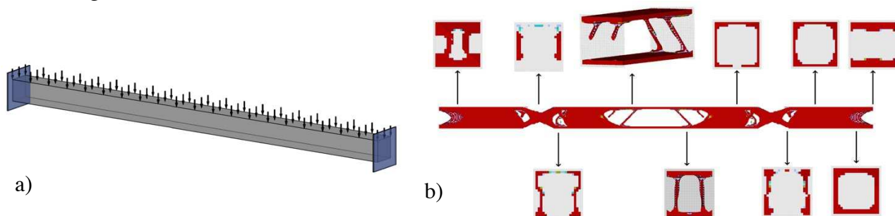
Figure 5. 3D optimisation input (a) and resulting topology with cross-sectional slices (b)
