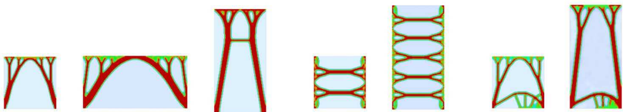
Figure 3. Topologies of cross-sections with various aspect ratios
