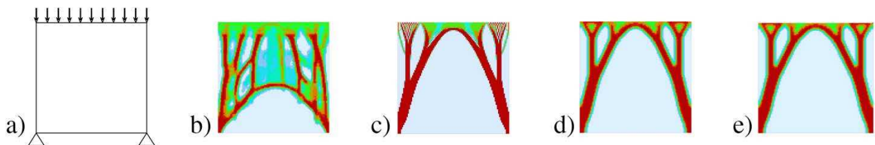
Figure 2. Development of the initial model topologies (a, b, c, d) and topology of S355 Steel (e)
