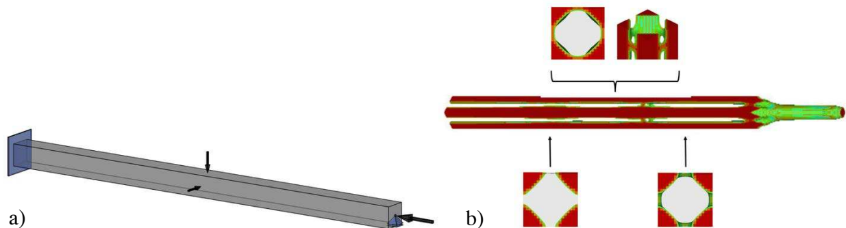
Figure 7. 3D optimisation input (a) and resulting topology with cross-sectional slices (b)
