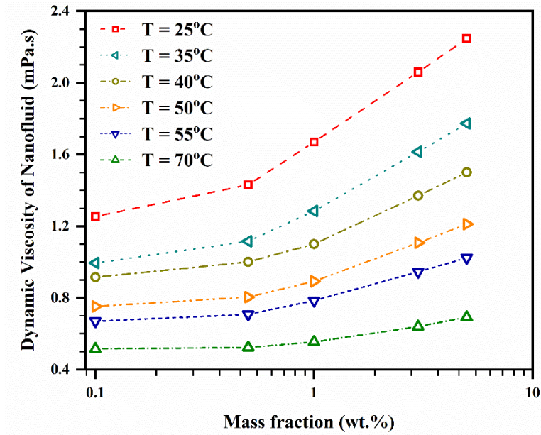
Figure 4. Value of nanofluid's dynamic viscosity at different nanoparticles mass fraction and temperature (Ghasemi & Karimipour, 2018; Sedeh et al., 2019; Dehghani et al., 2019; Abdollahi et al., 2018; Karimipour et al., 2018).
