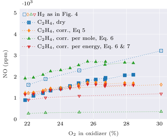
Figure 5: Comparison of measured and corrected NO x emissions for pulse detonation combustion with H 2 and C 2 H 4 . Stoichiometric mixtures are maintained while oxidizer mass flow rate is kept constant.
