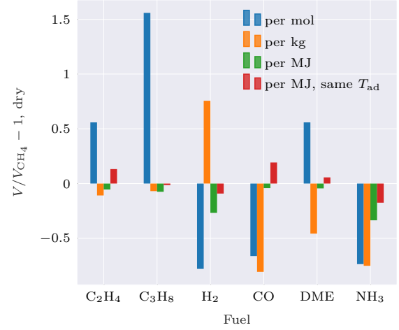
Figure 1: Reference volume for various fuels compared to \text{CH}_4 . All fuels combusted in air, except for \text{NH}_3 using enriched air with 30% _{\text{vol}}\text{O}_2 to reach the same T_{\text{ad}} .
