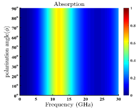
Fig. 3. Polarization insensitivity analysis for the designed absorber
