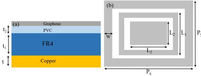
Fig. 1. Unit cell of the absorber (a) Layered view, (b) Top view
