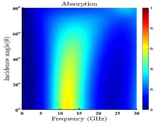
Fig. 5. TM wave incidence angle analysis for the designed absorber
