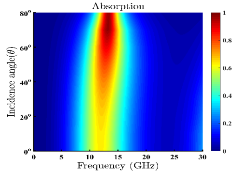
Fig. 4. TE wave incidence angle analysis for the designed absorber
