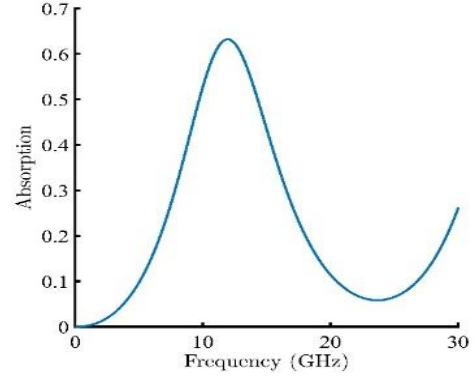
Fig. 2. Absorption for the designed absorber
