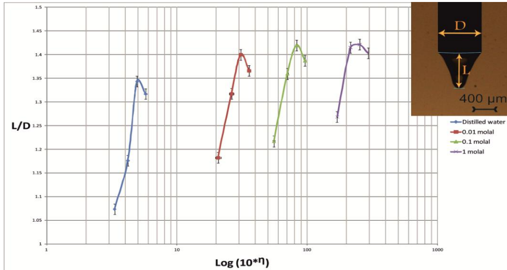
Figure 6 Fluctuation of non-dimensionalized cone length (L) versus non-dimensional flow rate for various conductivities. D is the nozzle outer diameter.
