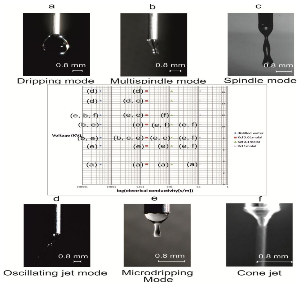
Figure 2 Electro spraying modes for different KCl solution in different applied voltage
