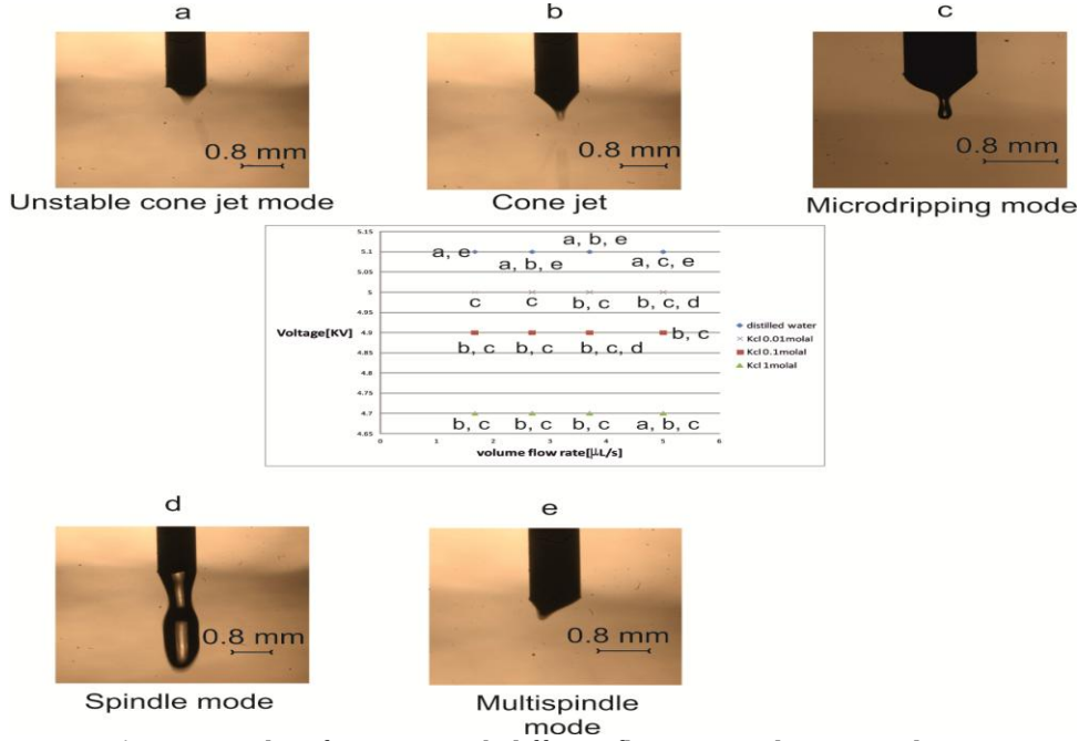
Figure 3 Modes of spraying with different flow rates and various voltages
