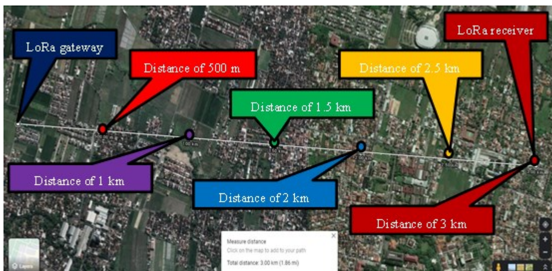
Figure 5. Distance measurement of LoRa gateway and receiver
