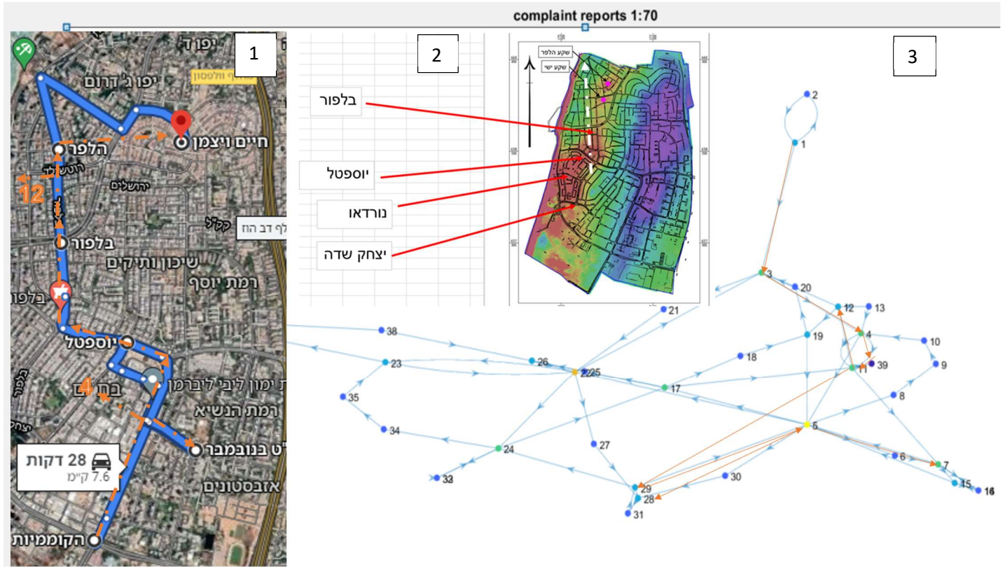
Fig. 6. Partial virtual faults network (1) vs. physical conduits (2) and topography (3)
