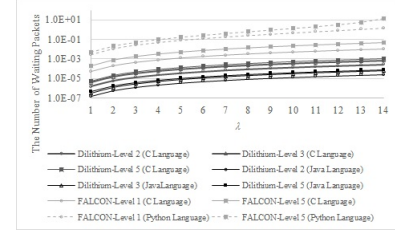
Fig. 3. The waiting packet number of each PQC method for signature.
