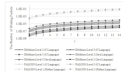
Fig. 5. The waiting packet number of each PQC method for verification.
