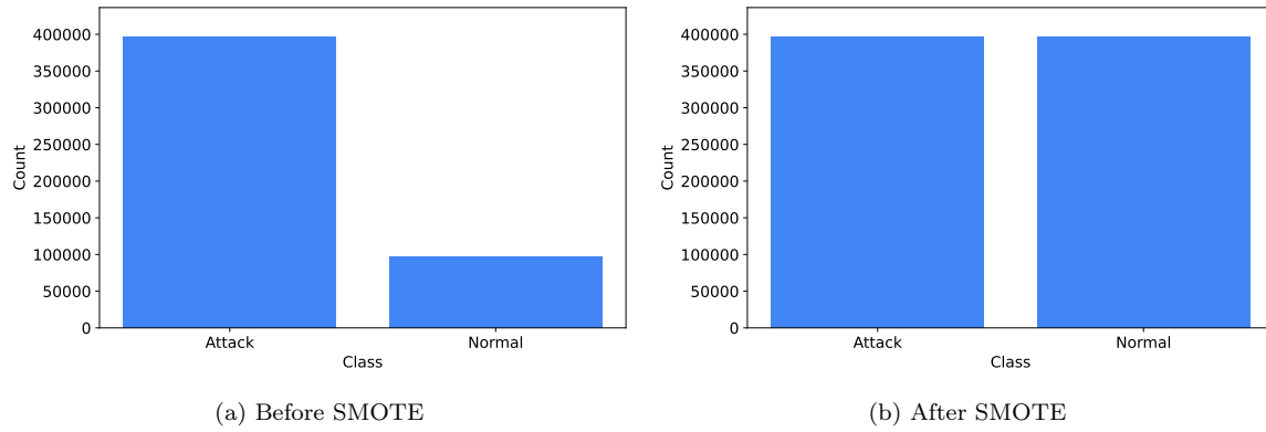
Figure 5: Before and After the distribution of attacks in KDDCUP'99 for binary classification.
