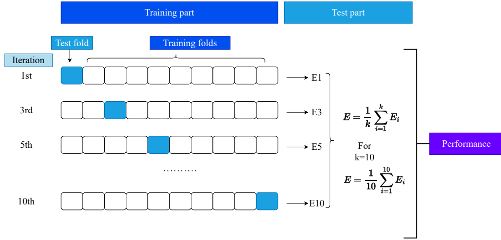
Figure 8: K-fold cross-validation.
